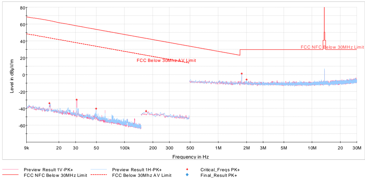
Plot 7-9. Radiated Spurious Emissions 9kHz – 30MHz (Reader A 848kbps, with AC/DC Adapter and Magnetic Charger)
