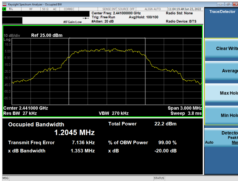
Plot 7-5. Conducted 20dB BW and 99% OBW Plot (Bluetooth, 8DPSK, ePA – Ch. 39)
