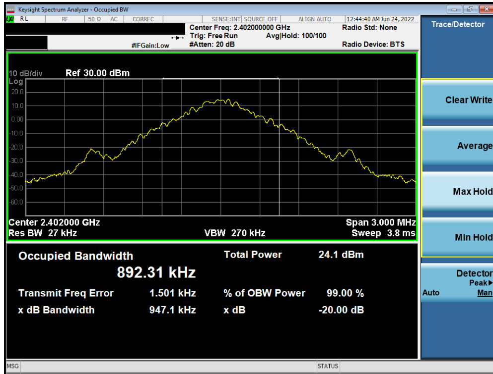
Plot 7-1. Conducted 20dB BW and 99% OBW Plot (Bluetooth, GFSK, ePA – Ch. 0)
