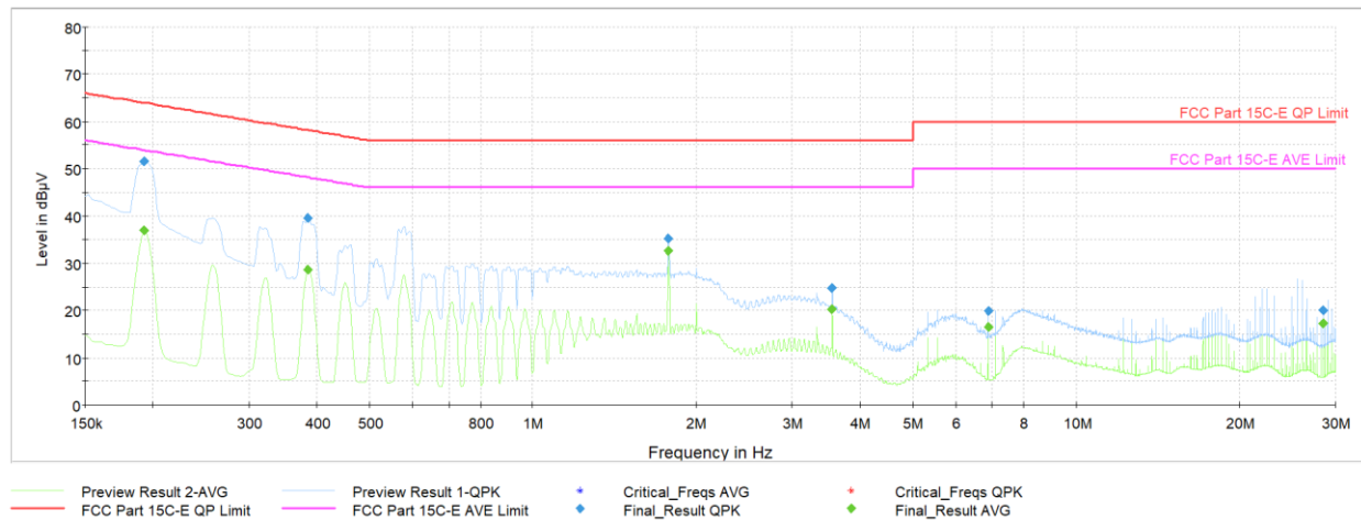
Plot 7-43. AC Line-Conducted Test Plot (L1, GFSK ePA – Ch.0, with AC/DC Adapter + Laptop Charger)
