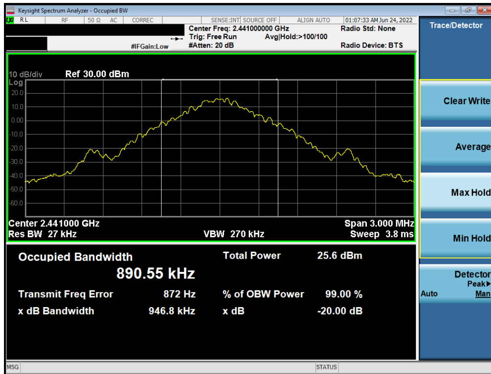
Plot 7-2. Conducted 20dB BW and 99% OBW Plot (Bluetooth, GFSK, ePA – Ch. 39)
