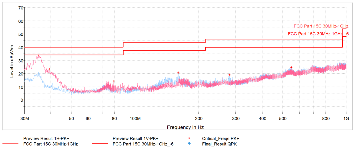
Plot 7-41. Radiated Spurious Plot Below 1GHz (GFSK ePA – Ch.39, Pol. H & V, with AC/DC Adapter + Magnetic Charger)
