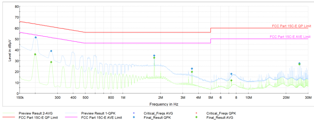
Plot 7-44. AC Line-Conducted Test Plot (N, GFSK ePA – Ch.39, with AC/DC Adapter + Laptop Charger)
