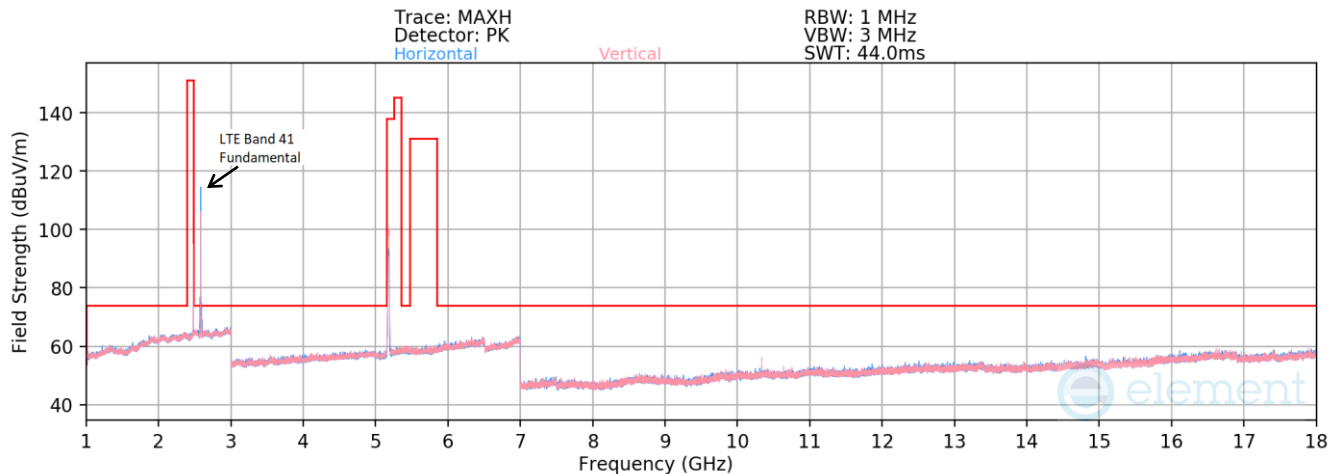
Plot 7-34. Radiated Spurious Emissions 1 - 18GHz – Simultaneous Transmission
