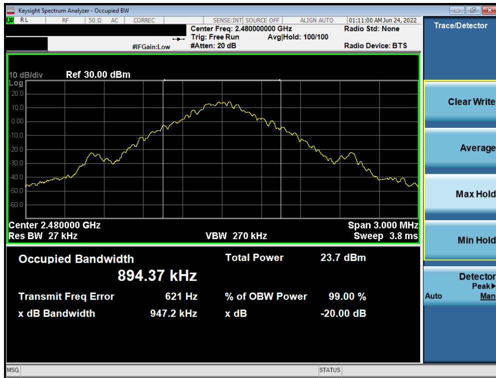
Plot 7-3. Conducted 20dB BW and 99% OBW Plot (Bluetooth, GFSK, ePA – Ch. 78)
