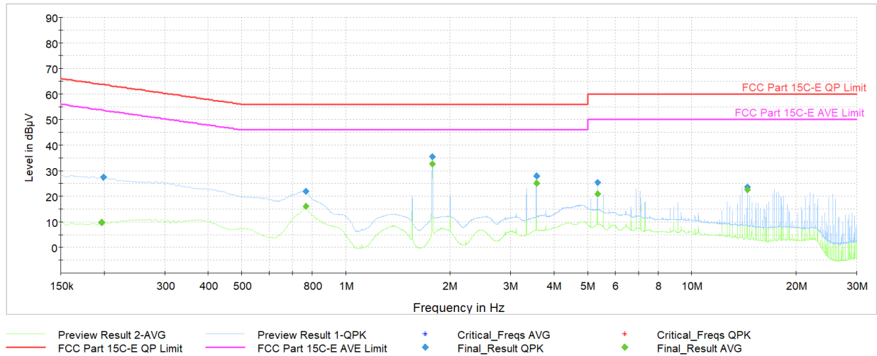
Plot 7-80. AC Line Conducted Plot 11b Ch.6 (N, with AC/DC Adapter and Magnetic Charger)
