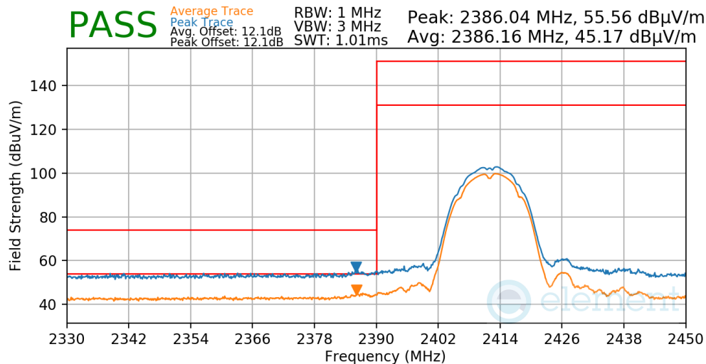
Plot 7-61. Radiated Restricted Lower Band Edge Measurement
