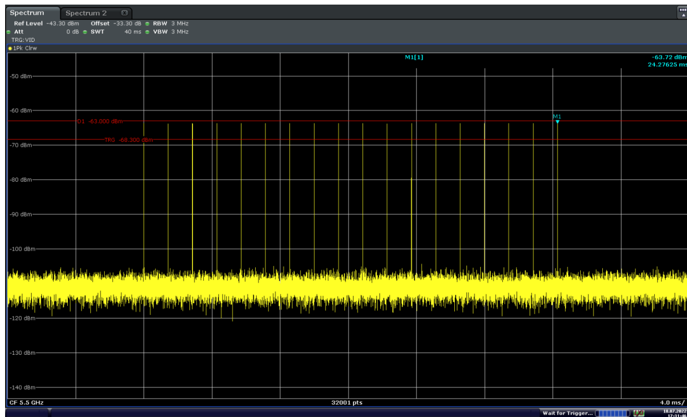
Figure 7-3. 5500MHz – Radar Pulse Type 0 (20MHz)
