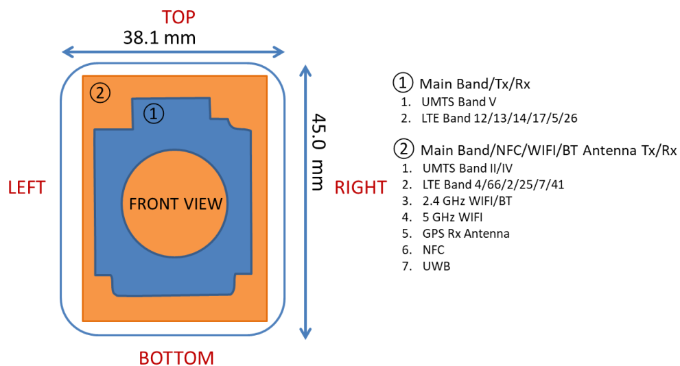
Figure E-1 DUT Antenna Locations
