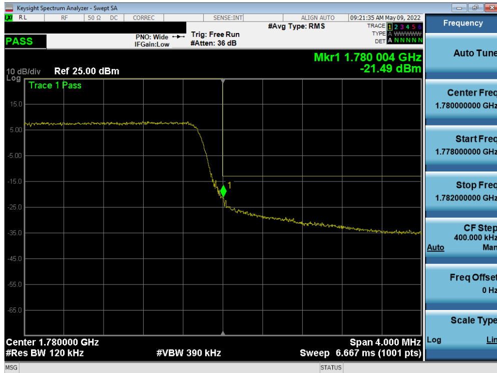
Plot 7-66. Upper Band Edge Plot (LTE Band 66 - 5MHz QPSK – Full RB)
