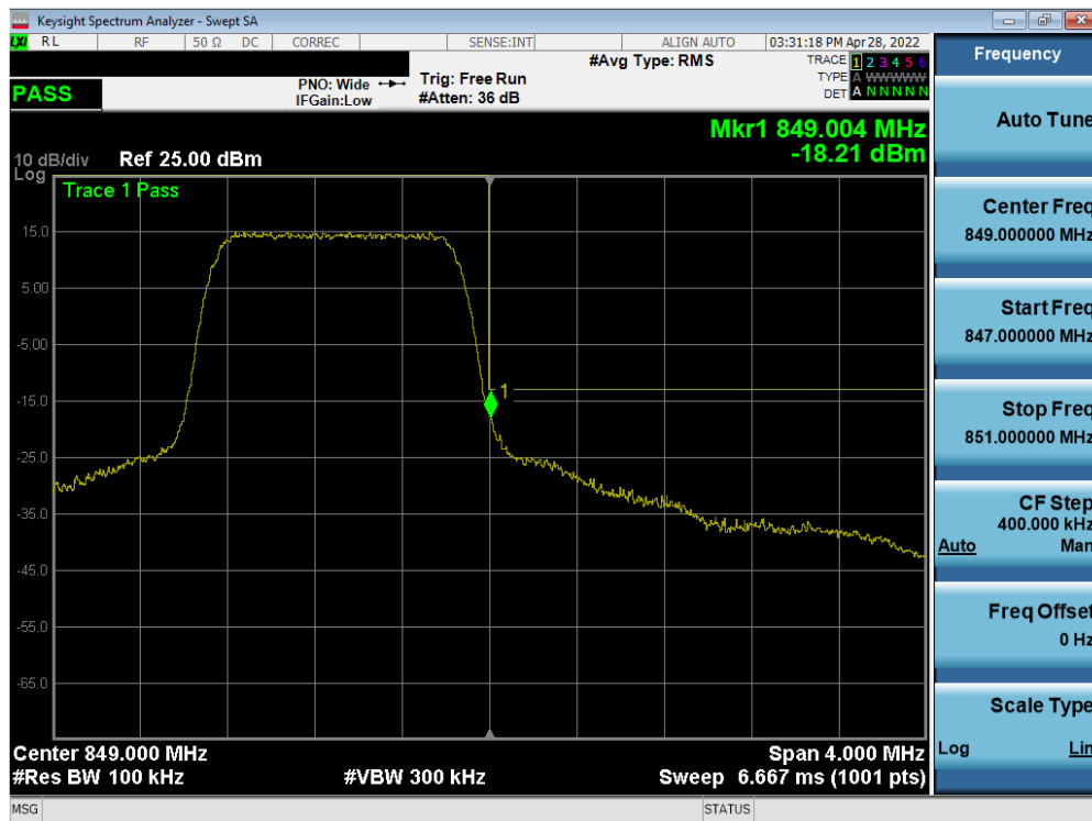
Plot 7-37. Upper BE Plot (LTE Band 26 – 1.4MHz QPSK – Full RB Configuration)
