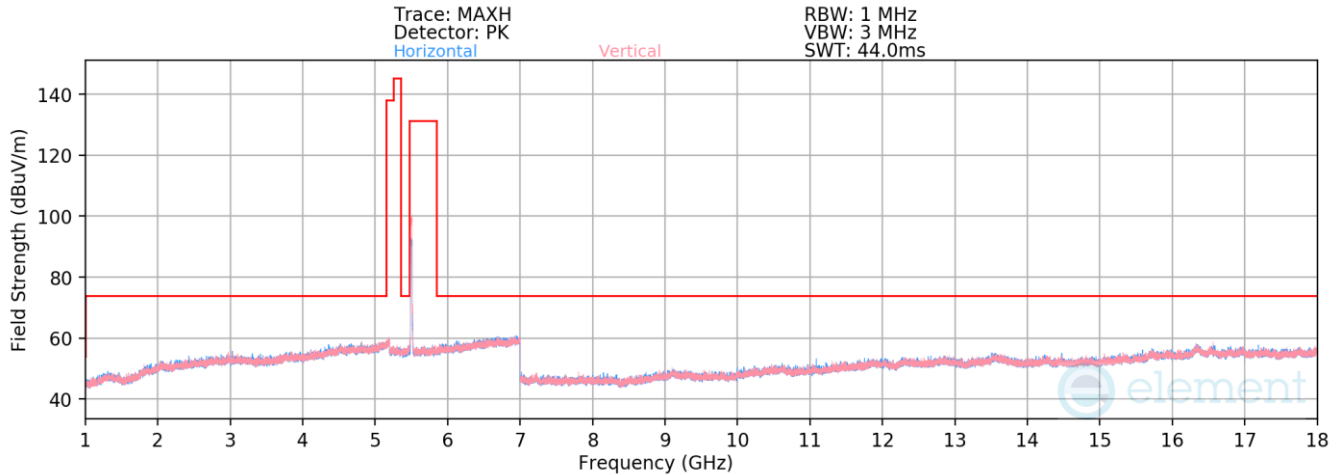
Plot 7-33. Radiated Spurious Emissions above 1GHz (802.11n – Ch. 100)
