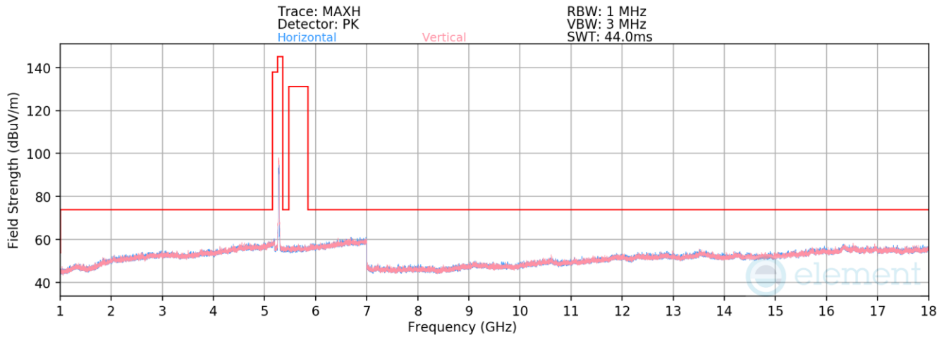
Plot 7-31. Radiated Spurious Emissions above 1GHz (802.11n – Ch. 56)
