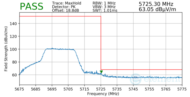
Plot 7-51. FCM (Pk, Ch.140, 802.11n, MCS7)
