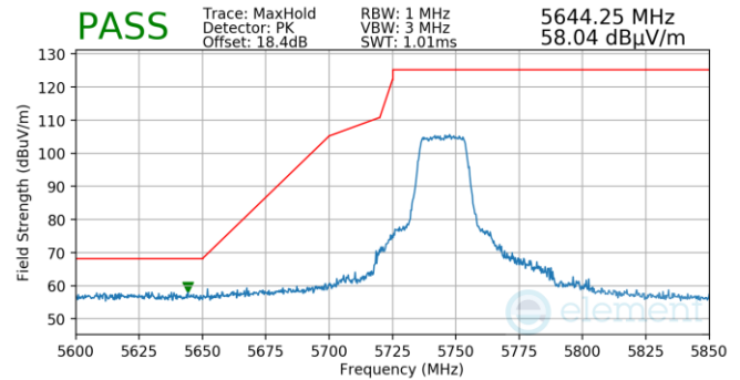
Plot 7-52. FCM (Pk, Ch.149, 802.11n, MCS0)
