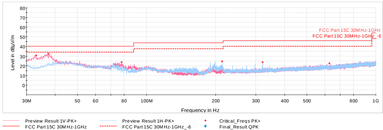
Plot 7-56. Radiated Spurious Emissions below 1GHz 802.11n, Ch.36 with AC/DC Adapter & magnetic charger
