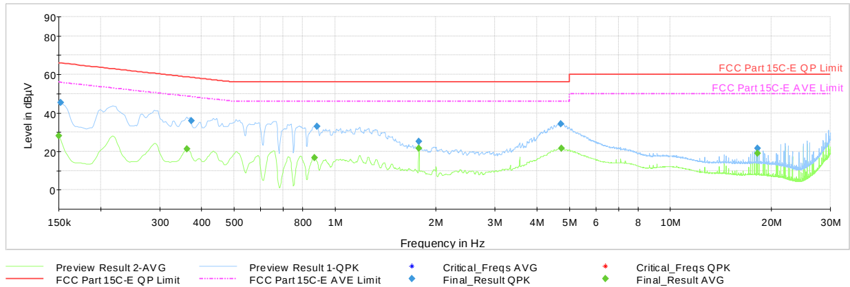
Plot 7-59. AC Line Conducted Plot with 802.11n– Ch.36 (N), with Laptop & magnetic charger
