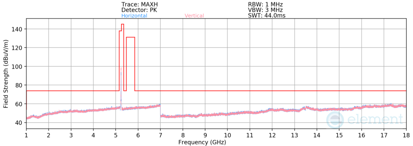
Plot 7-29. Radiated Spurious Emissions above 1GHz (802.11n – Ch. 48)
