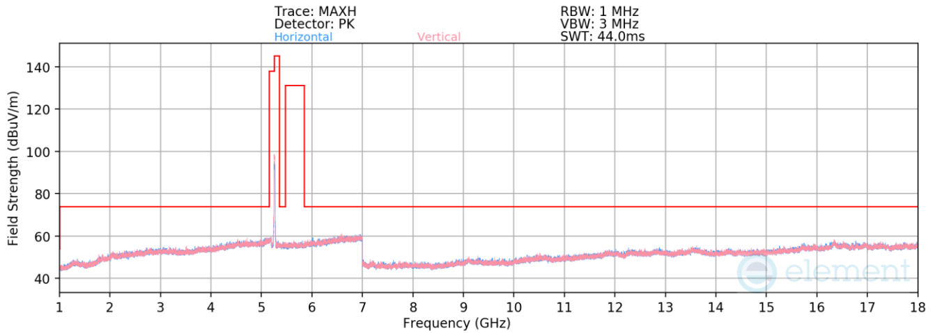
Plot 7-30. Radiated Spurious Emissions above 1GHz (802.11n – Ch. 52)
