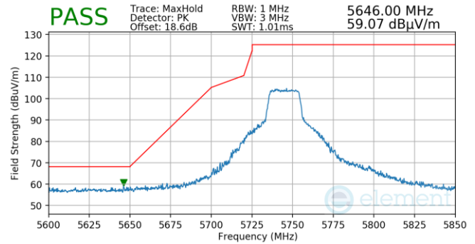
Plot 7-53. FCM (Pk, Ch.149, 802.11n, MCS7)
