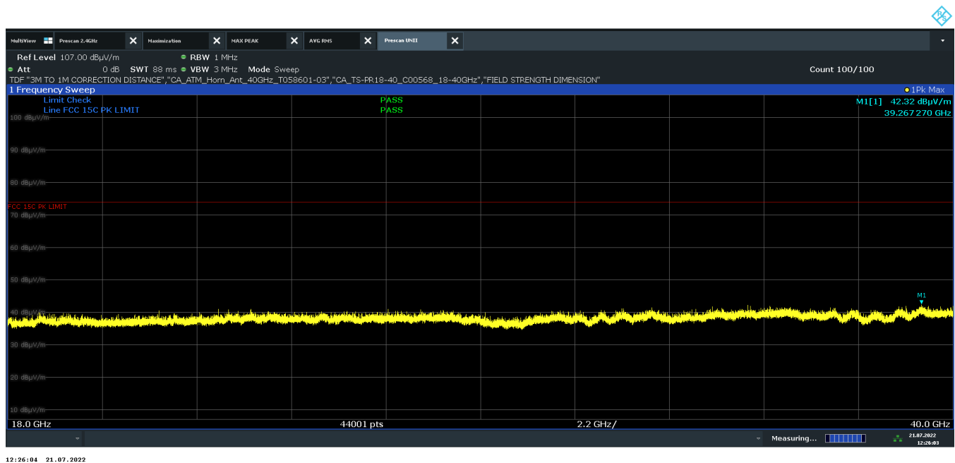
Plot 7-27. Radiated Spurious Emissions 18GHz-40GHz V Polarity (802.11n – Ch. 36)
