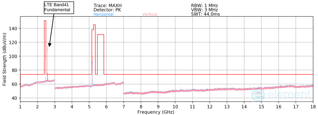
Plot 7-39. Radiated Spurious Emissions -Simultaneous Transmission 1GHz – 18GHz
