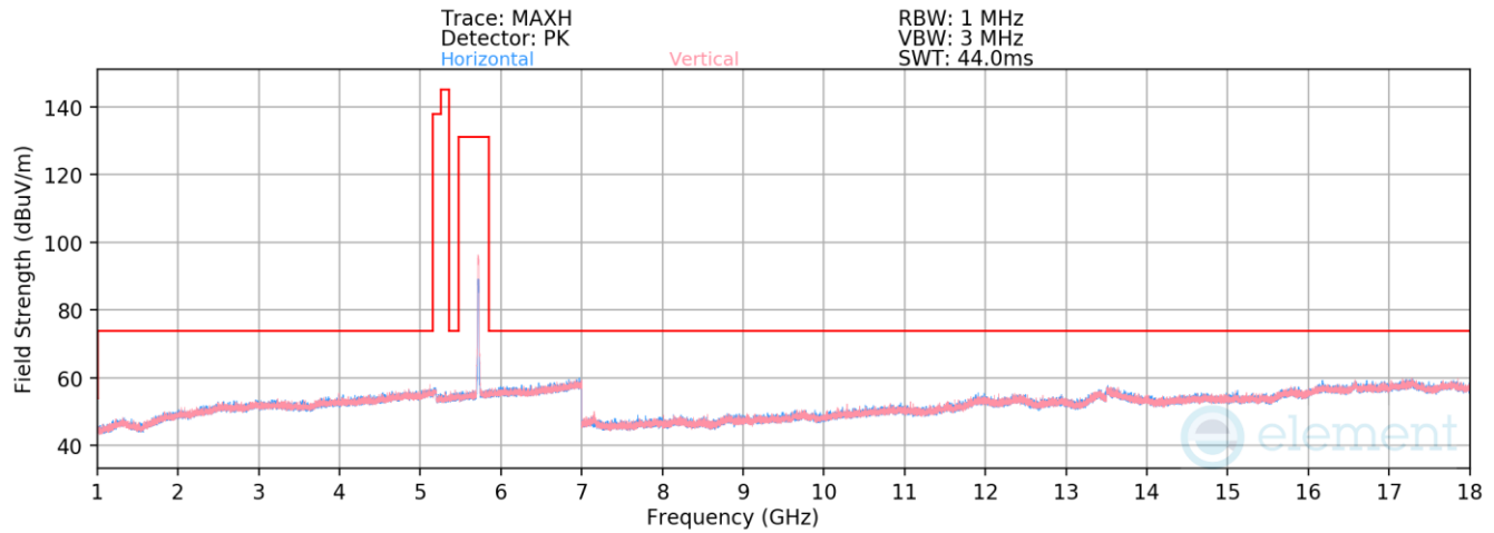
Plot 7-35. Radiated Spurious Emissions above 1GHz (802.11n – Ch. 144)
