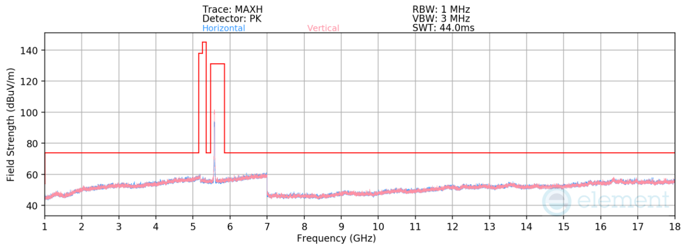
Plot 7-34. Radiated Spurious Emissions above 1GHz (802.11n – Ch. 116)
