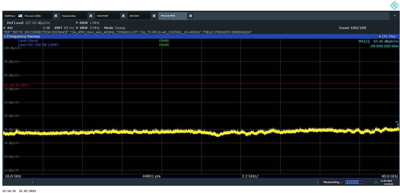
Plot 7-26. Radiated Spurious Emissions 18GHz-40GHz H Polarity (802.11n – Ch. 36)
