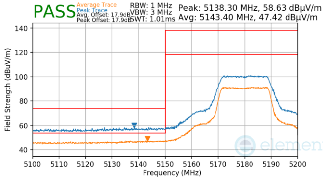
Plot 7-42. FCM (Pk & Avg, Ch.36, 802.11n, MCS0)
