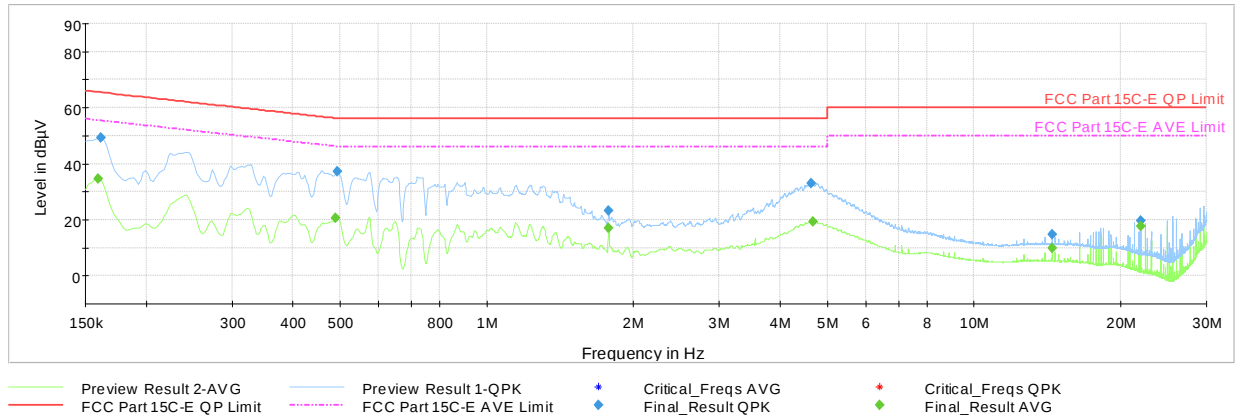
Plot 7-58. AC Line Conducted Plot with 802.11n- Ch.36 (L1), with Laptop & magnetic charger
