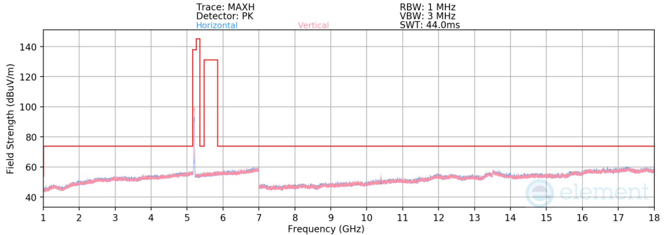
Plot 7-28. Radiated Spurious Emissions above 1GHz (802.11n – Ch. 40)
