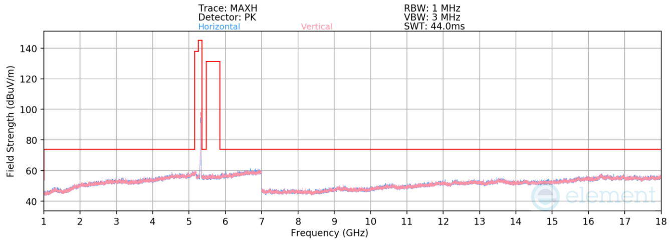
Plot 7-32. Radiated Spurious Emissions above 1GHz (802.11n – Ch. 64)
