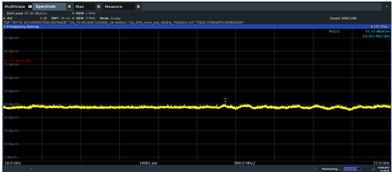
Plot 7-33. Radiated Spurious Emissions Above 18GHz (1Mbps ePA – Ch. 39, Pol. V)
