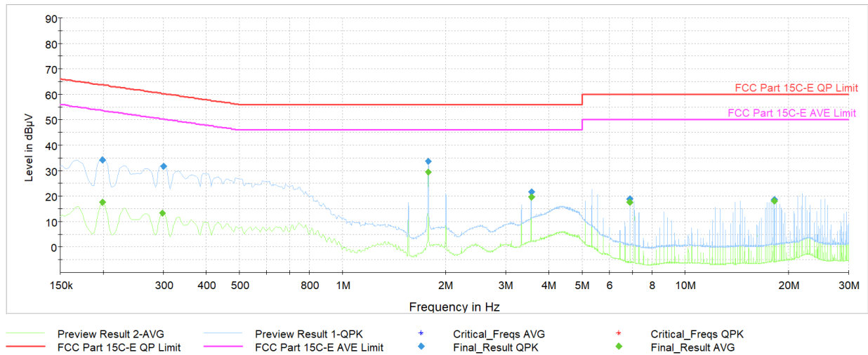
Plot 7-40. AC Line Conducted Plot with Bluetooth LE (N, 1Mbps ePA – Ch.19, with AC/DC Adapter + Magnetic Charger)
