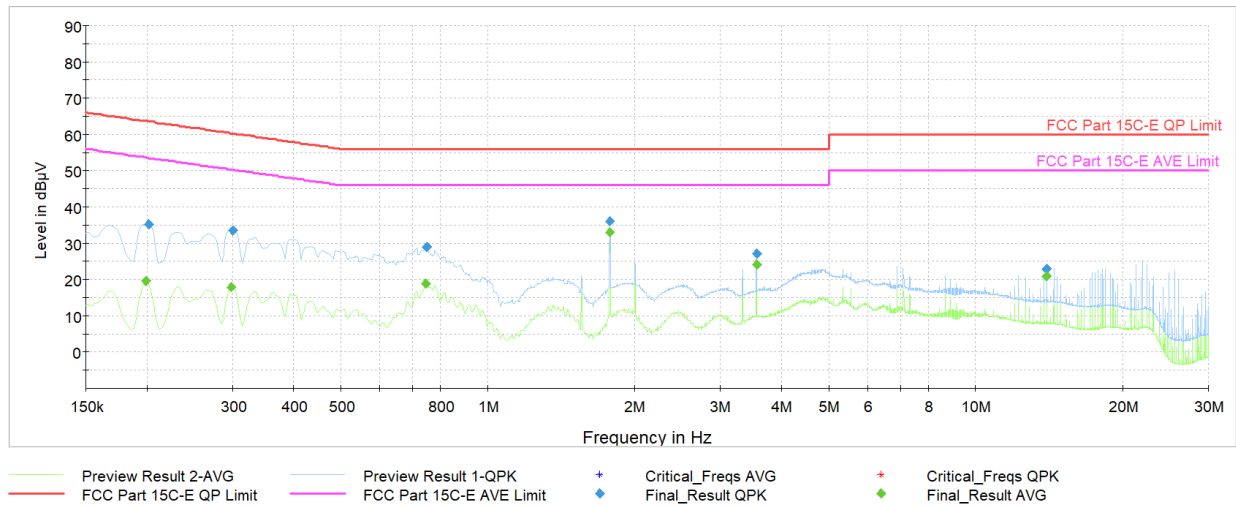
Plot 7-39. AC Line Conducted Plot with Bluetooth LE (L1, 1Mbps ePA – Ch.19 with AC/DC Adapter + Magnetic Charger)
