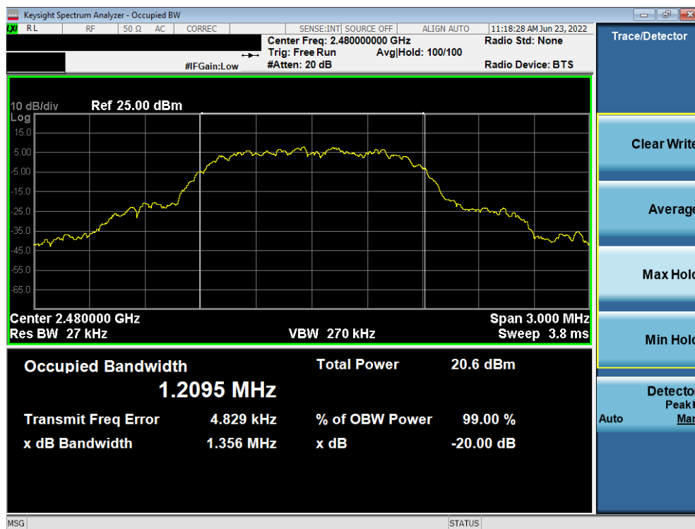
Plot 7-6. Conducted 20dB BW and 99% OBW Plot (Bluetooth, 8DPSK, ePA – Ch. 78)
