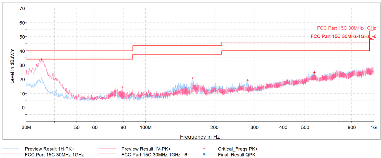
Plot 7-41. Radiated Spurious Plot Below 1GHz (GFSK ePA – Ch.39, Pol. H & V, with AC/DC Adapter + Magnetic Charger)
