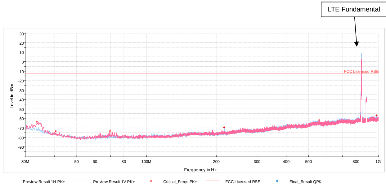
Plot 7-46. Antenna BCM Radiated Spurious Plot below 1GHz (LTE Band 26)
