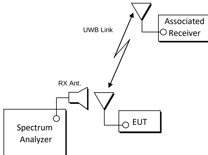
Figure 7-4. Test Setup
