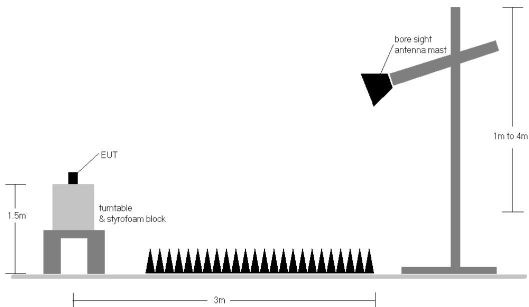
Figure 7-1. Test Setup
