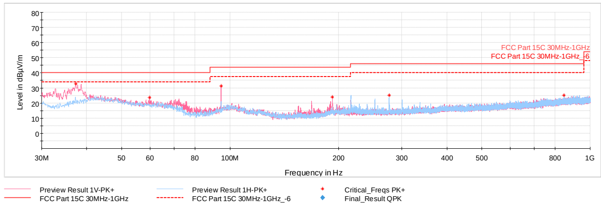
Plot 7-41. Radiated Spurious Emissions Below 1GHz (GFSK ePA, Pol. H & V, with AC/DC Adapter + Magnetic Charger)
