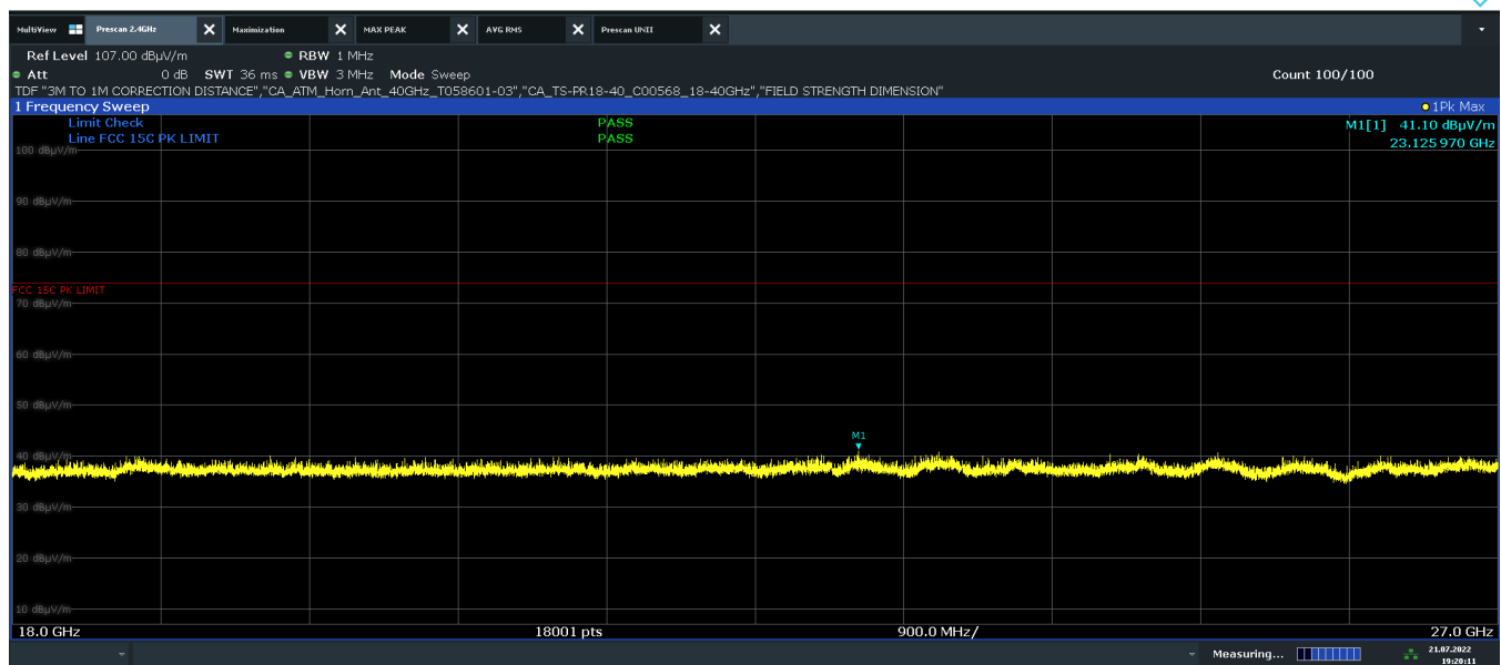
Plot 7-33. Radiated Spurious Emissions above 18GHz (BT GFSK ePA – Ch.0, Ant. Pol V)
