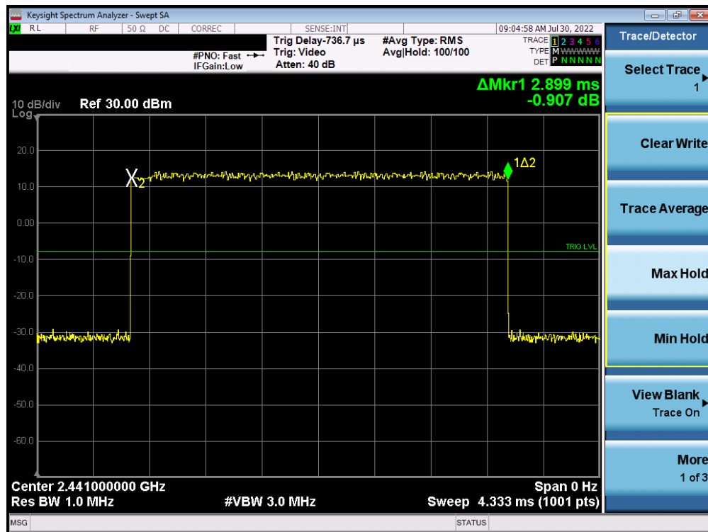
Plot 7-18. Time of Occupancy Plot(Bluetooth, 8DPSK, ePA)
