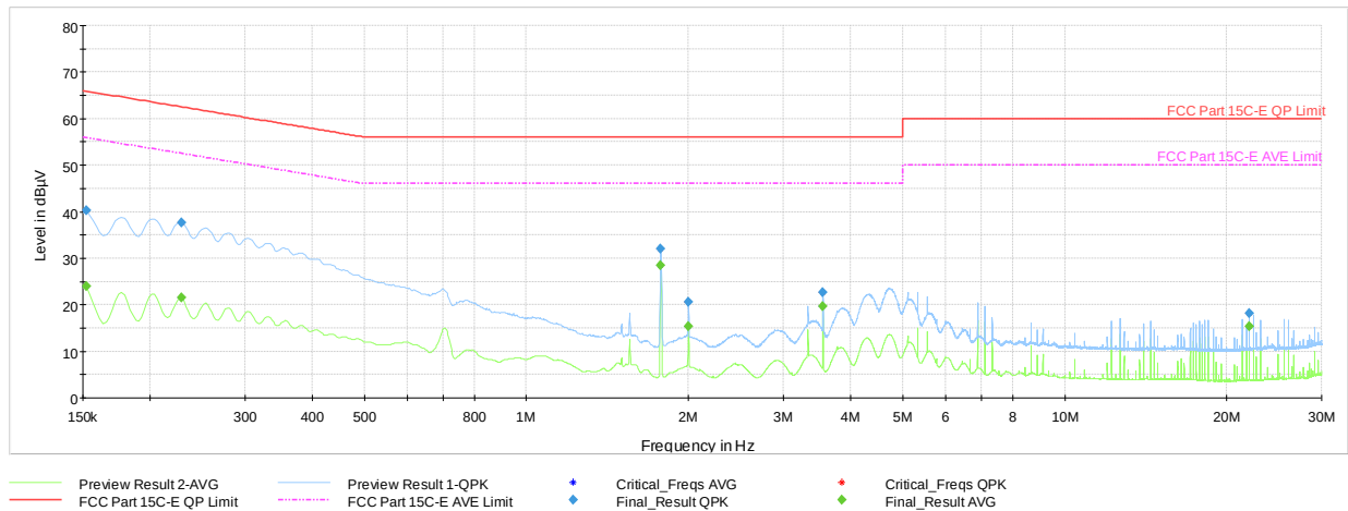
Plot 7-43. AC Line-Conducted Test Plot (N, GFSK ePA – Ch.0, with AC/DC Adapter + Magnetic Charger)
