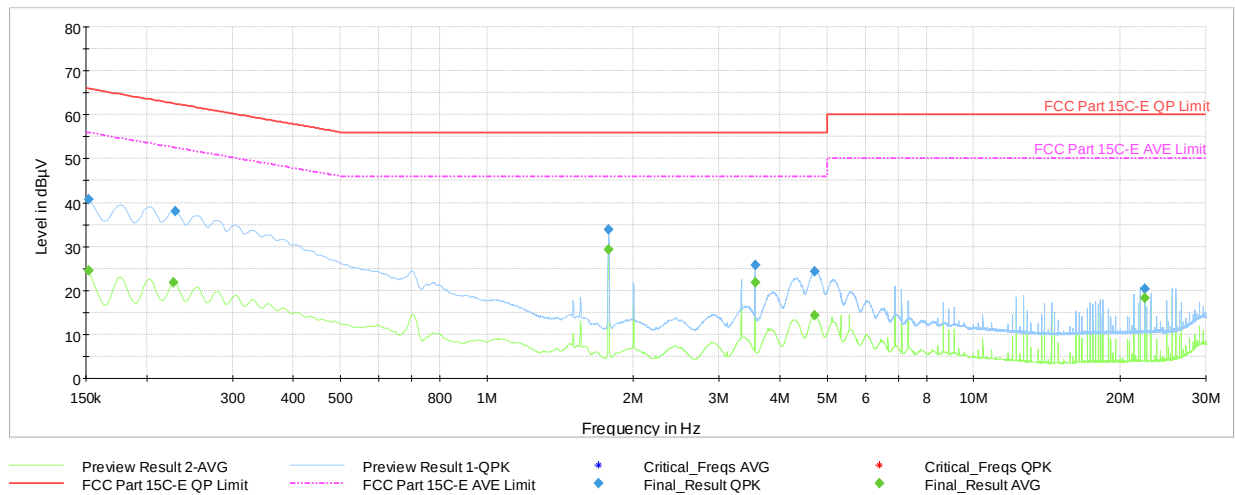
Plot 7-42. AC Line-Conducted Test Plot (L1, GFSK ePA – Ch.0, with AC/DC Adapter + Magnetic Charger)
