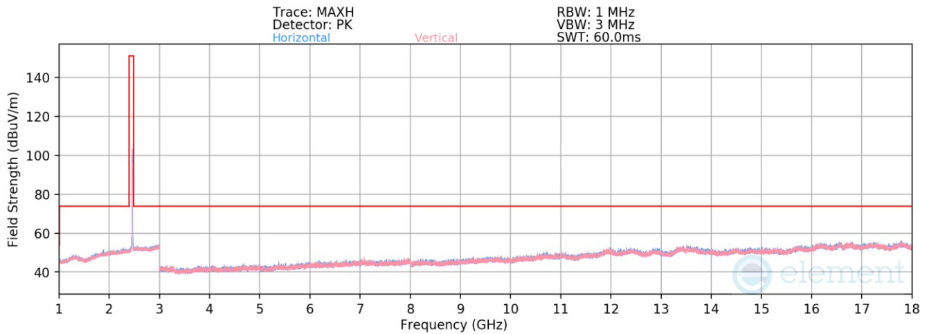
Plot 7-55. Radiated Spurious Emissions above 1GHz (802.11b – Ch. 11)
