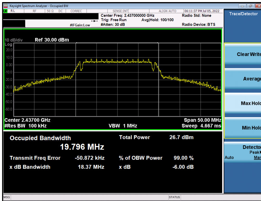
Plot 7-5. 6dB BW and 99% OBW Plot (802.11g – Ch. 6) – 6Mbps
