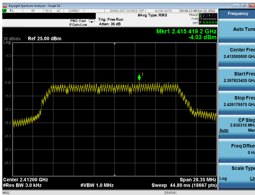
Plot 7-22. Power Spectral Density Plot (802.11n MCS7 – Ch. 1)
