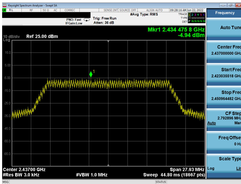
Plot 7-20. Power Spectral Density Plot (802.11n MCS0 – Ch. 6)
