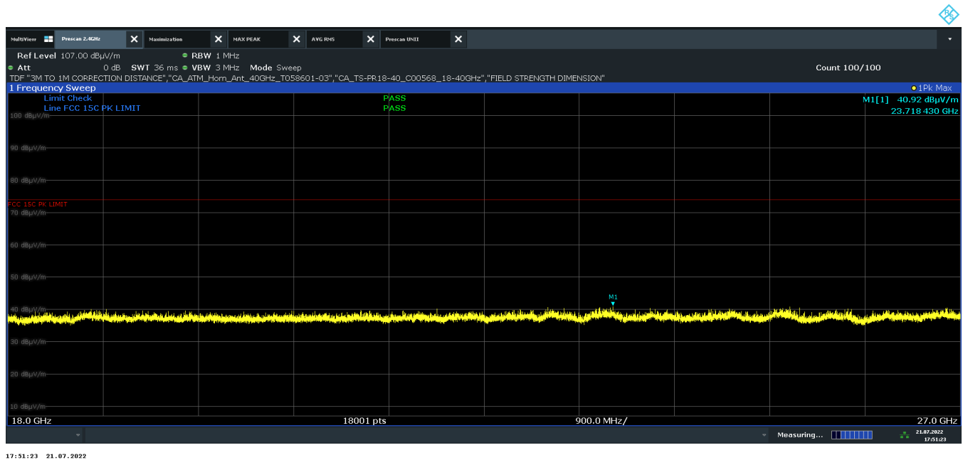
Plot 7-56. Radiated Spurious Plot above 18GHz (802.11b – Ch. 6 Ant. Pol H)
