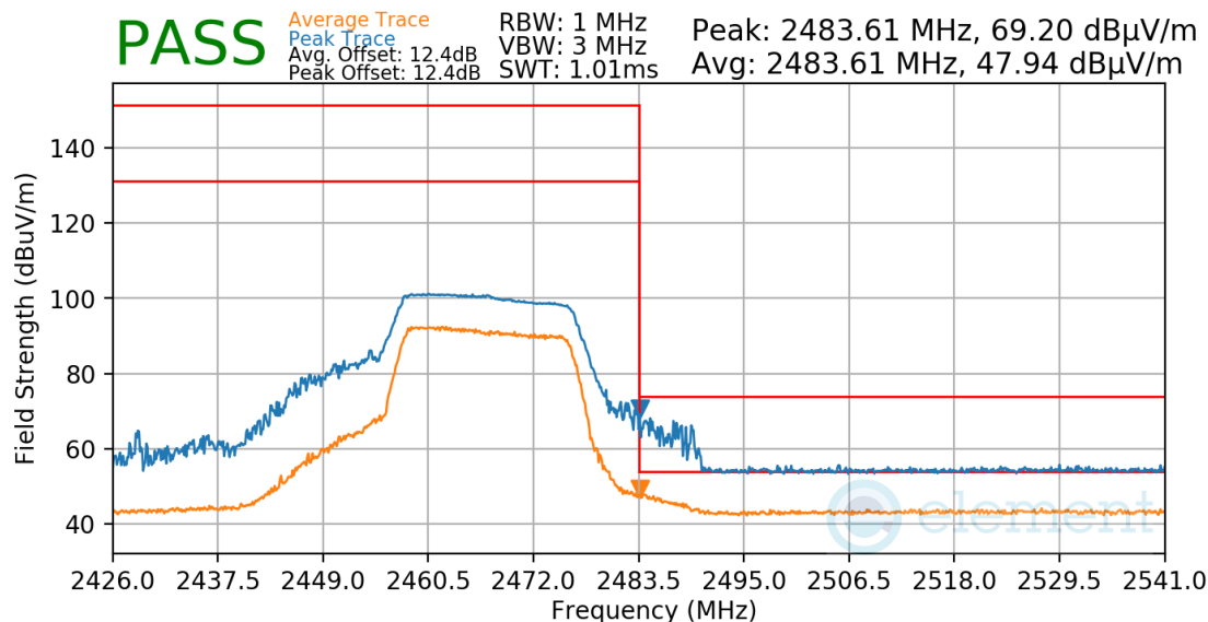
Plot 7-67. Radiated Restricted Upper Band Edge Measurement
