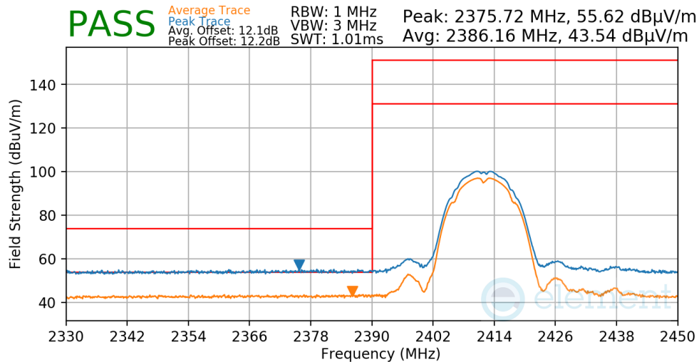
Plot 7-58. Radiated Restricted Lower Band Edge Measurement
