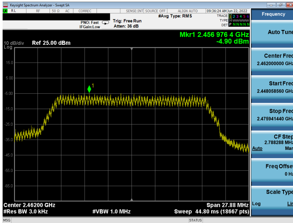
Plot 7-21. Power Spectral Density Plot (802.11n MCS0 – Ch. 11)
