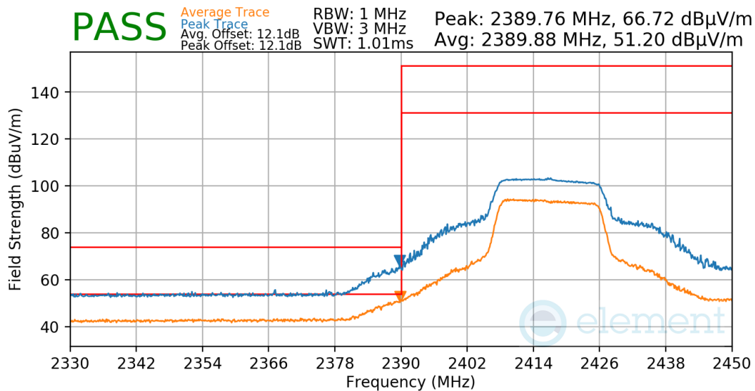
Plot 7-63. Radiated Restricted Lower Band Edge Measurement
