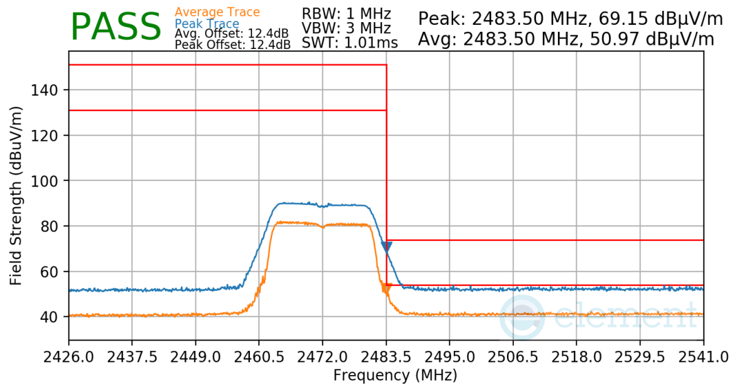
Plot 7-68. Radiated Restricted Upper Band Edge Measurement
