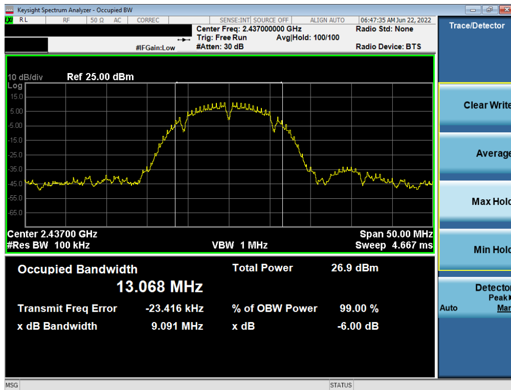
Plot 7-2. 6dB BW and 99% OBW Plot (802.11b – Ch. 6) – 1Mbps
