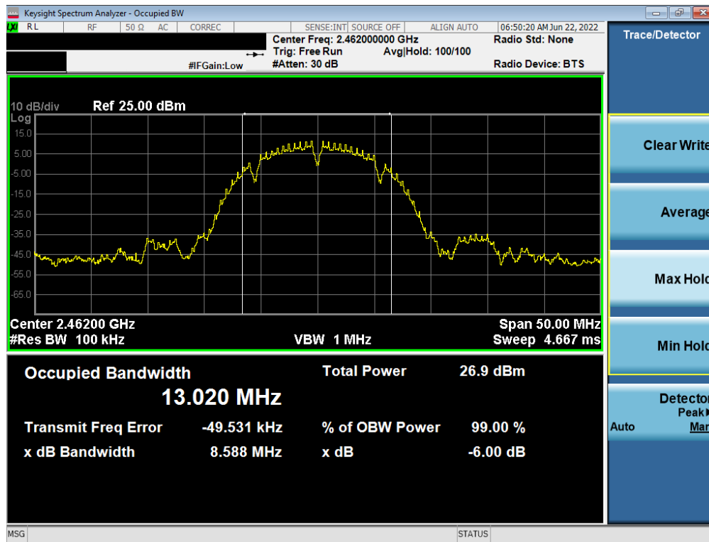
Plot 7-3. 6dB BW and 99% OBW Plot (802.11b – Ch. 11) – 1Mbps
