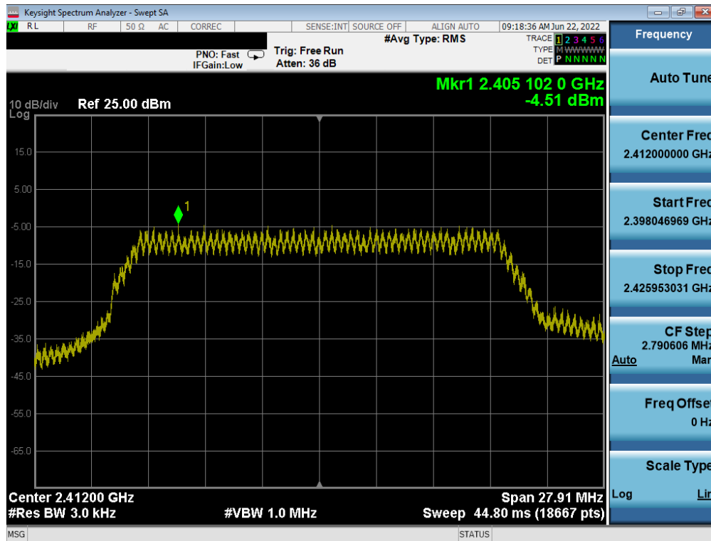
Plot 7-19. Power Spectral Density Plot (802.11n MCS0 – Ch. 1)
