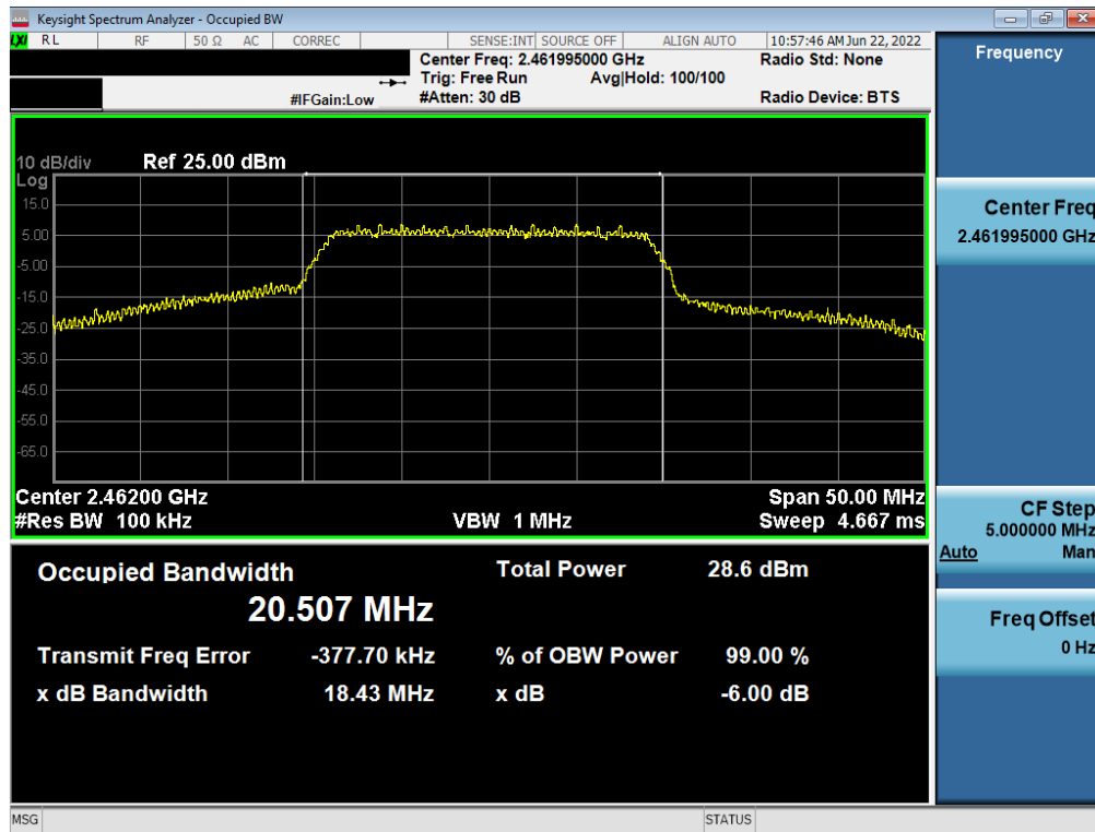
Plot 7-12. 6dB BW and 99% OBW Plot (802.11n (2.4GHz) – Ch. 11) – MCS7
