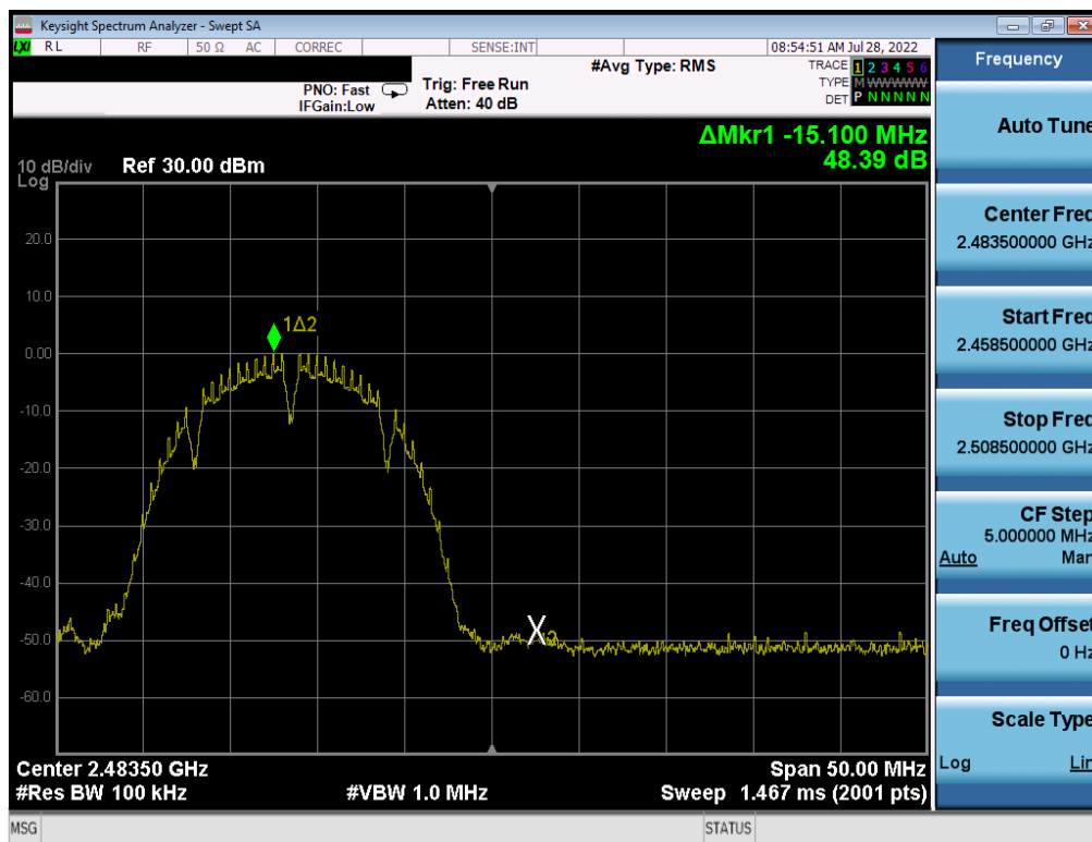
Plot 7-28. Band Edge Plot (802.11b – Ch. 13)
