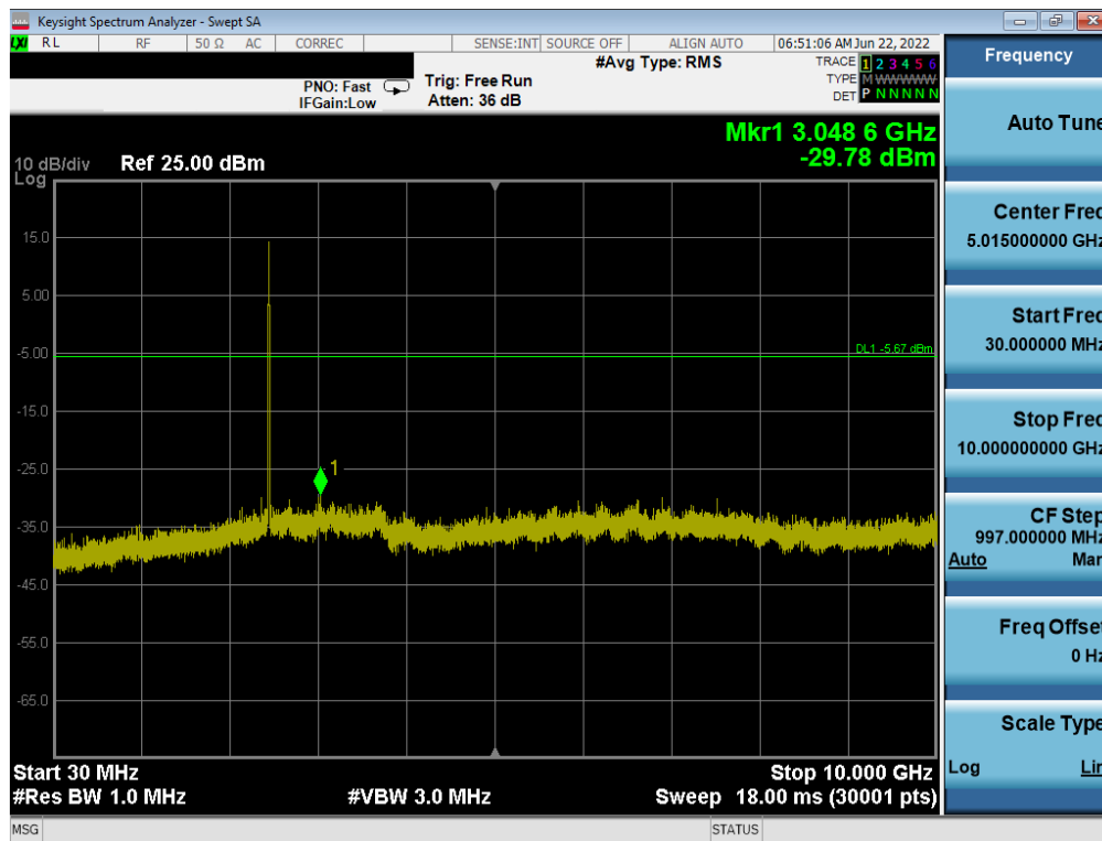
Plot 7-51. Conducted Spurious Plot Antenna 1 (802.11b – Ch. 11)
