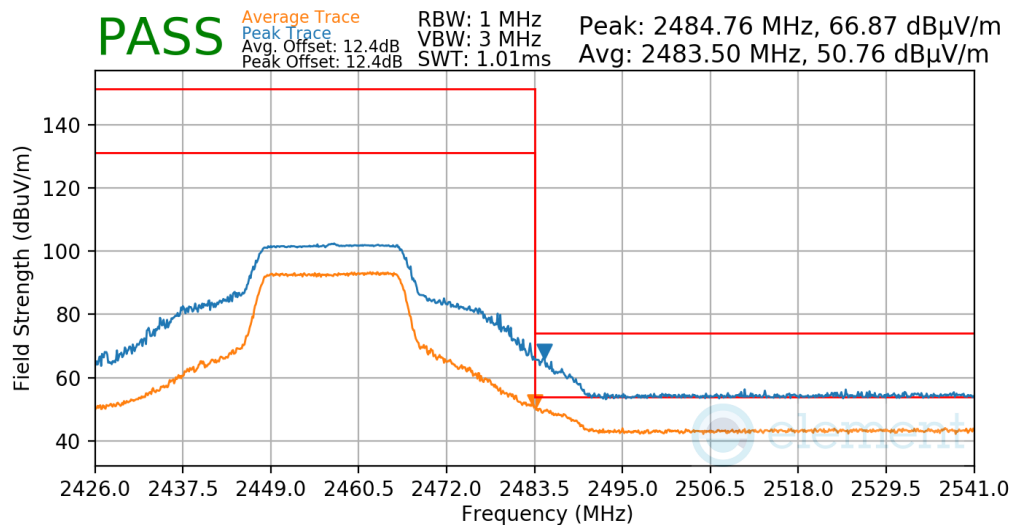
Plot 7-65. Radiated Restricted Upper Band Edge Measurement
