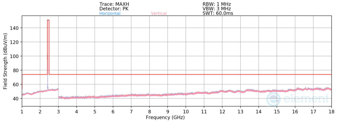
Plot 7-53. Radiated Spurious Emissions above 1GHz (802.11b – Ch. 1)
