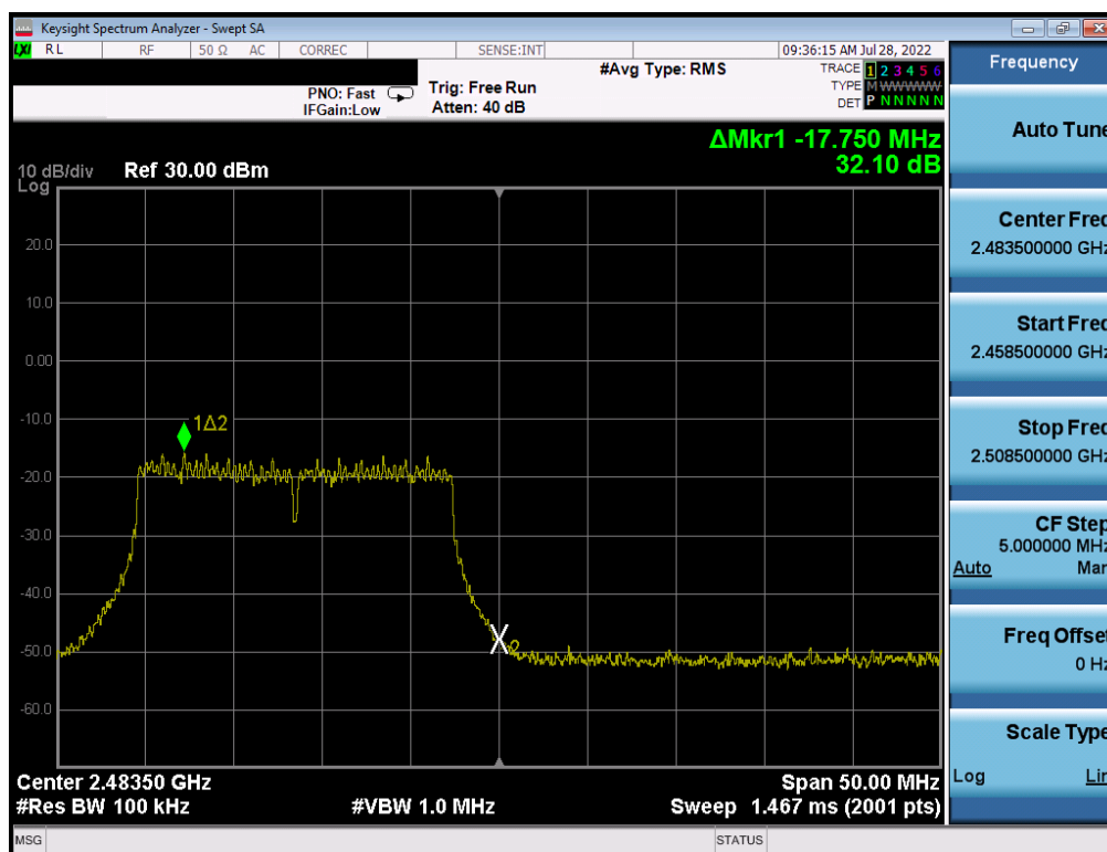
Plot 7-46. Band Edge Plot (802.11n (2.4GHz) – Ch. 13) – MCS7
