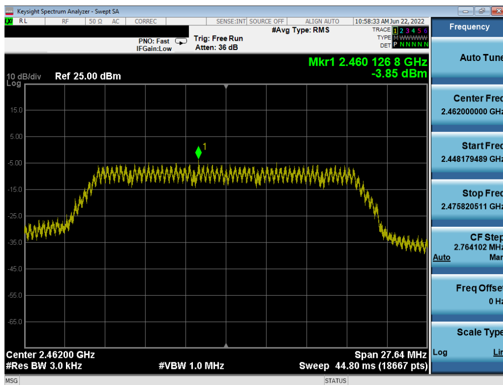
Plot 7-24. Power Spectral Density Plot (802.11n MCS7 – Ch. 11)
