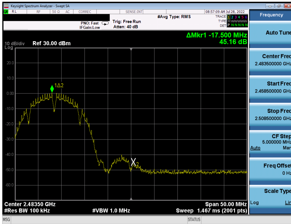
Plot 7-27. Band Edge Plot (802.11b – Ch. 12)
