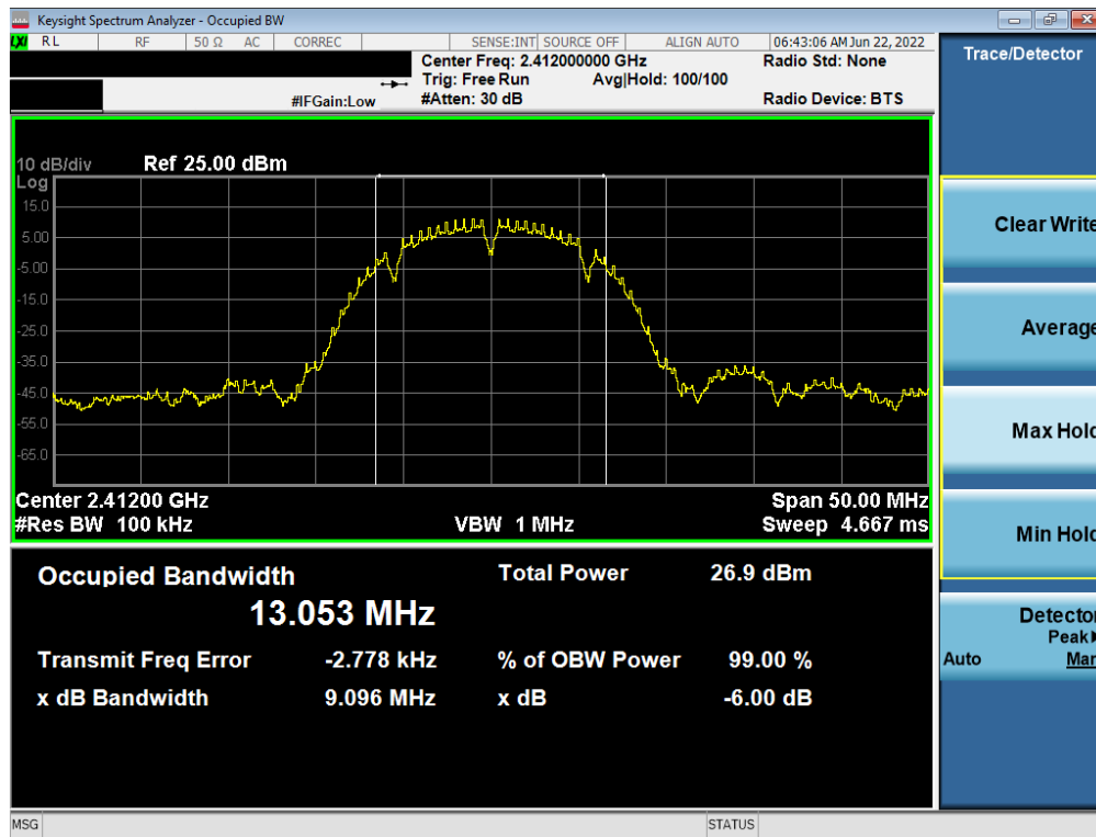
Plot 7-1. 6dB BW and 99% OBW Plot (802.11b – Ch. 1) – 1Mbps
