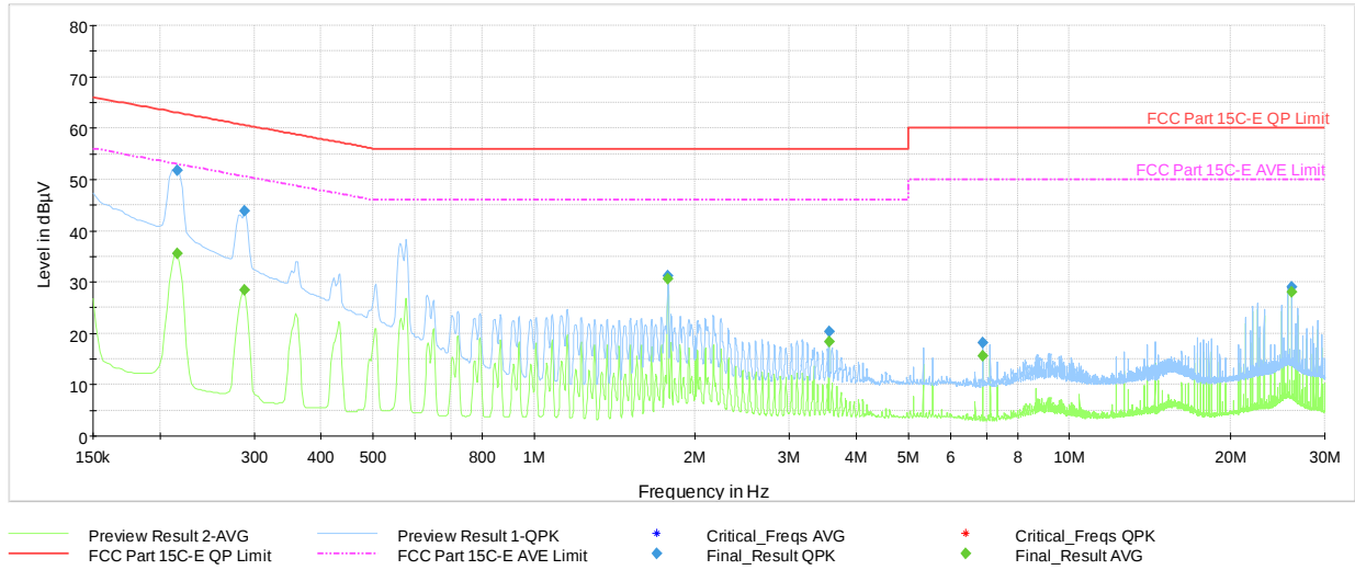
Plot 7-75. AC Line Conducted Plot 802.11b - Ch.6 (N), with Laptop
