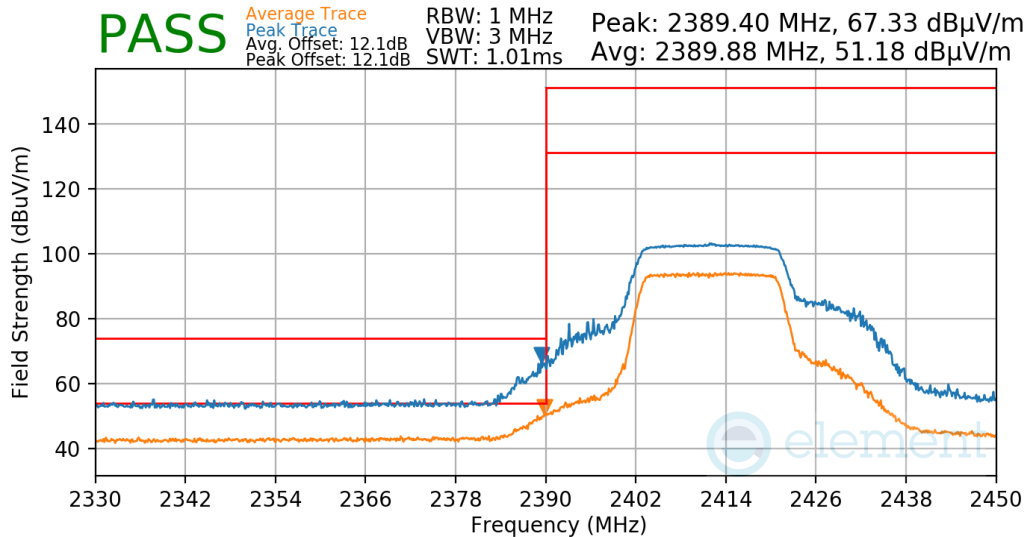
Plot 7-62. Radiated Restricted Lower Band Edge Measurement
