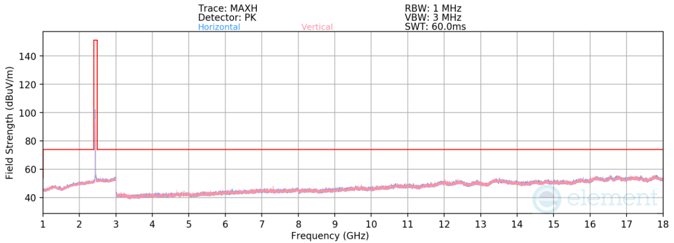
Plot 7-54. Radiated Spurious Emissions above 1GHz (802.11b – Ch. 6)
