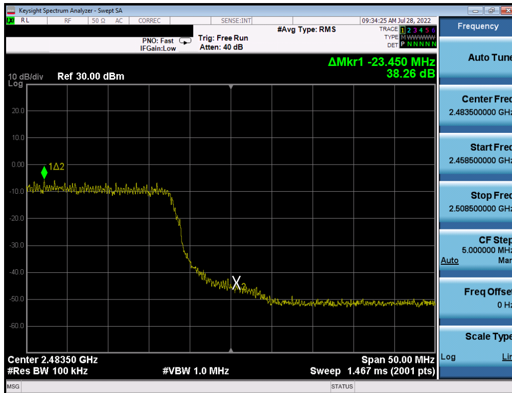
Plot 7-45. Band Edge Plot (802.11n (2.4GHz) – Ch. 12) – MCS7
