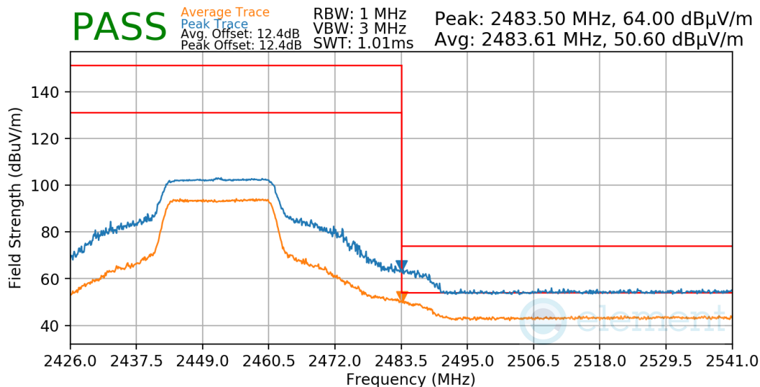
Plot 7-64. Radiated Restricted Upper Band Edge Measurement
