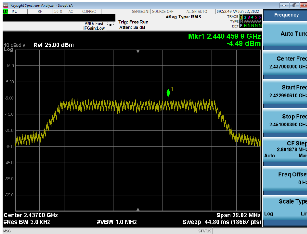
Plot 7-23. Power Spectral Density Plot (802.11n MCS7 – Ch. 6)
