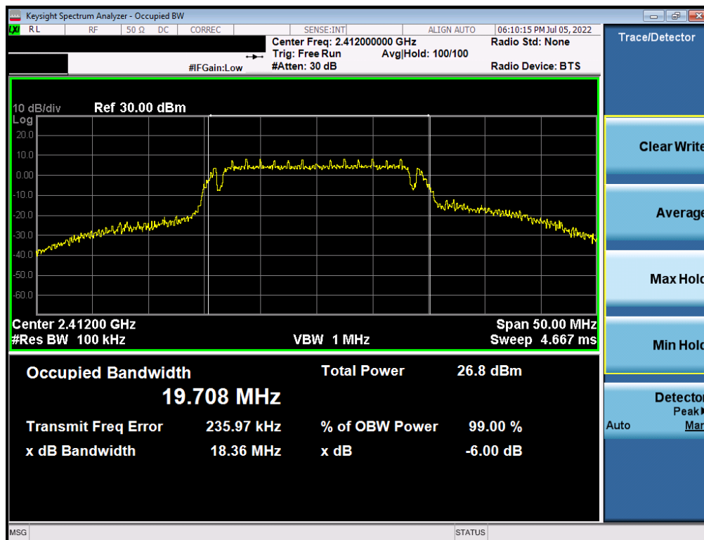
Plot 7-4. 6dB BW and 99% OBW Plot (802.11g – Ch. 1) – 6Mbps
