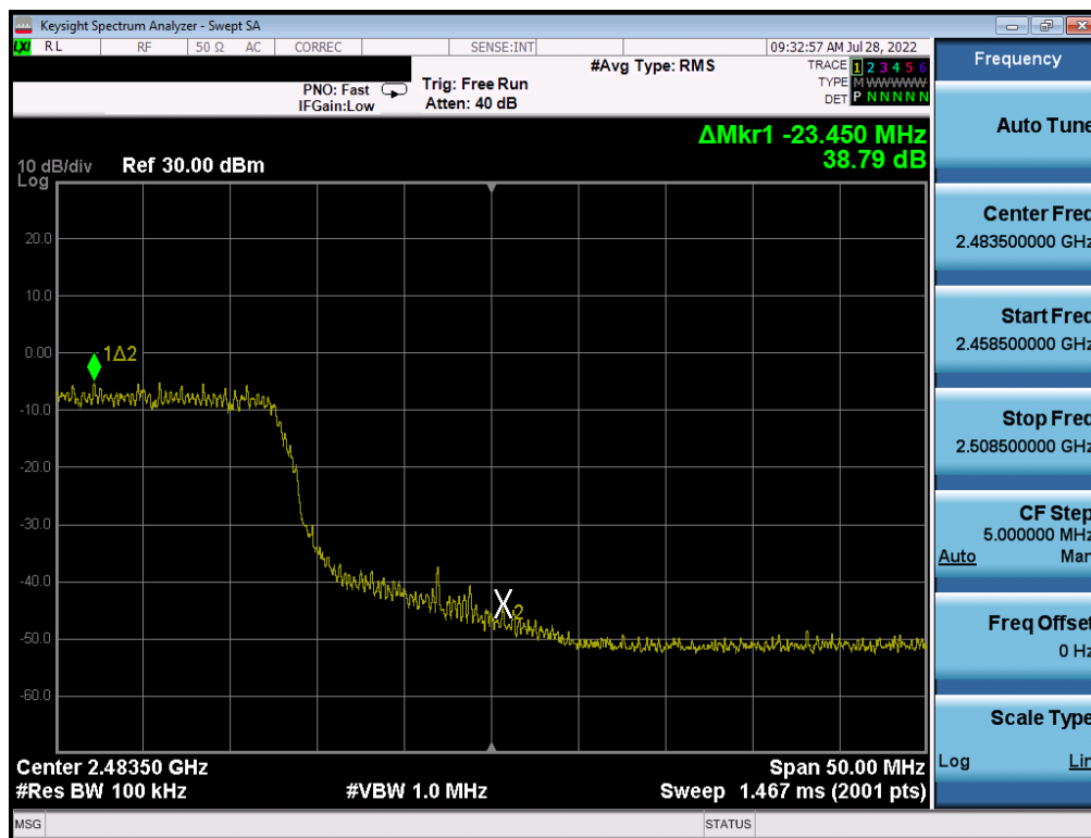
Plot 7-44. Band Edge Plot (802.11n (2.4GHz) – Ch. 11) – MCS7
