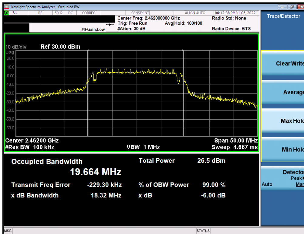
Plot 7-6. 6dB BW and 99% OBW Plot (802.11g – Ch. 11) – 6Mbps
