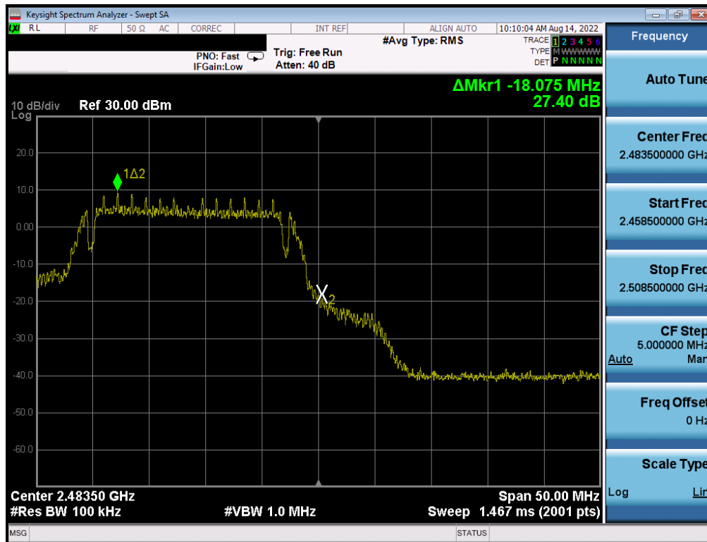
Plot 7-35. Band Edge Plot (802.11g – Ch. 13) – 6Mbps
