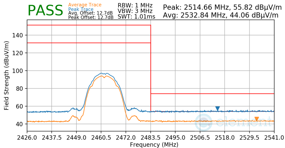
Plot 7-59. Radiated Restricted Upper Band Edge Measurement
