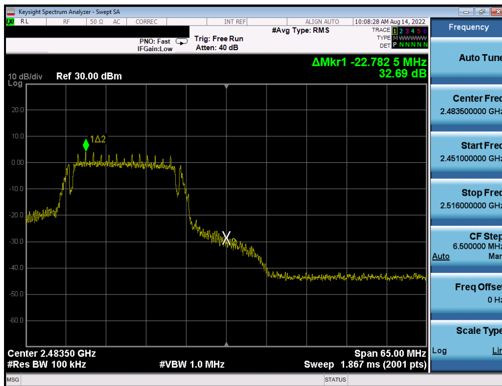
Plot 7-34. Band Edge Plot (802.11g – Ch. 12) – 6Mbps
