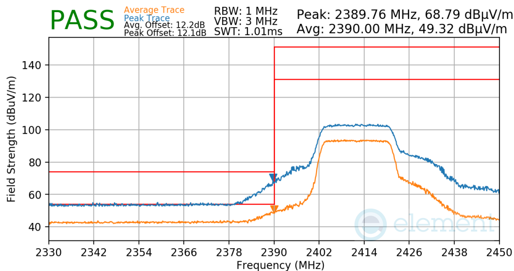
Plot 7-69. Radiated Restricted Lower Band Edge Measurement
