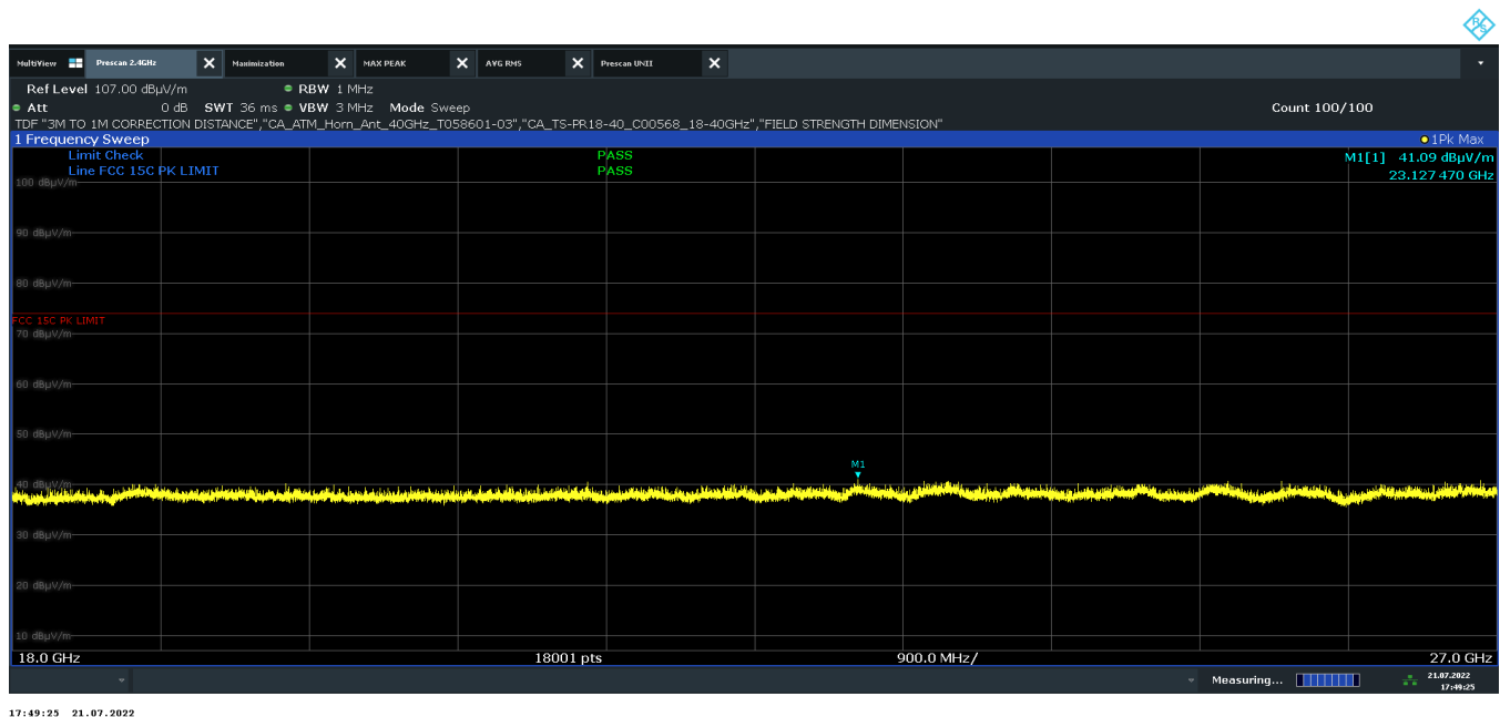
Plot 7-57. Radiated Spurious Plot above 18GHz (802.11b – Ch. 6 Ant. Pol V)
