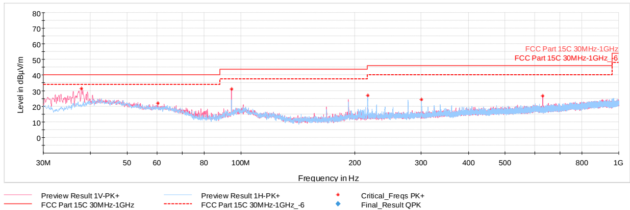
Plot 7-73. Radiated Spurious Emissions below 1GHz 802.11b Ch.6, with AC/DC Adapter and Magnetic Charger
