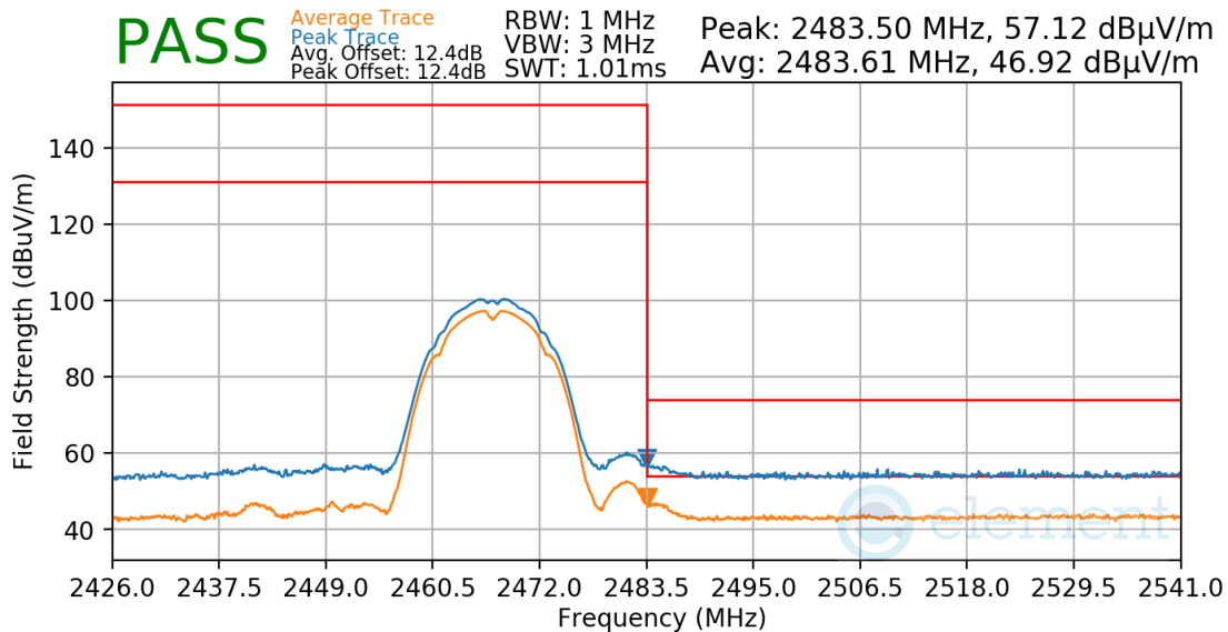
Plot 7-60. Radiated Restricted Upper Band Edge Measurement
