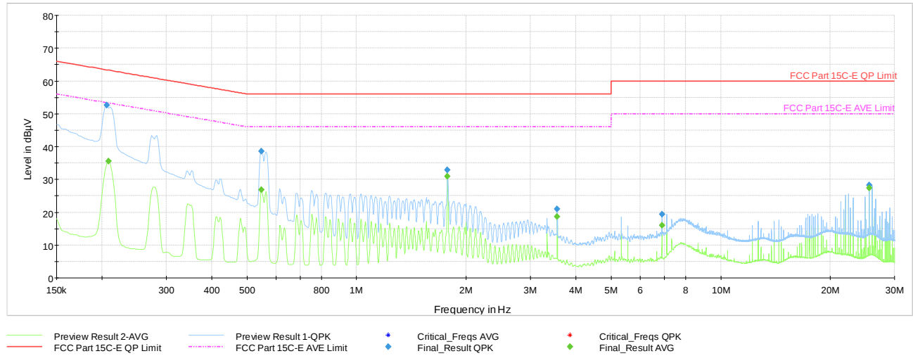
Plot 7-74. AC Line Conducted Plot 802.11n - Ch.6 (L1), with Laptop
