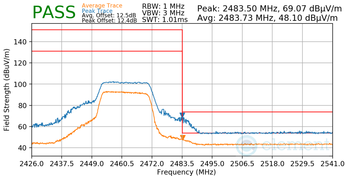
Plot 7-66. Radiated Restricted Upper Band Edge Measurement
