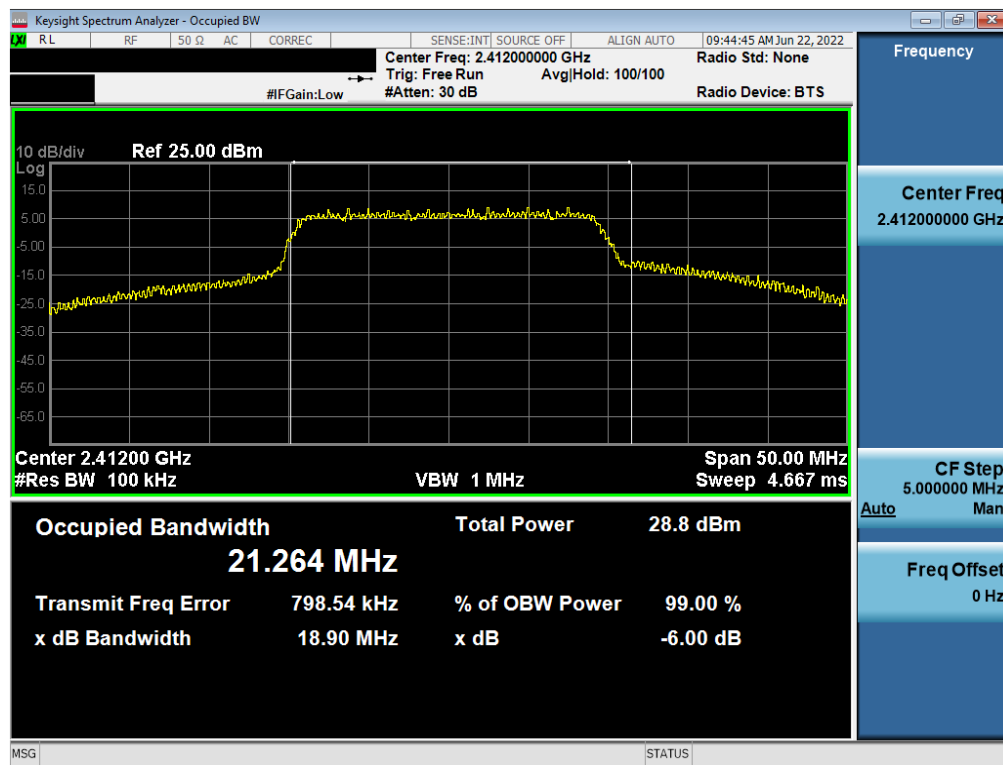
Plot 7-10. 6dB BW and 99% OBW Plot (802.11n (2.4GHz) – Ch. 1) – MCS7
