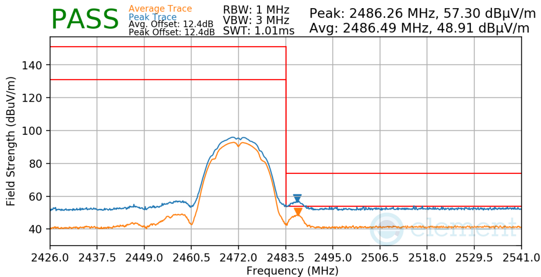
Plot 7-61. Radiated Restricted Upper Band Edge Measurement
