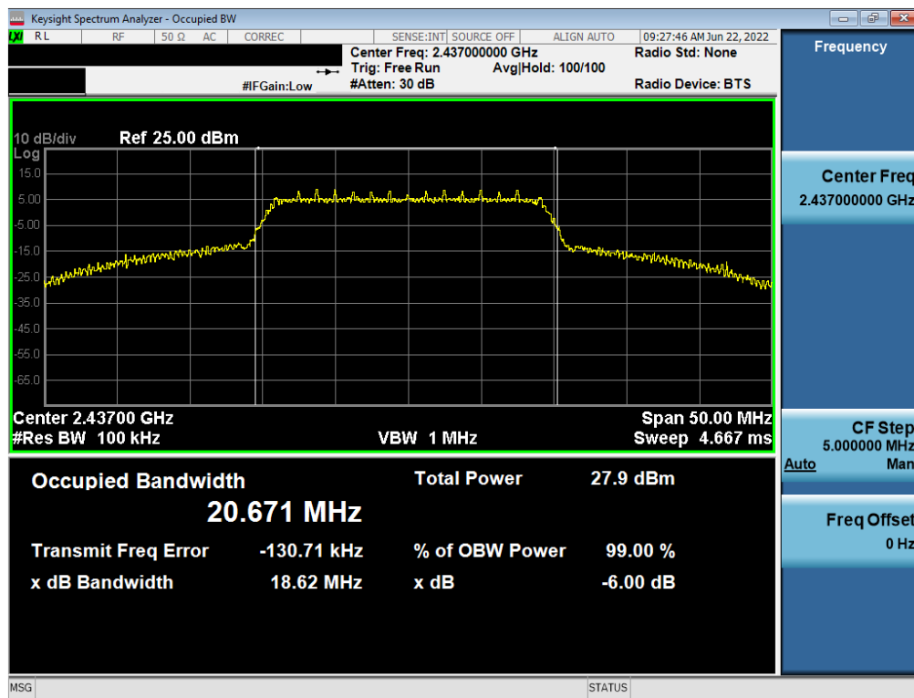
Plot 7-8. 6dB BW and 99% OBW Plot (802.11n (2.4GHz) – Ch. 6) – MCS0
