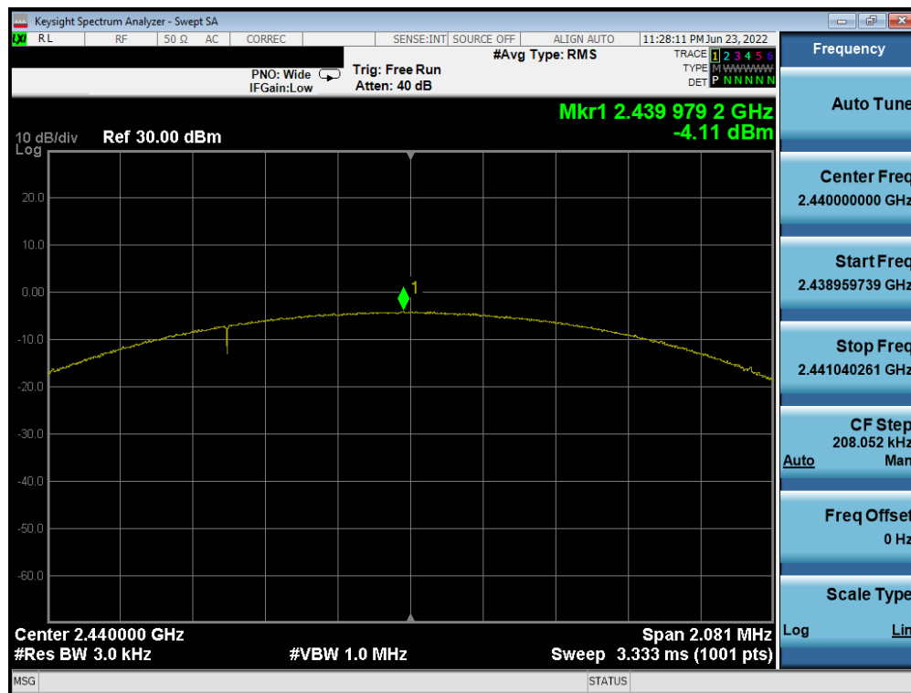
Plot 7-14. Power Spectral Density Plot (Bluetooth (LE), 2Mbps, ePA – Ch. 19)
