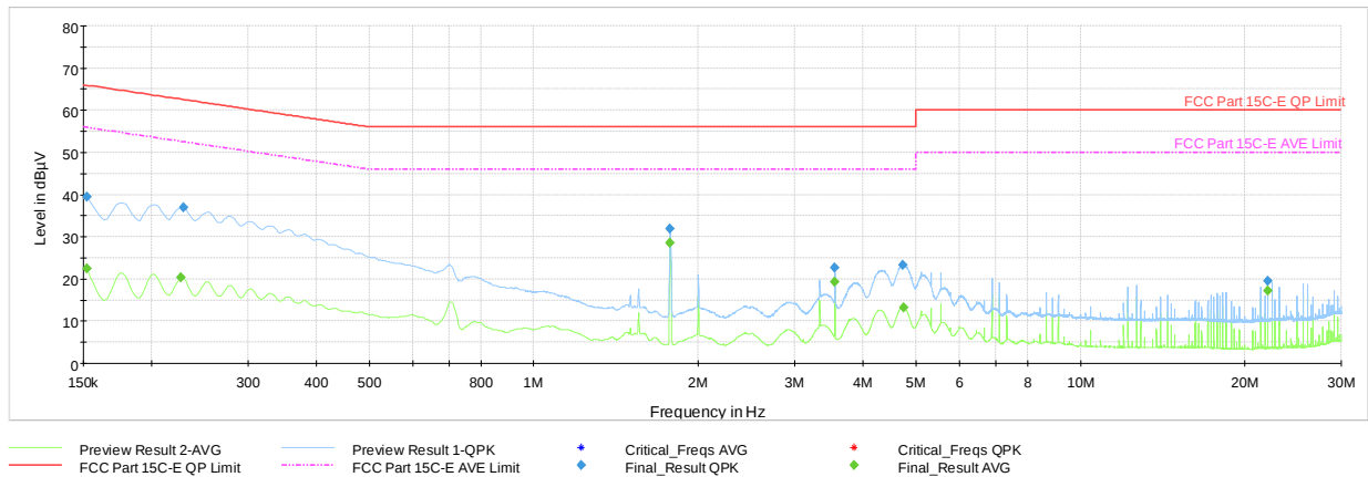
Plot 7-39. AC Line Conducted Plot with Bluetooth LE (L1, 1Mbps ePA – Ch.19 with AC/DC Adapter + Magnetic Charger)
