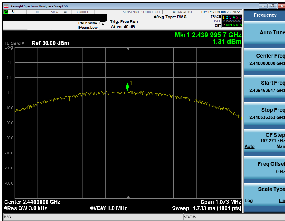
Plot 7-8. Power Spectral Density Plot (Bluetooth (LE), 1Mbps, ePA – Ch. 19)
