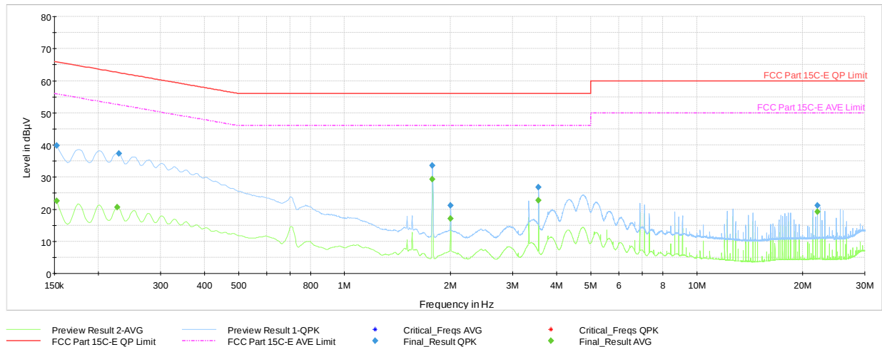
Plot 7-40. AC Line Conducted Plot with Bluetooth LE (N, 1Mbps ePA – Ch.19, with AC/DC Adapter + Magnetic Charger)
