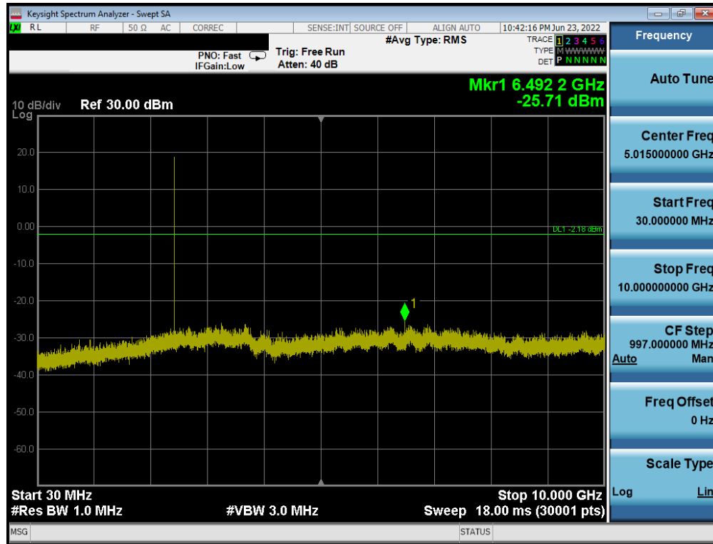
Plot 7-25. Conducted Spurious Plot (Bluetooth (LE), 1Mbps, ePA – Ch. 19)
