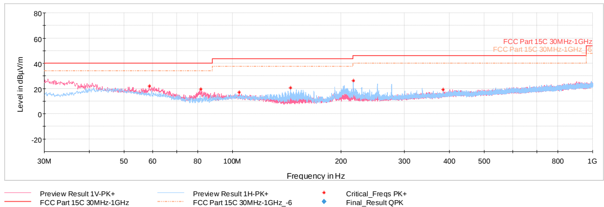
Plot 7-38. Radiated Spurious Plot (Below 1GHz 1Mbps, ePA – Ch.19, Pol. H & V, with AC/DC Adapter + Magnetic Charger)
