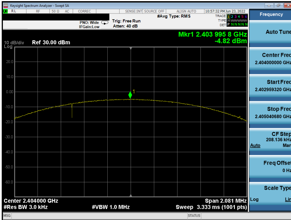
Plot 7-13. Power Spectral Density Plot (Bluetooth (LE), 2Mbps, ePA – Ch. 1)
