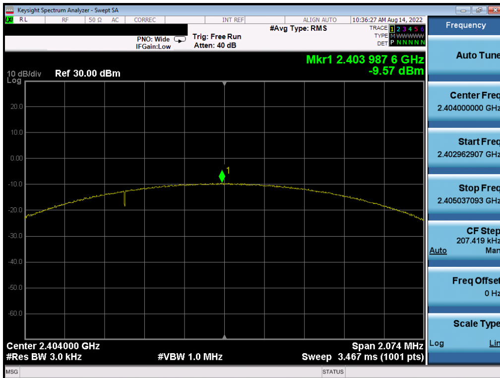
Plot 7-16. Power Spectral Density Plot (Bluetooth (LE), 2Mbps, iPA – Ch. 1)
