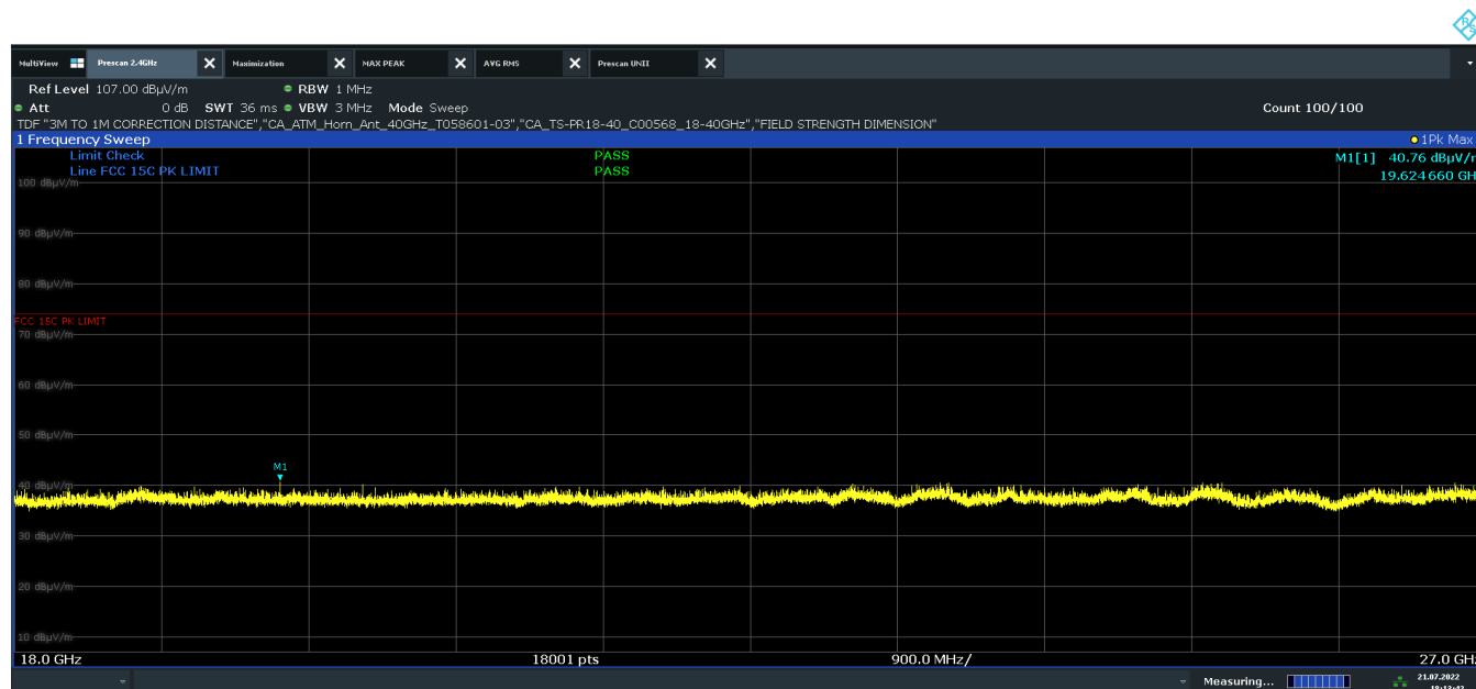
Plot 7-32. Radiated Spurious Plot Above 18GHz (1Mbps, ePA – Ch.19, Ant. Pol.H)
