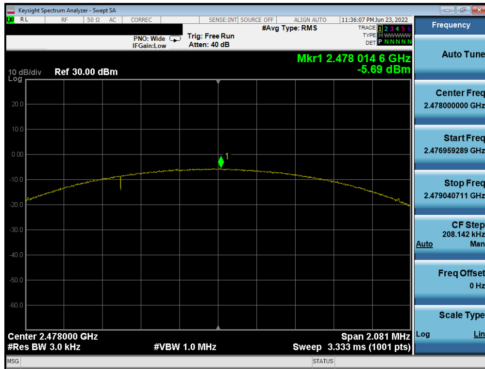
Plot 7-15. Power Spectral Density Plot (Bluetooth (LE), 2Mbps, ePA – Ch. 38)
