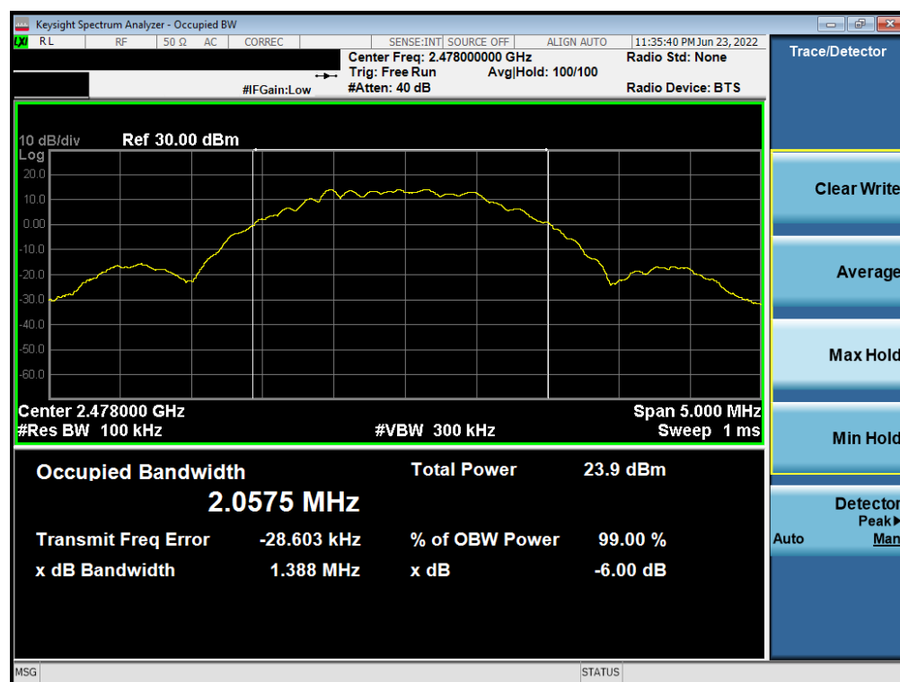
Plot 7-6. 6dB BW & 99% OBW Plot (Bluetooth (LE), 2Mbps, ePA – Ch. 38)
