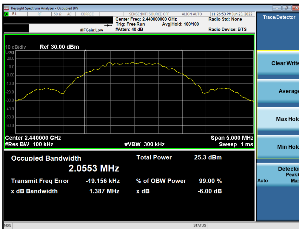
Plot 7-5. 6dB BW & 99% OBW Plot (Bluetooth (LE), 2Mbps, ePA – Ch. 19)
