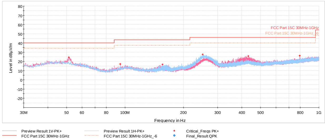
Plot 7-38. Radiated Spurious Emissions Below 1GHz (4Mbps, ePA – Ch.38, with Laptop)
