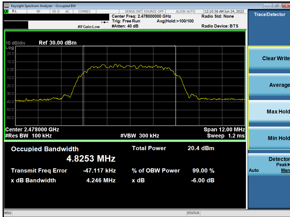
Plot 7-6. 6dB BW & 99% OBW Plot (Bluetooth (HDR8), 8Mbps, ePA – Ch. 75)
