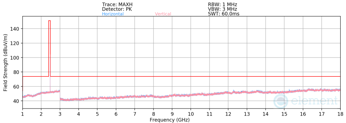
Plot 7-31. Radiated Spurious Emissions 1-18GHz (4Mbps, HDR4, ePA – Ch. 75)
