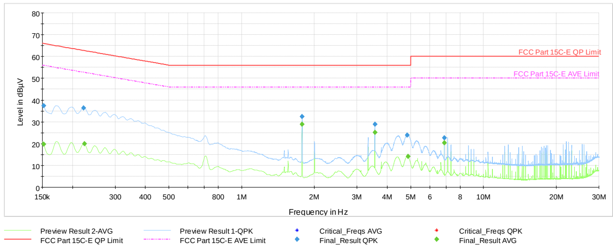
Plot 7-39. AC Line Conducted Plot with Bluetooth HDR (L1, 4Mbps ePA - Ch.38 with AC/DC Adapter + Magnetic Charger)
