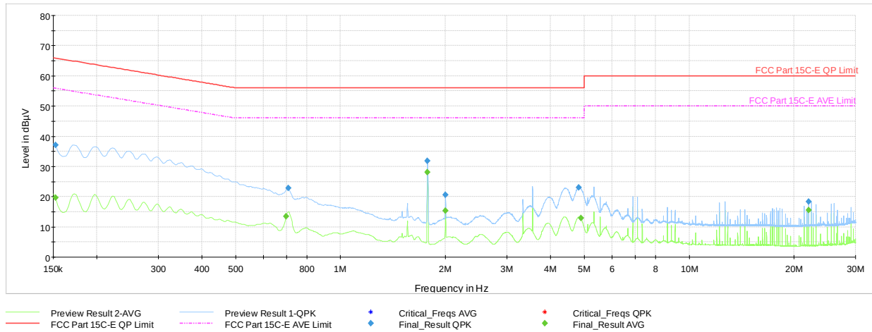
Plot 7-40. AC Line Conducted Plot with Bluetooth HDR (N, 4Mbps ePA - Ch.38 with AC/DC Adapter + Magnetic Charger)
