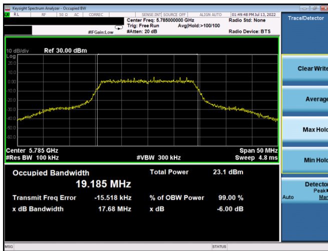
Plot 7-11. 6dB BW & 99% OBW (20MHz BW 802.11n – Ch. 157, MCS0)
