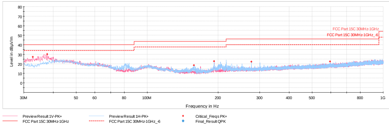
Plot 7-57. Radiated Spurious Emissions – Simultaneous Transmission 30MHz – 1GHz, with AC/DC Adapter) & Magnetic Charger
