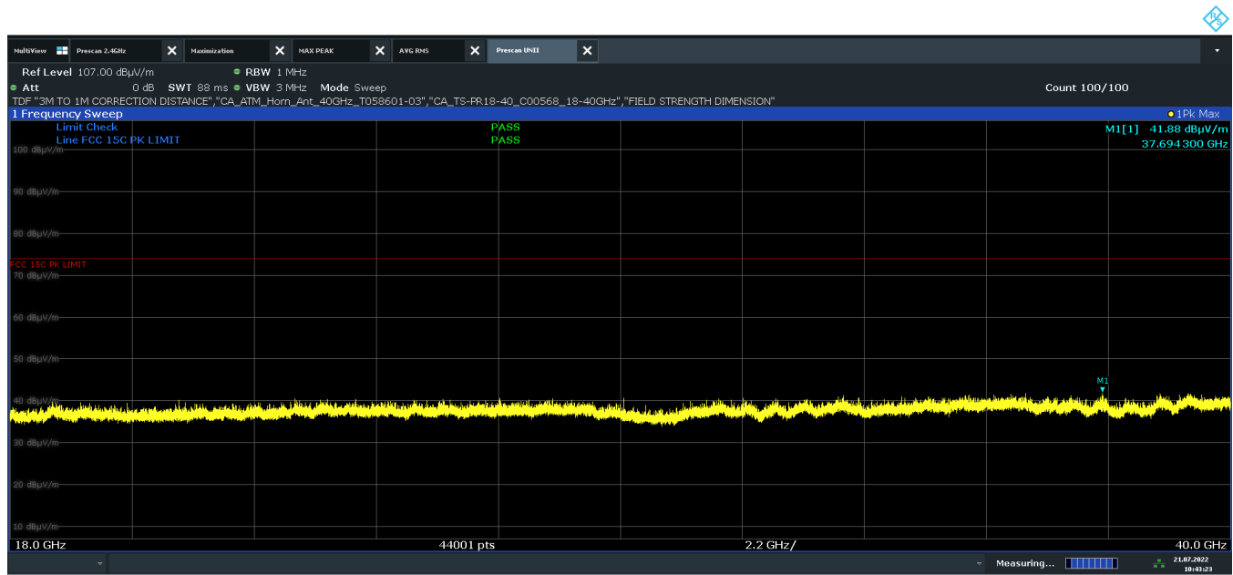
Plot 7-28. Radiated Spurious Emissions 18GHz-40GHz V Polarity (802.11n – Ch. 40)
