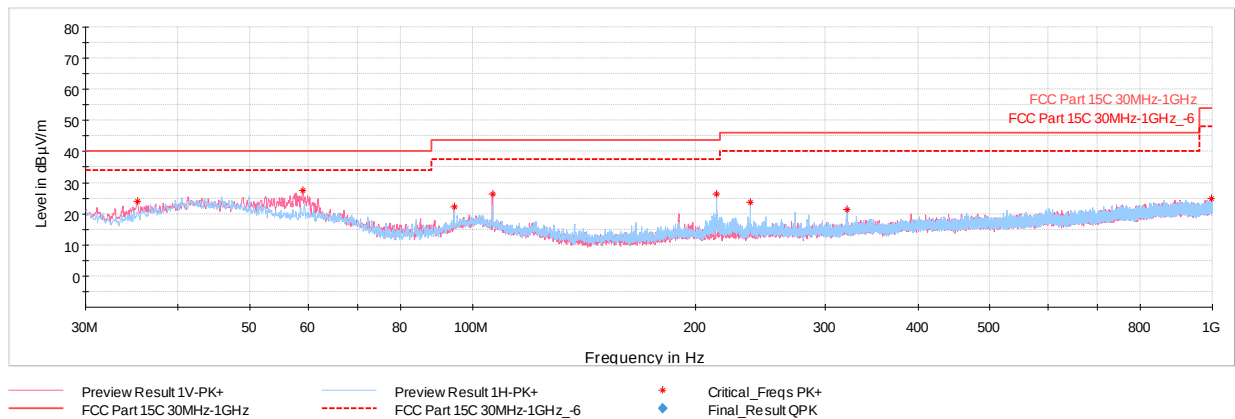
Plot 7-56. Radiated Spurious Emissions below 1GHz 802.11n, Ch.40 with AC/DC Adapter & Magnetic Charger
