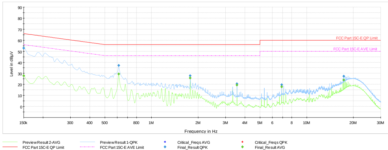
Plot 7-59. AC Line Conducted Plot with 802.11n– Ch.40 (N), with Laptop & Magnetic Charger
