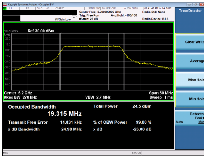
Plot 7-2. 26dB BW & 99% OBW (20MHz BW 802.11n – Ch. 40, MCS0)
