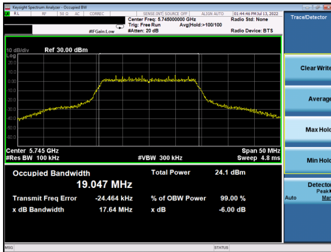
Plot 7-10. 6dB BW & 99% OBW (20MHz BW 802.11n – Ch. 149, MCS0)
