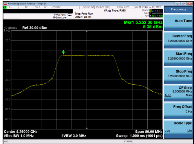
Plot 7-16. PSD (20MHz BW 802.11n - Ch. 52, MCS0)
