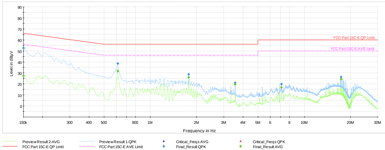
Plot 7-58. AC Line Conducted Plot with 802.11n- Ch.40 (L1), with Laptop & Magnetic Charger
