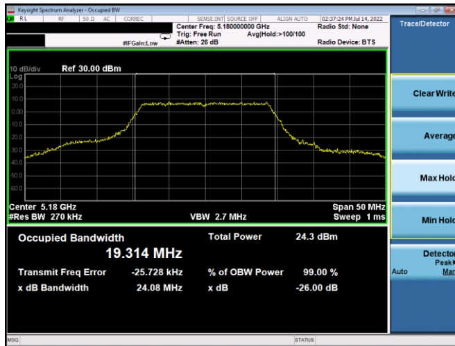
Plot 7-1. 26dB BW & 99% OBW (20MHz BW 802.11n – Ch. 36, MCS0)
