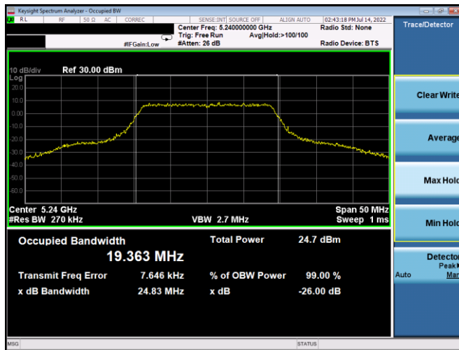
Plot 7-3. 26dB BW & 99% OBW (20MHz BW 802.11n – Ch. 48, MCS0)
