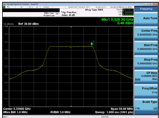
Plot 7-18. PSD (20MHz BW 802.11n - Ch. 64, MCS0)
