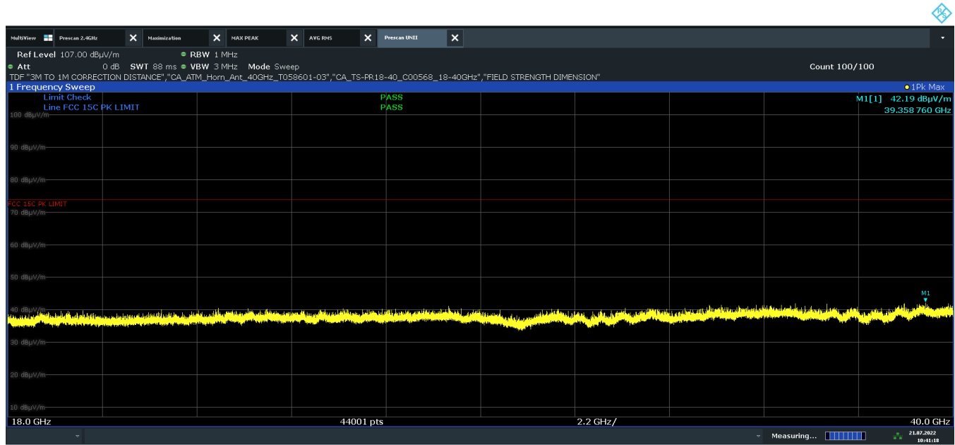
Plot 7-27. Radiated Spurious Emissions 18GHz-40GHz H Polarity (802.11n – Ch. 40)
