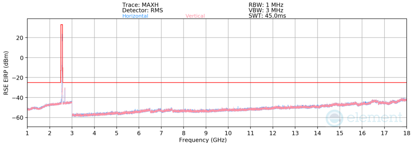
Plot 6-1. Radiated Spurious Emission 1 – 18GHz (LTE Band 7)
