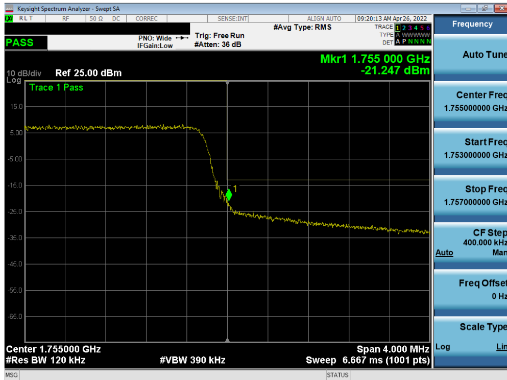
Plot 7-90. Upper Band Edge Plot (LTE Band 4 - 5MHz QPSK – Full RB)
