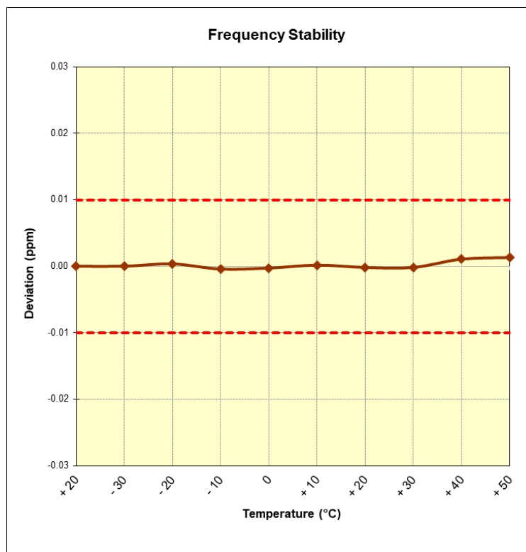
Figure 7-3. Frequency Stability Plot (CE B 848kbps)
