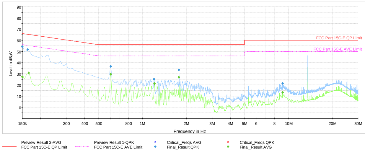
Plot 7-13. AC Line-Conducted Plot (N, CE B 106kbps, with Laptop and Magnetic Charger)
