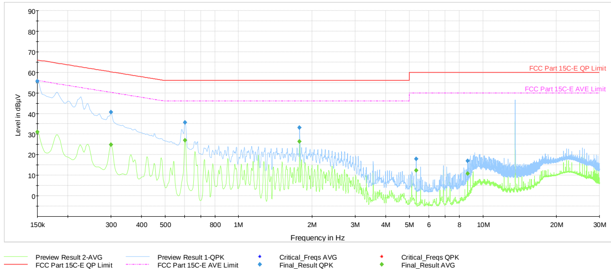
Plot 7-12. AC Line-Conducted Plot (L1, CE B 848kbps, with Laptop and Magnetic Charger)
