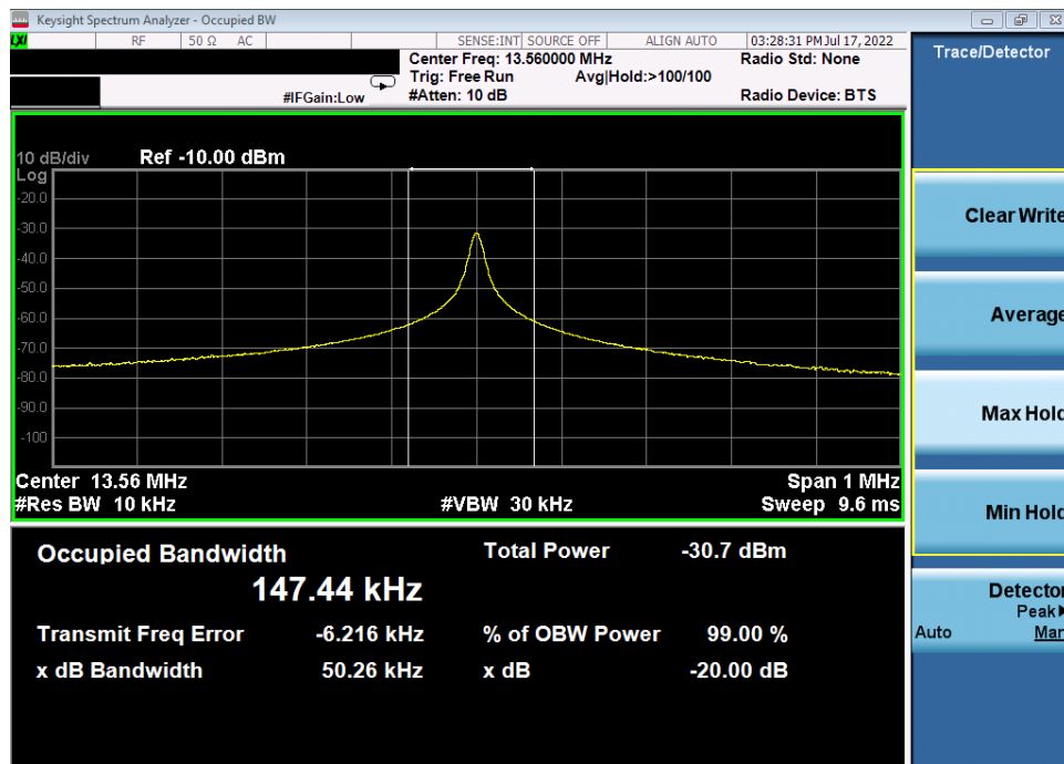
Plot 7-1. 20dB and 99% Bandwidth Plot (CE A 106kbps)
