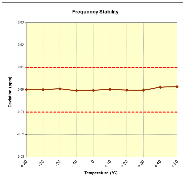
Figure 7-4. Frequency Stability Plot (Reader 100% ASK 1 out of 256)
