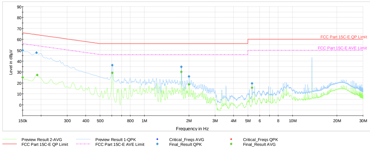
Plot 7-15. AC Line-Conducted Plot (N, Reader A 848kbps, with Laptop and Magnetic Charger)
