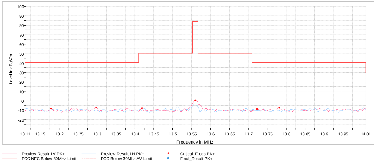
Plot 7-7. In Band Radiated Spurious Emissions (Reader A 848kbps, AC/DC Adapter and Magnetic Charger)
