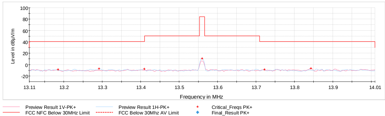
Plot 7-6. In Band Radiated Spurious Emissions (CE B 848kbps, with AC/DC Adapter and Magnetic Charger)
