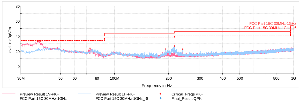
Plot 7-10. Radiated Spurious Emissions 30MHz – 1GHz (CE B 848kbps, with AC/DC Adapter and Magnetic Charger)
