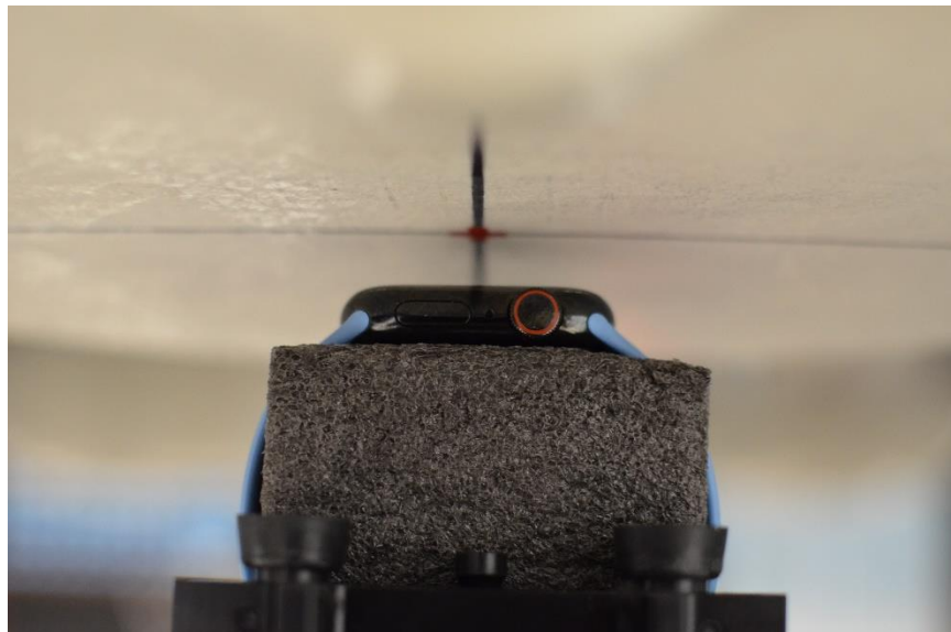
SAR Test Setup Photo 4: Stainless Steel with Sport Wristband, Head, Front Side at 1.0 cm
