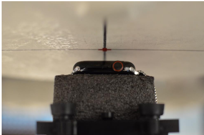
SAR Test Setup Photo 6: Stainless Steel with Metal Loop Wristband, Head, Front Side at 1.0 cm
