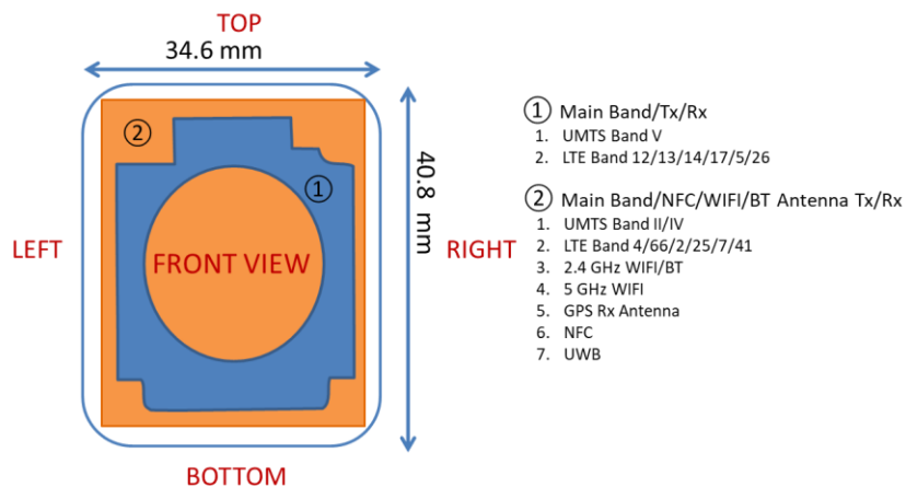
Figure E-1 DUT Antenna Locations
