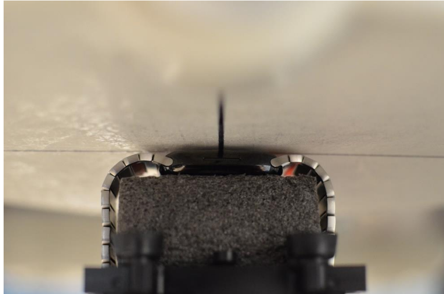
SAR Test Setup Photo 14: Stainless Steel with Metal Links Wristband, Extremity, Back Side at 0.0 cm
