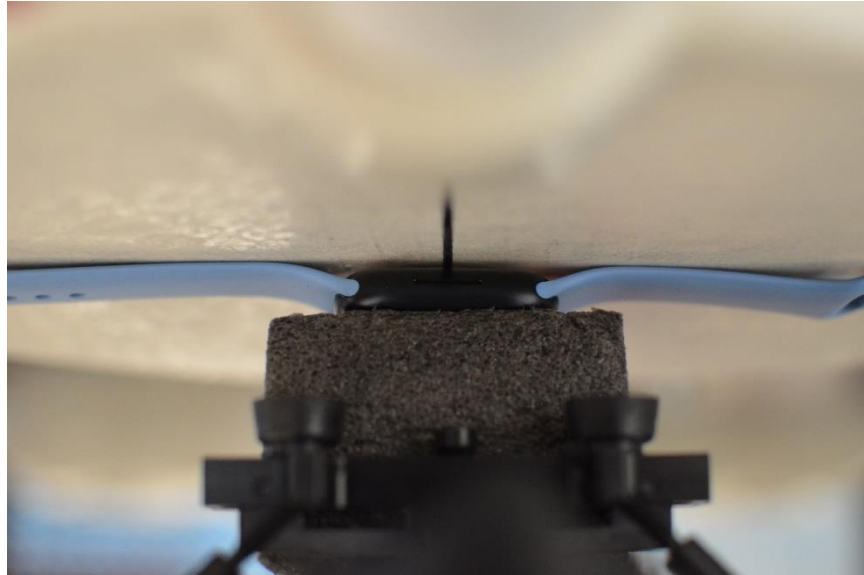
SAR Test Setup Photo 10: Aluminum with Sport Wristband, Extremity, Back Side at 0.0 cm
