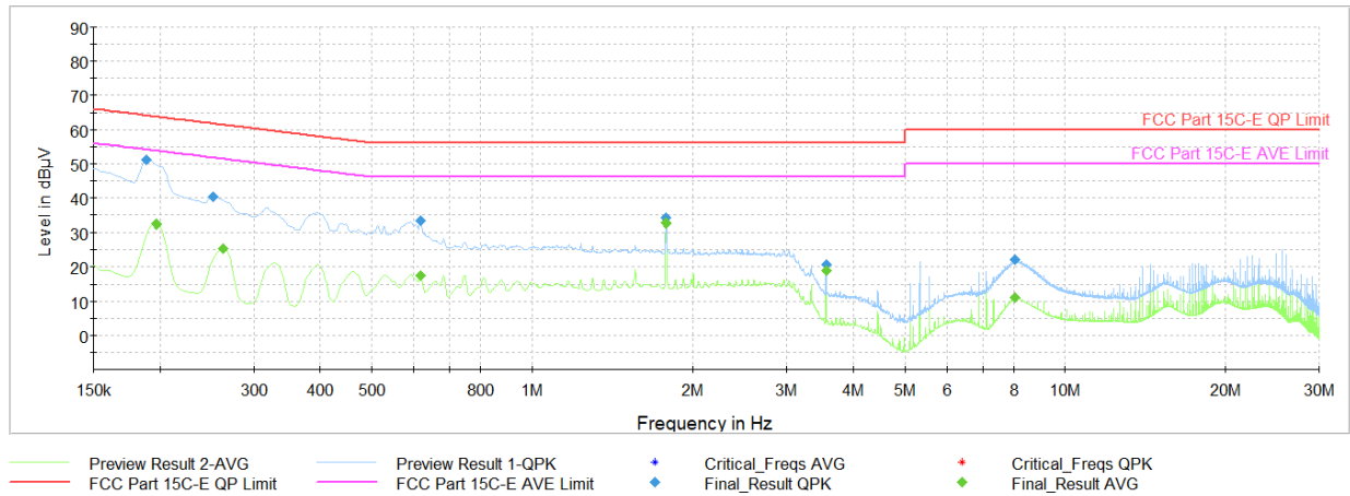
Plot 6-13. AC Line Conducted Plot (L1 - Mode 1, with Magnetic Charger & Laptop)
