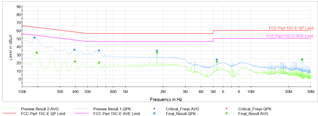
Plot 6-14. AC Line Conducted Plot (N - Mode 1, with Magnetic Charger & Laptop)
