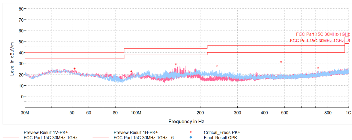
Plot 6-12. Radiated Spurious Emissions 30MHz – 1GHz (Mode 1, with Magnetic Charger & Laptop)
