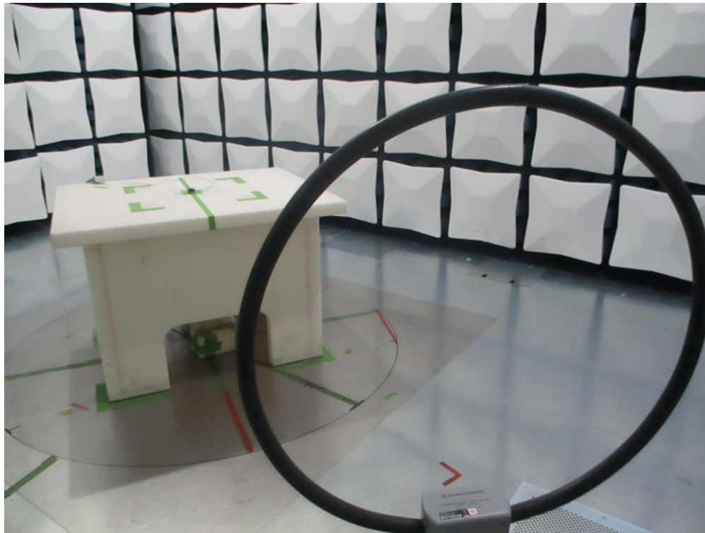
Figure 23: 9kHz-30MHz Test Setup (Front View)
