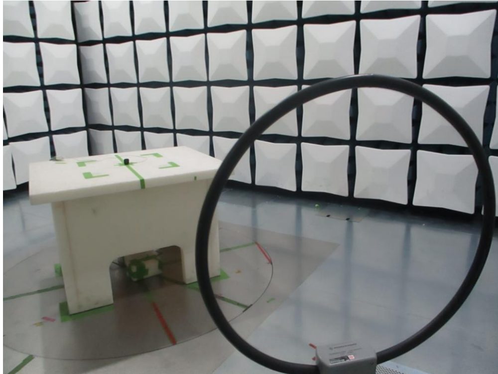
Figure 25: 9kHz-30MHz Test Setup (Front View)
