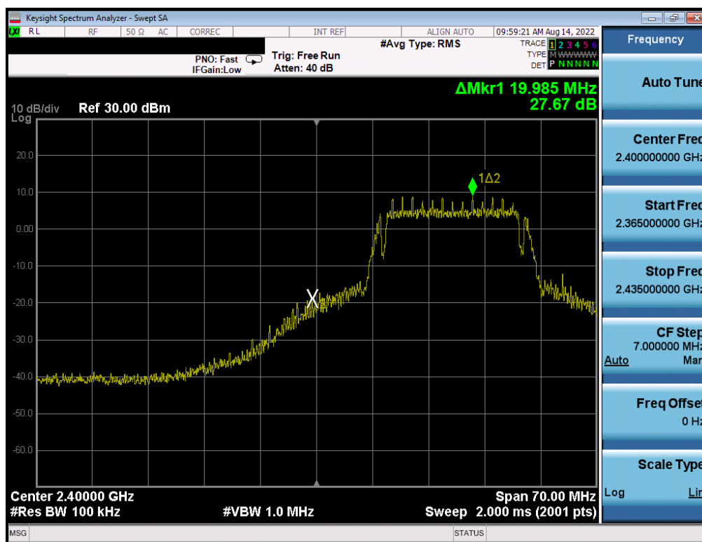
Plot 7-30. Band Edge Plot (802.11g – Ch. 2) – 6Mbps
