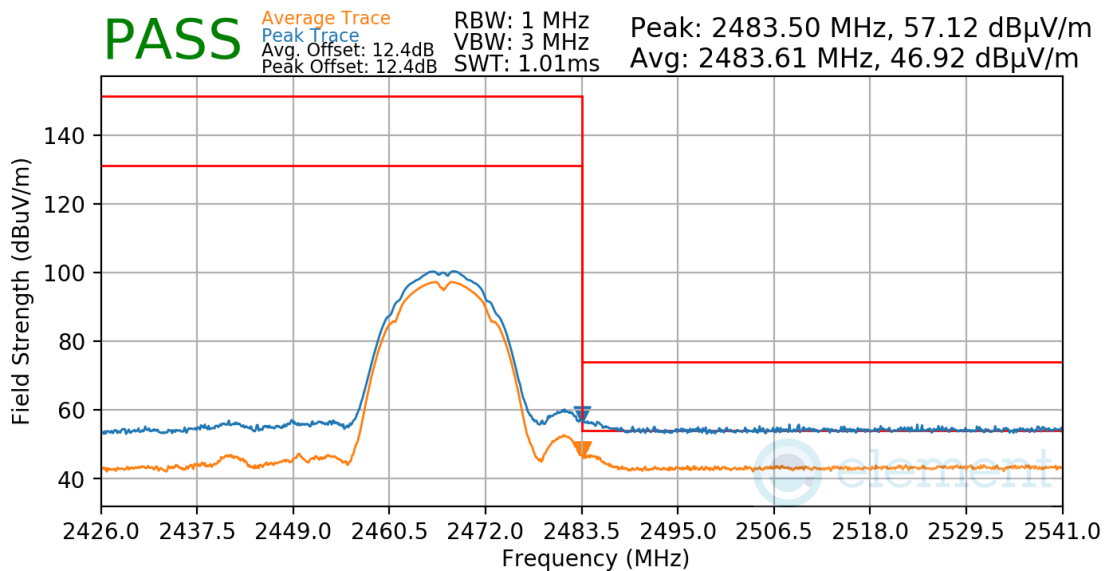
Plot 7-60. Radiated Restricted Upper Band Edge Measurement
