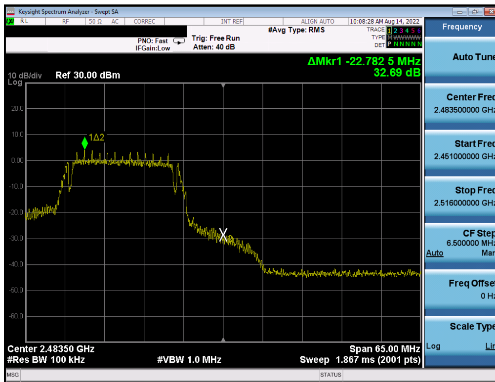
Plot 7-34. Band Edge Plot (802.11g – Ch. 12) – 6Mbps
