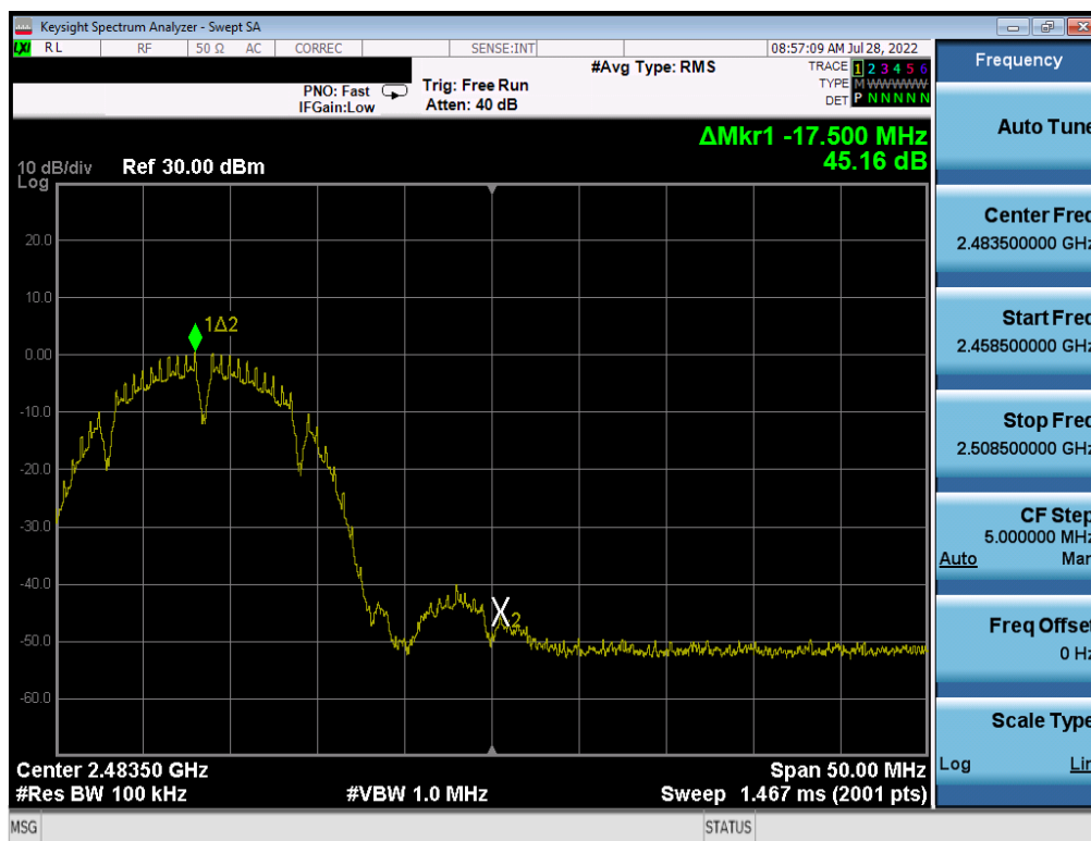
Plot 7-27. Band Edge Plot (802.11b – Ch. 12)
