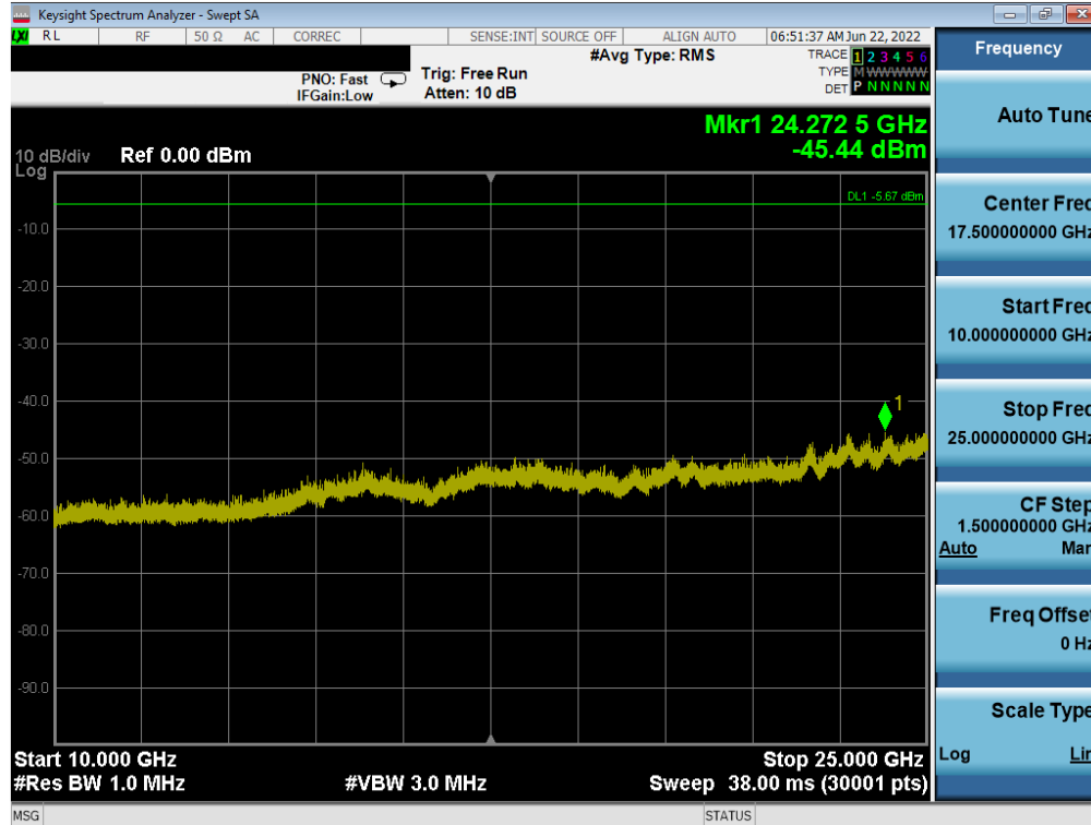
Plot 7-52. Conducted Spurious Plot Antenna 1 (802.11b – Ch. 11)
