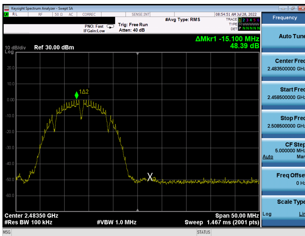
Plot 7-28. Band Edge Plot (802.11b – Ch. 13)
