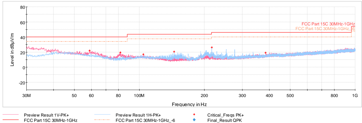
Plot 7-38. Radiated Spurious Plot (Below 1GHz 1Mbps, ePA – Ch.19, Pol. H & V, with AC/DC Adapter + Magnetic Charger)
