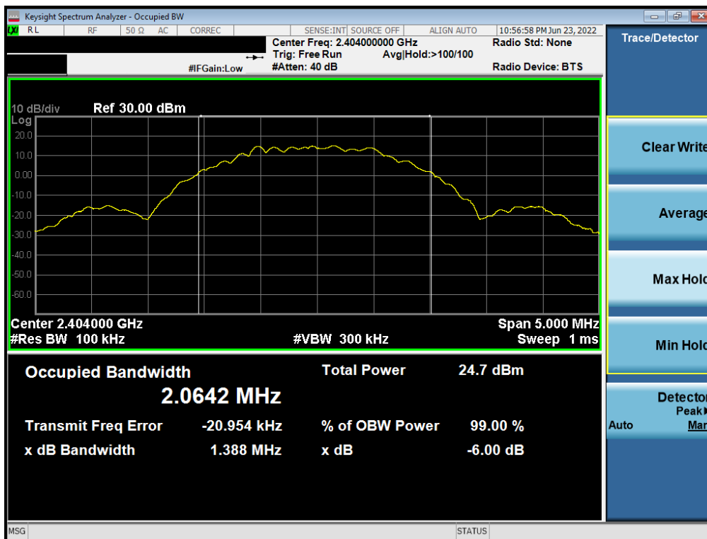
Plot 7-4. 6dB BW & 99% OBW Plot (Bluetooth (LE), 2Mbps, ePA – Ch. 1)
