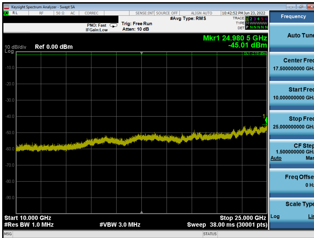
Plot 7-26. Conducted Spurious Plot (Bluetooth (LE), 1Mbps, ePA – Ch. 19)
