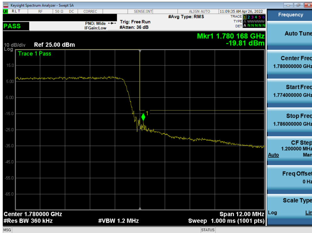
Plot 7-74. Upper Band Edge Plot (LTE Band 66 - 15MHz QPSK – Full RB)
