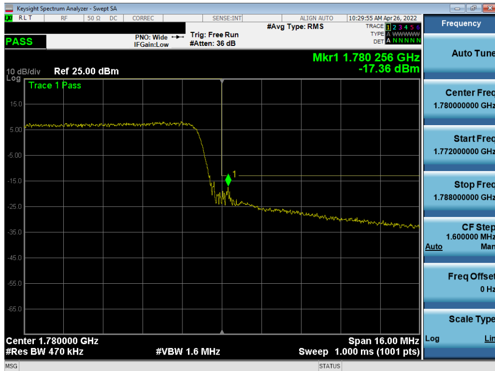
Plot 7-78. Upper Band Edge Plot (LTE Band 66 - 20MHz QPSK – Full RB)
