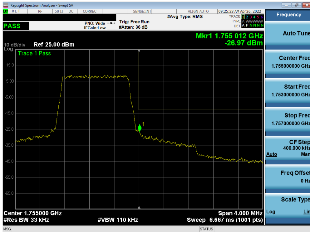
Plot 7-82. Upper Band Edge Plot (LTE Band 4 – 1.4MHz QPSK – Full RB)
