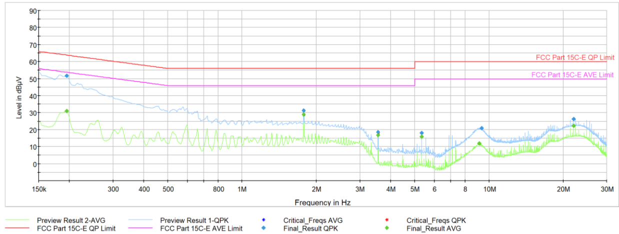
Plot 6-12. AC Line Conducted Plot (N - Mode 1, with Laptop and magnetic charger)
