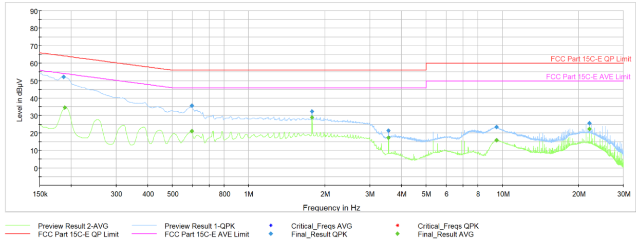
Plot 6-11. AC Line Conducted Plot (L1 - Mode 1, with Laptop and magnetic charger)
