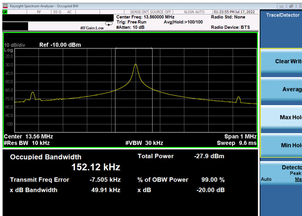
Plot 7-3. 20dB and 99% Bandwidth Plot (CE F 424kbps)
