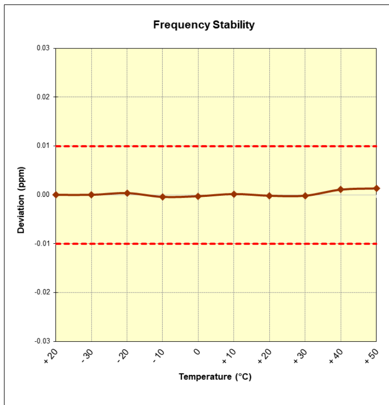
Figure 7-3. Frequency Stability Plot (CE B 106kbps)
