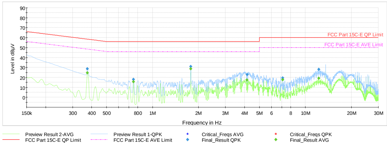
Plot 7-15. AC Line-Conducted Plot (N, Reader A 848kbps, with Laptop and Magnetic Charger)
