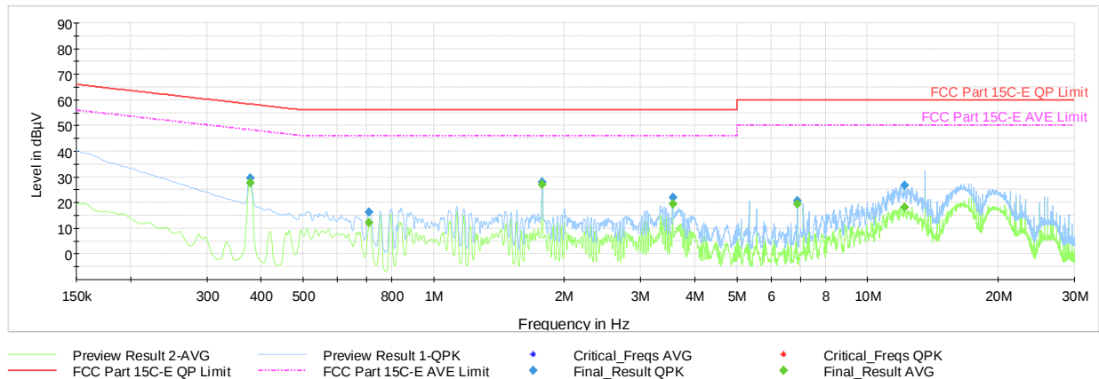
Plot 7-12. AC Line-Conducted Plot (L1, CE B 106kbps, with Laptop and Magnetic Charger)
