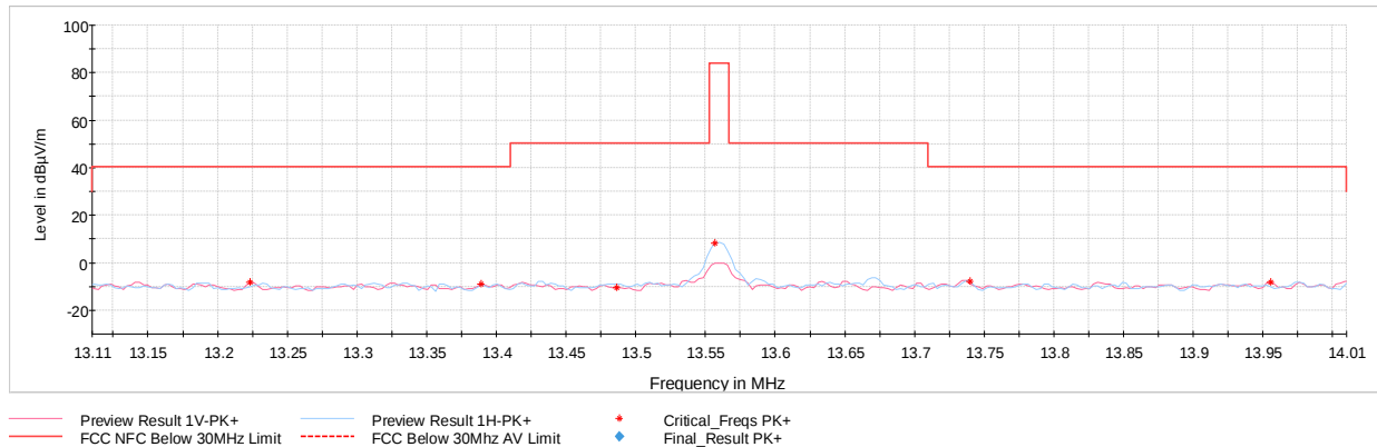
Plot 7-7. In Band Radiated Spurious Emissions (Reader A 848kbps, AC/DC Adapter and Magnetic Charger)
