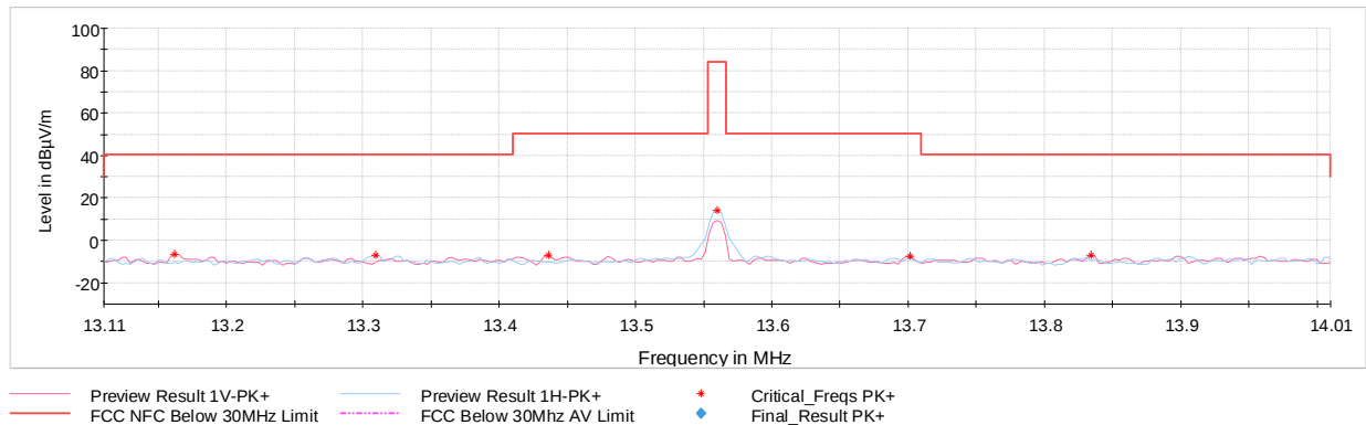
Plot 7-6. In Band Radiated Spurious Emissions (CE B 106kbps, with AC/DC Adapter and Magnetic Charger)
