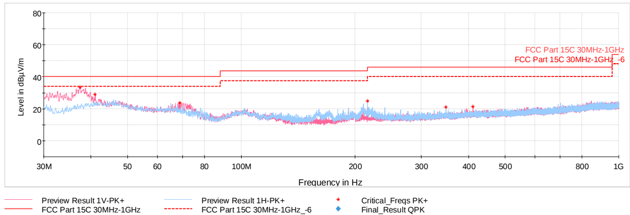
Plot 7-10. Radiated Spurious Emissions 30MHz – 1GHz (CE B 106kbps, with AC/DC Adapter and Magnetic Charger)
