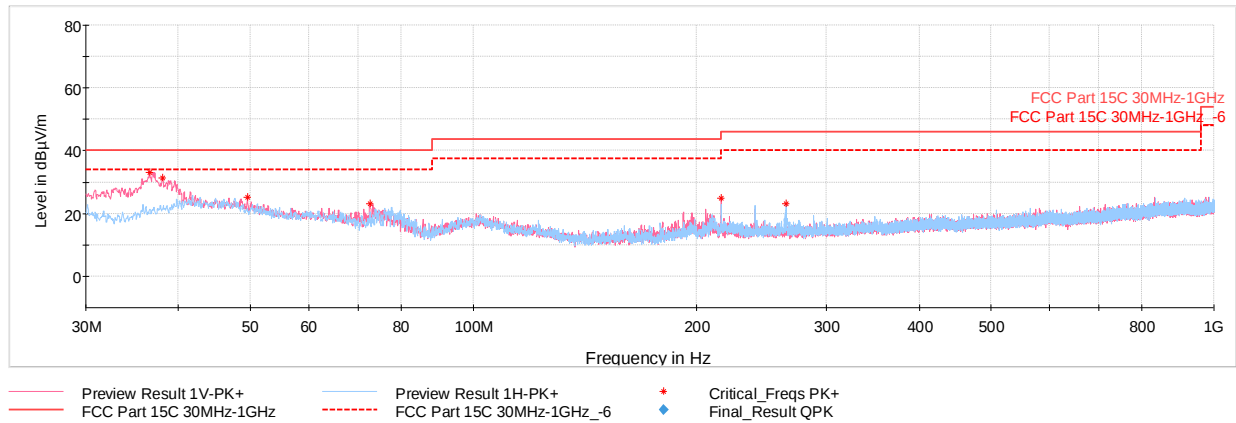
Plot 7-11. Radiated Spurious Emissions 30MHz – 1GHz (Reader A 848kbps, with AC/DC Adapter and Magnetic Charger)
