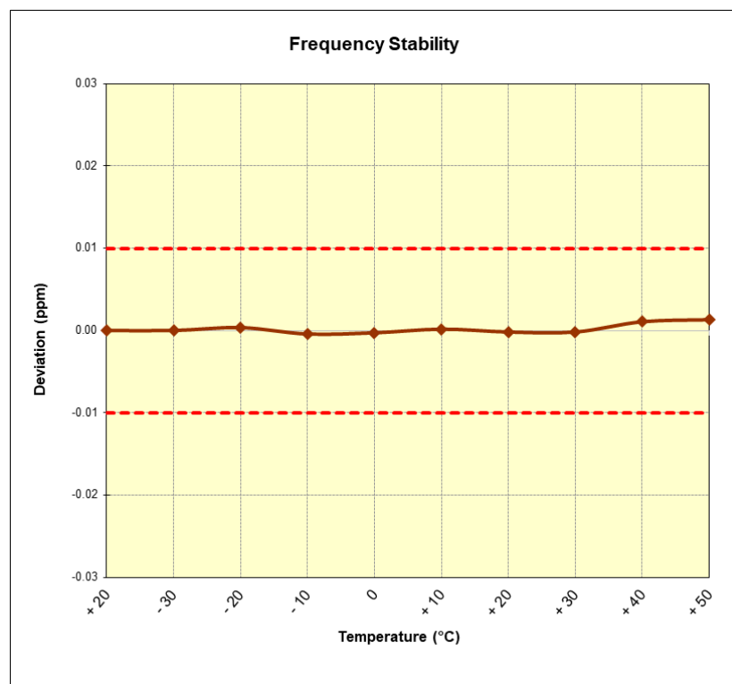
Figure 7-4. Frequency Stability Plot (Reader 100% ASK 1 out of 4)
