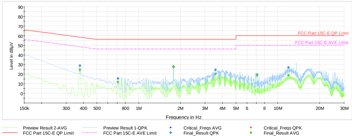
Plot 7-13. AC Line-Conducted Plot (N, CE B 106kbps, with Laptop and Magnetic Charger)
