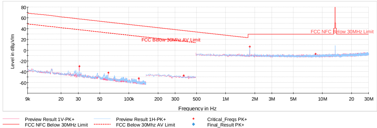
Plot 7-8. Radiated Spurious Emissions 9kHz – 30MHz (CE B 106kbps, with AC/DC Adapter and Magnetic Charger)
