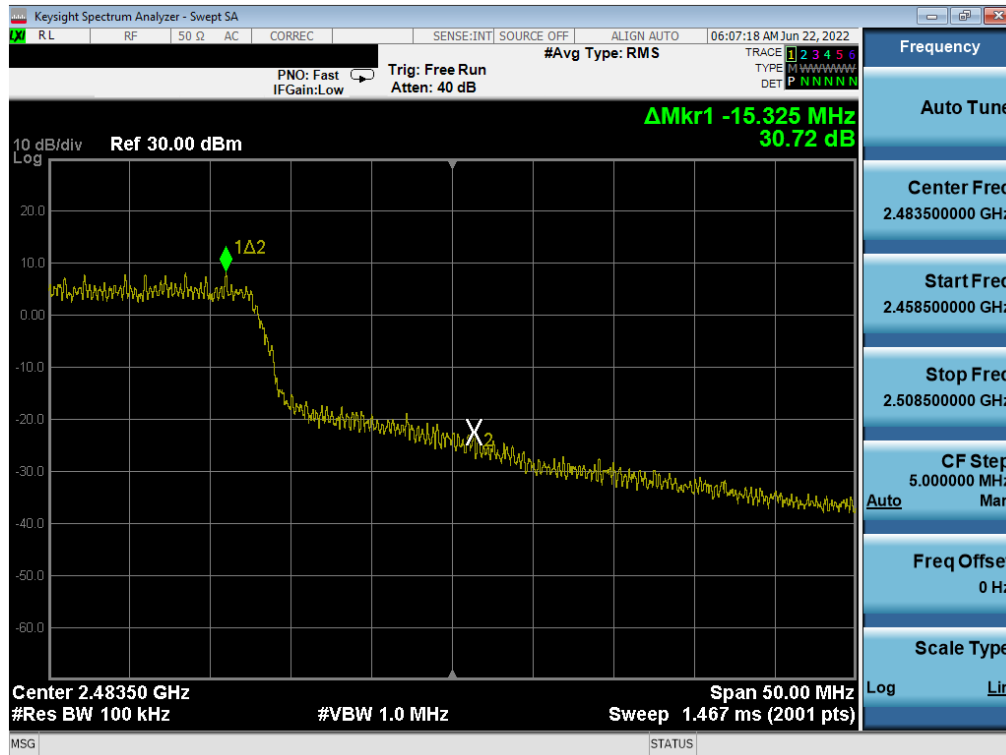
Plot 7-43. Band Edge Plot (802.11n MCS7 – Ch. 11)
