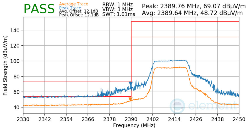
Plot 7-60. Radiated Restricted Lower Band Edge Measurement
