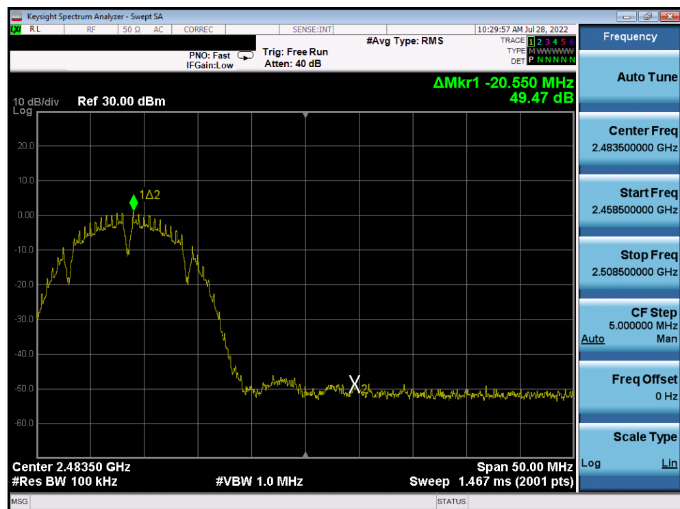
Plot 26. Band Edge Plot (802.11b – Ch. 12)
