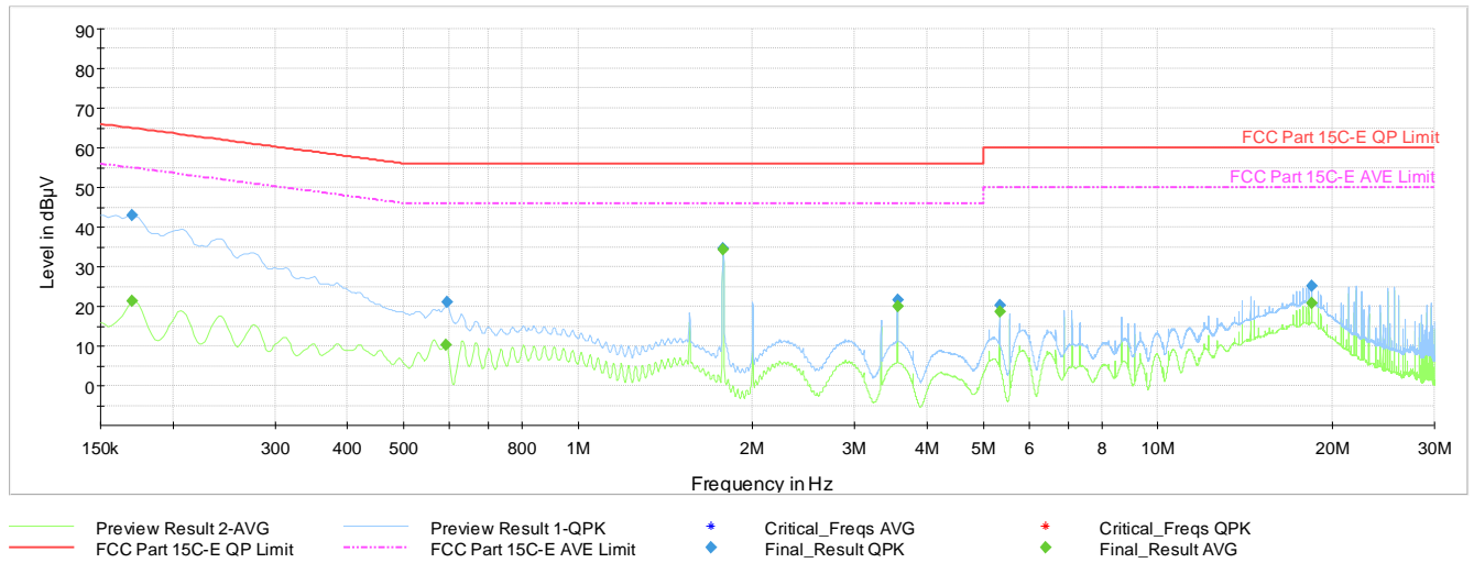
Plot 7-74. AC Line Conducted Plot 802.11b Ch.6 (N), with Laptop
