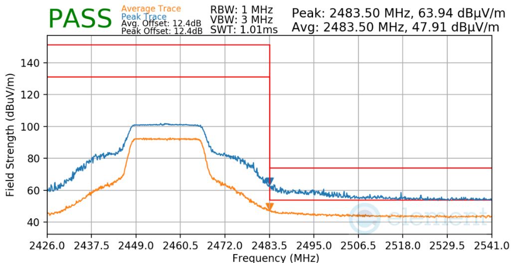
Plot 7-62. Radiated Restricted Upper Band Edge Measurement
