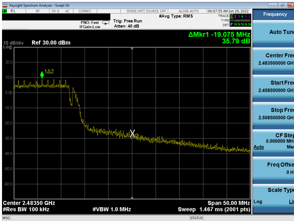
Plot 7-33. Band Edge Plot (802.11g– Ch. 13)
