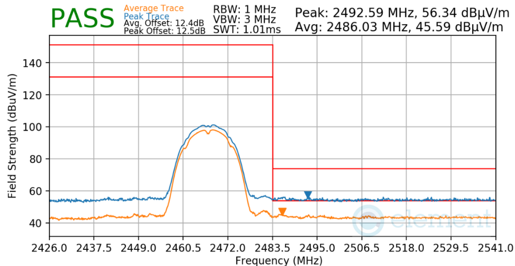
Plot 7-58. Radiated Restricted Upper Band Edge Measurement
