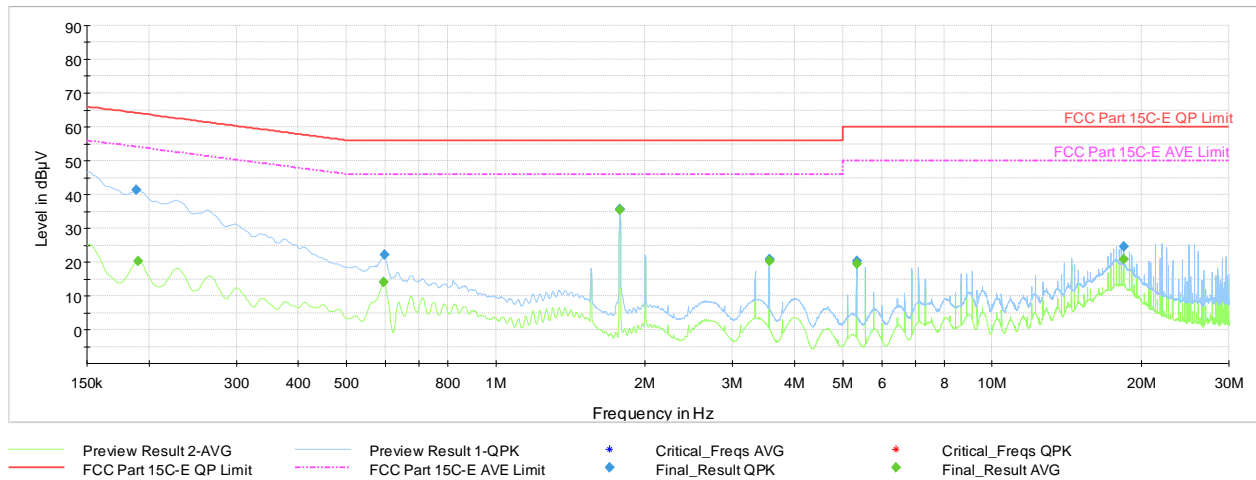
Plot 7-73. AC Line Conducted Plot 802.11b Ch.6 (L1), with Laptop
