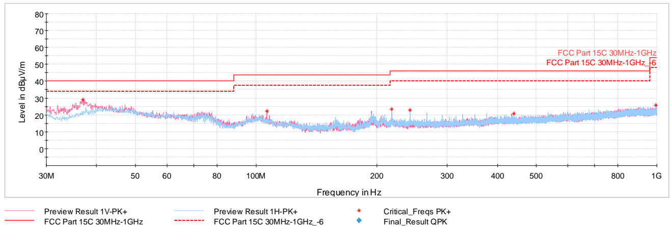
Plot 7-71. Radiated Spurious Emissions 30MHz-1GHz (802.11b – Ch.11, with AC/DC Adapter + Magnetic Charger)
