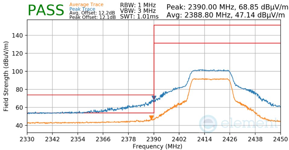
Plot 7-67. Radiated Restricted Lower Band Edge Measurement
