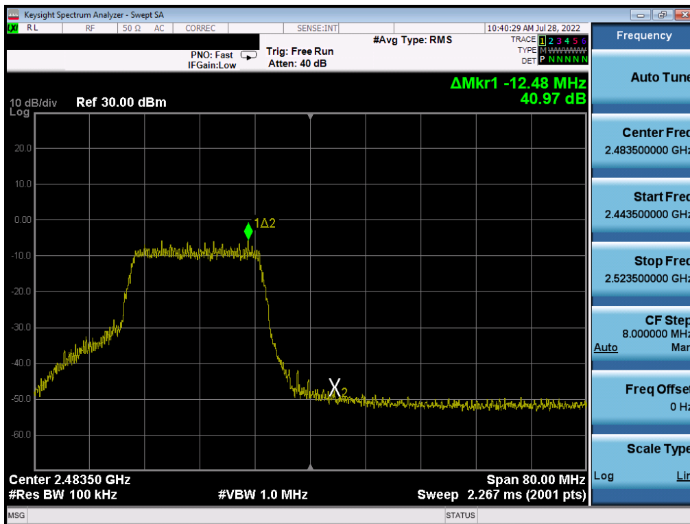
Plot 7-44. Band Edge Plot (802.11n MCS7 – Ch. 12)
