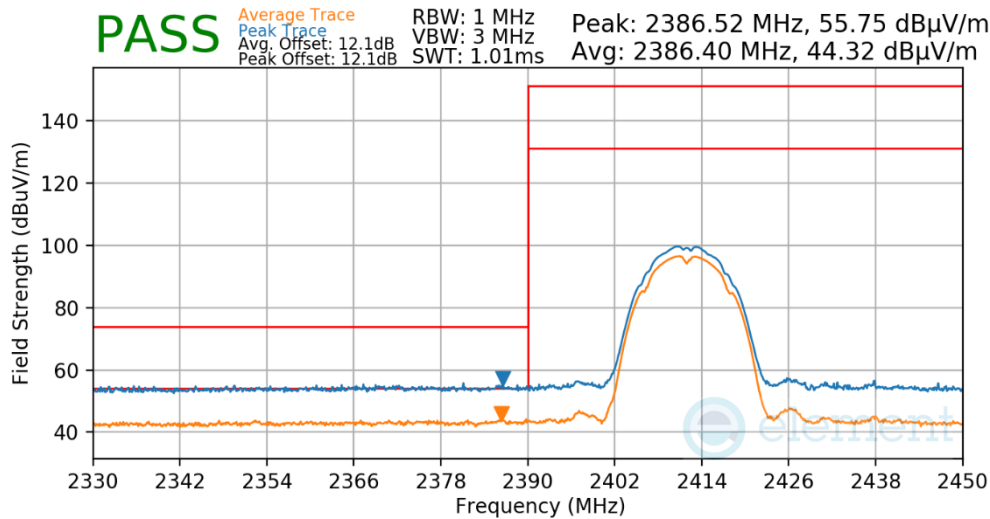
Plot 7-57. Radiated Restricted Lower Band Edge Measurement
