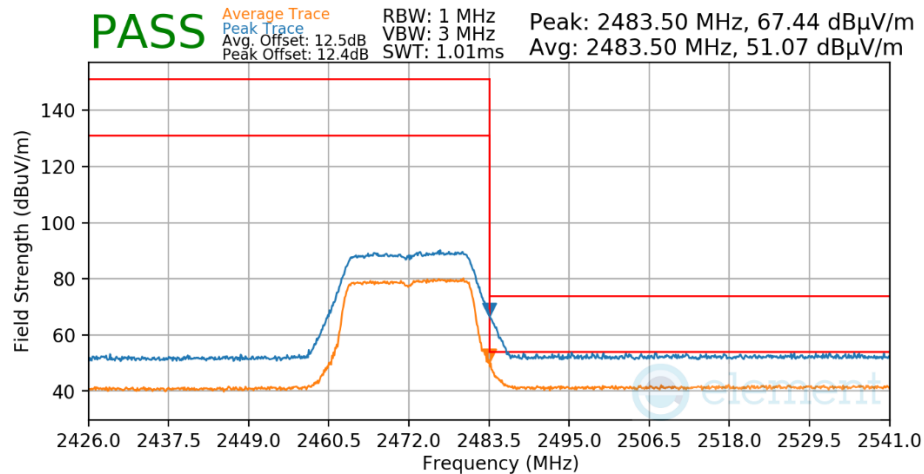
Plot 7-71. Radiated Restricted Upper Band Edge Measurement
