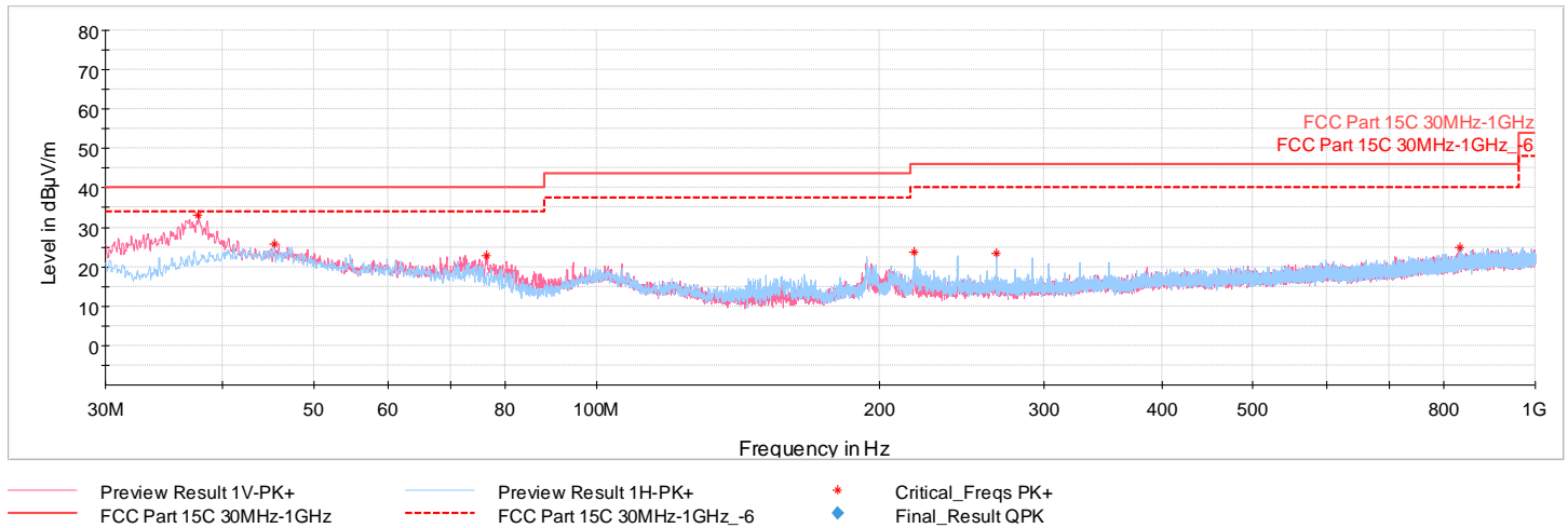
Plot 7-38. Radiated Spurious Plot Below 1GHz 1Mbps, ePA – Ch.39, Pol. H & V, with AC/DC Adapter + Magnetic Charger)
