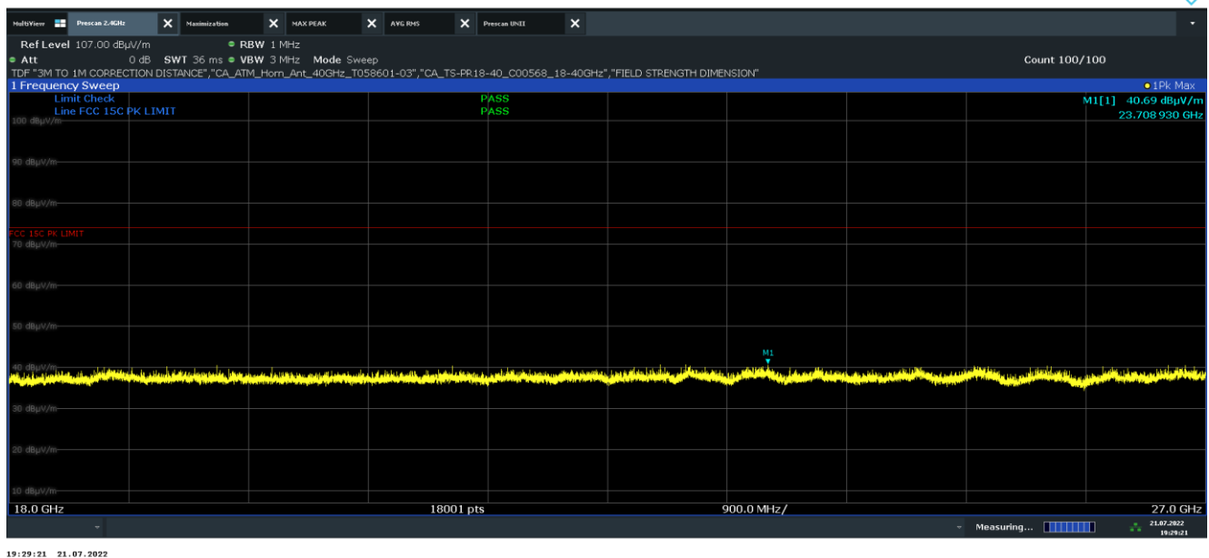
Plot 7-33. Radiated Spurious Plot Above 18GHz (4Mbps, HDR4, ePA – Ch.75, Ant. Pol.V)
