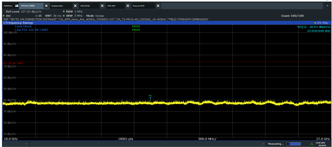
Plot 7-32. Radiated Spurious Plot Above 18GHz (4Mbps, HDR4, ePA – Ch.75, Ant. Pol.H)
