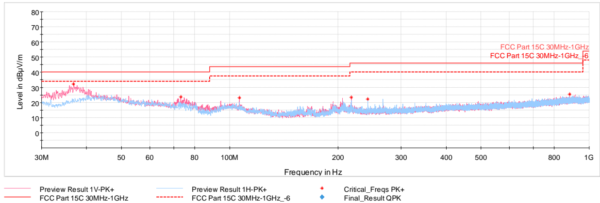
Plot 7-38. Radiated Spurious Emissions Below 1GHz (4Mbps, ePA – Ch.75 with AC/DC Adapter + Magnetic Charger)
