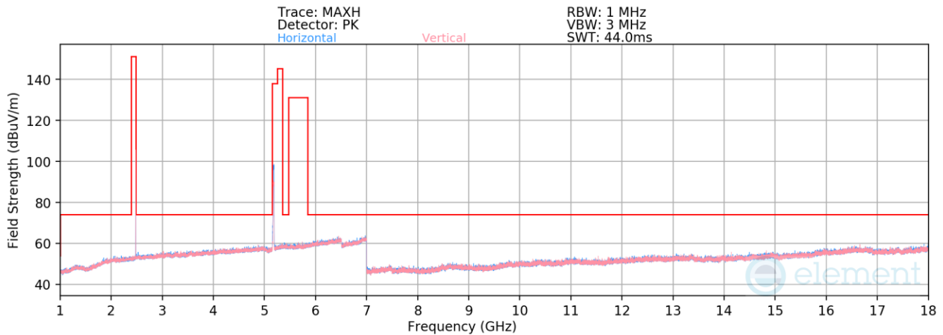
Plot 7-39. Radiated Spurious Emissions above 1-18GHz Simultaneous Tx
