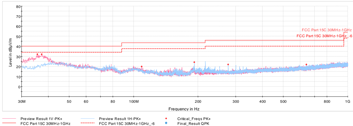
Plot 7-57. Radiated Spurious Emissions – Simultaneous Transmission 30MHz – 1GHz, with AC/DC Adapter & Magnetic Charger
