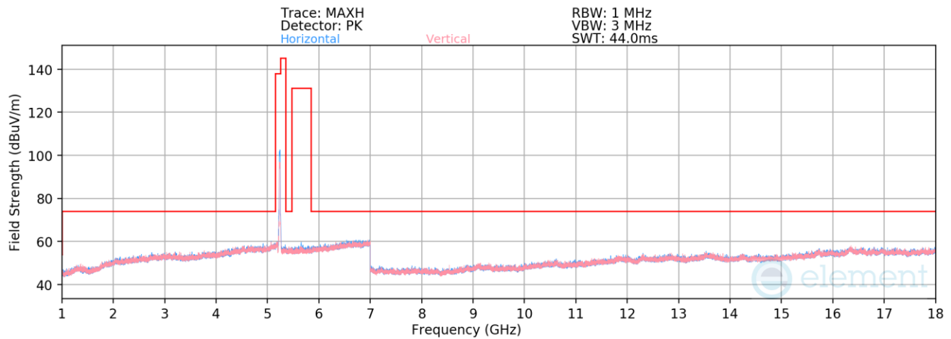
Plot 7-27. Radiated Spurious Emissions above 1GHz (802.11n – Ch. 48)
