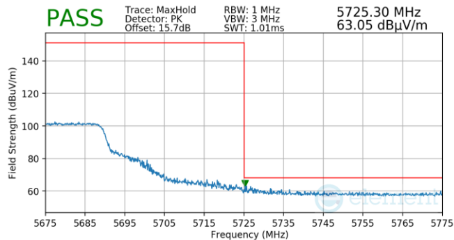
Plot 7-49. FCM (Pk, Ch.136, 802.11n, MCS7)
