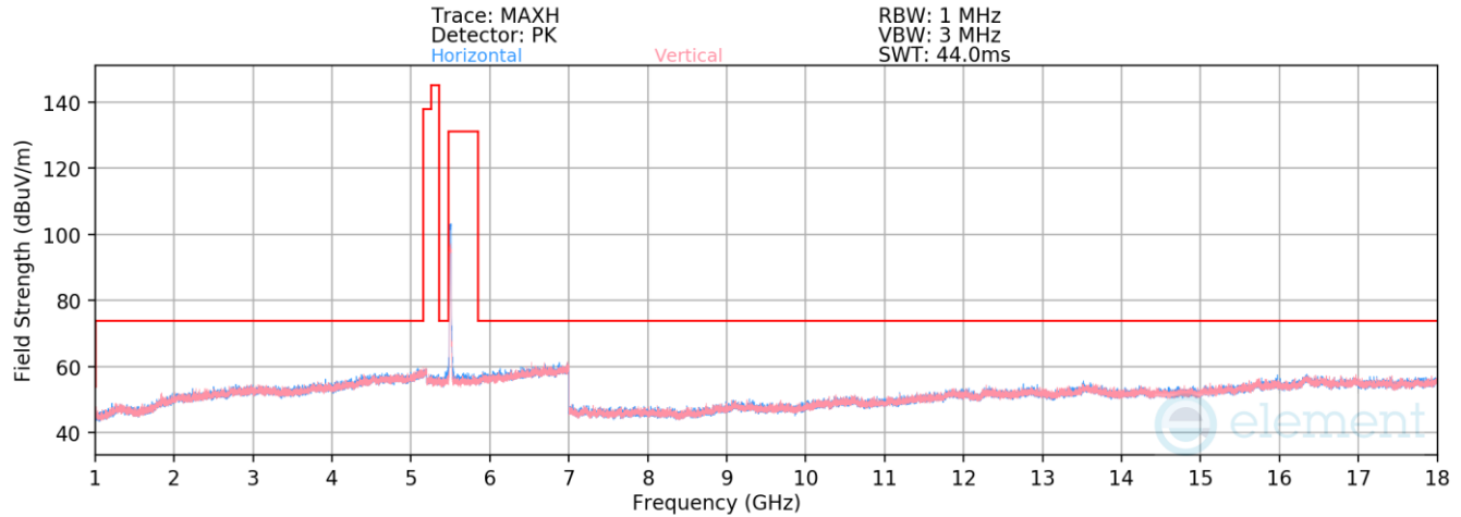
Plot 7-31. Radiated Spurious Emissions above 1GHz (802.11n – Ch. 100)
