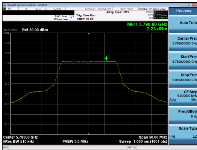
Plot 7-23. PSD (20MHz BW 802.11n – Ch. 157, MCS0)
