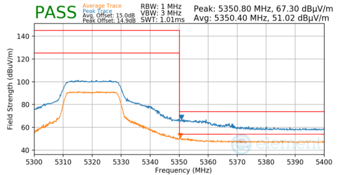
Plot 7-45. FCM (Pk & Avg, Ch.64, 802.11n, MCS7)
