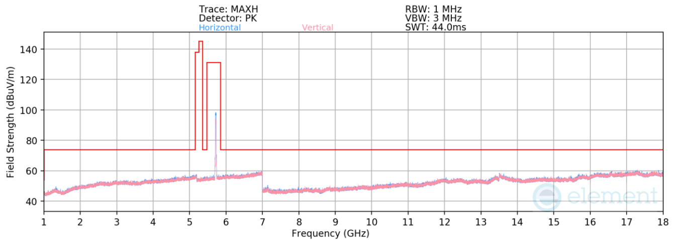
Plot 7-33. Radiated Spurious Emissions above 1GHz (802.11n – Ch. 144)
