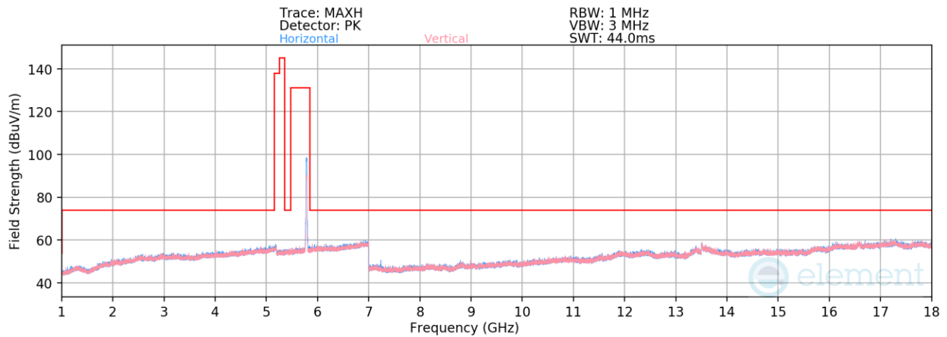
Plot 7-37. Radiated Spurious Emissions above 1GHz (802.11n – Ch. 157)
