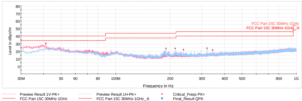
Plot 7-56. Radiated Spurious Emissions below 1GHz 802.11n, Ch.144 with AC/DC Adapter & Magnetic Charger
