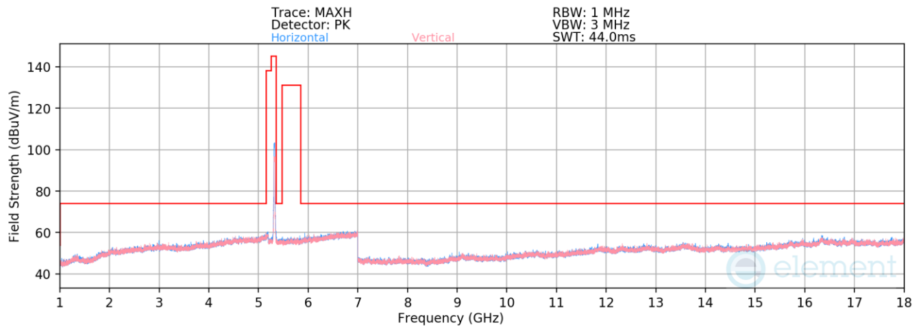
Plot 7-30. Radiated Spurious Emissions above 1GHz (802.11n – Ch. 64)
