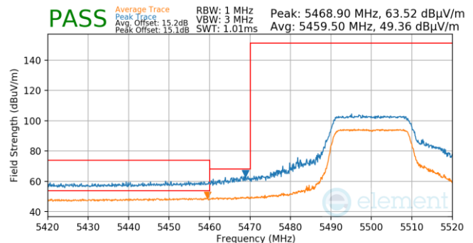
Plot 7-47. FCM (Pk & Avg, Ch.100, 802.11n, MCS7)
