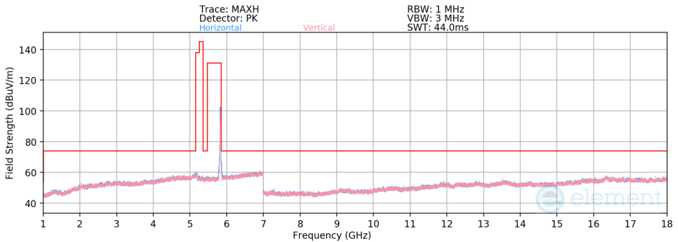
Plot 7-38. Radiated Spurious Emissions above 1GHz (802.11n – Ch. 165)
