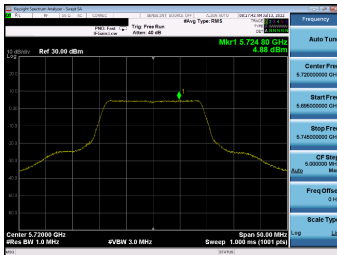
Plot 7-21. PSD (20MHz BW 802.11n - Ch. 144, MCS0)
