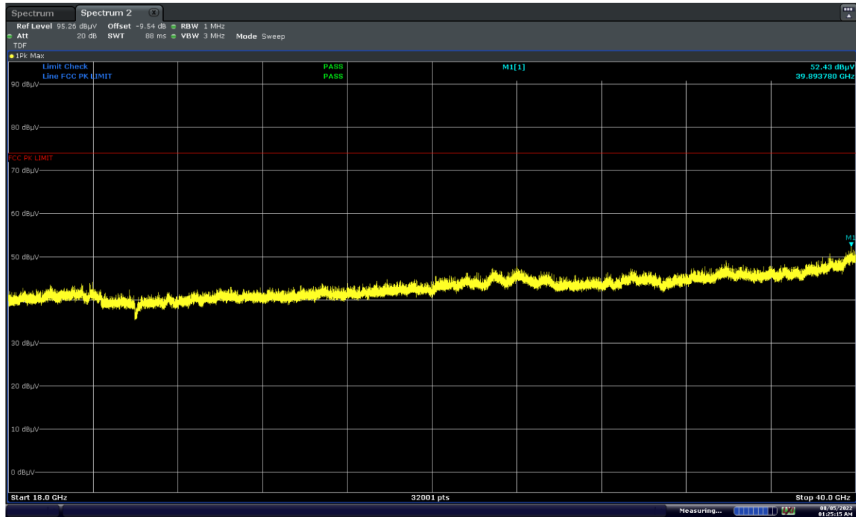
Plot 7-40. Radiated Spurious Emissions – Simultaneous Transmission 18GHz-40GHz Pol H
