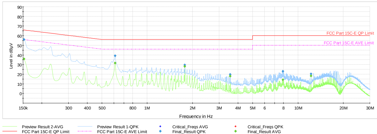
Plot 7-58. AC Line Conducted Plot with 802.11n- Ch.144 (L1) with Laptop & Magnetic Charger
