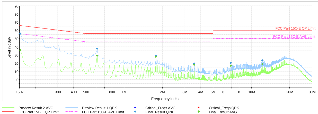
Plot 7-59. AC Line Conducted Plot with 802.11n– Ch.144 (N) with Laptop & Magnetic Charger
