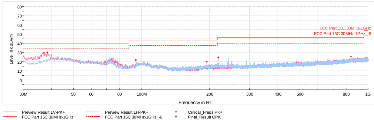
Plot 7-57. Radiated Spurious Emissions – Simultaneous Transmission 30MHz – 1GHz, with AC/DC Adapter)
