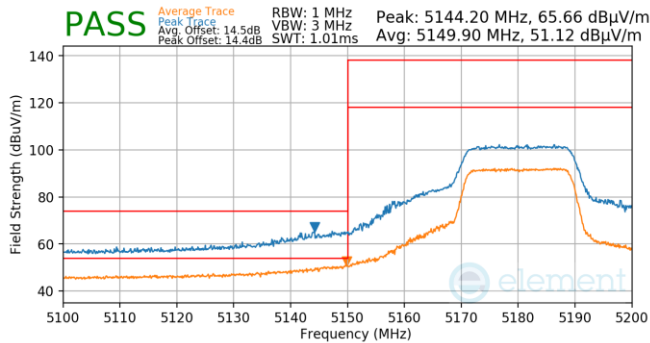
Plot 7-43. FCM (Pk & Avg, Ch.36, 802.11n, MCS7)
