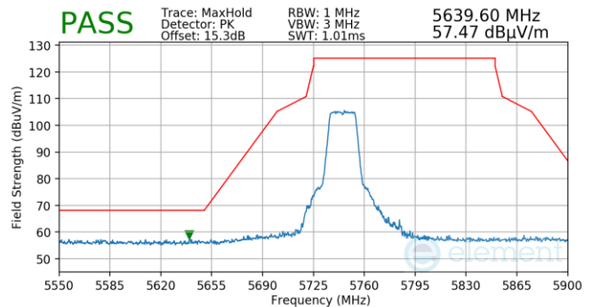
Plot 7-52. FCM (Pk, Ch.149, 802.11n, MCS0)
