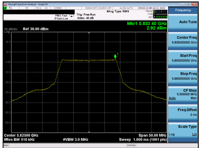
Plot 7-24. PSD (20MHz BW 802.11n – Ch. 165, MCS0)
