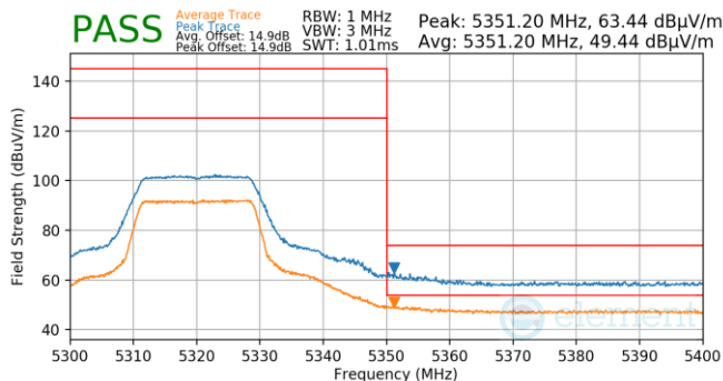
Plot 7-44. FCM (Pk & Avg, Ch.64, 802.11n, MCS0)
