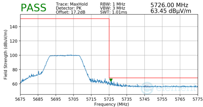
Plot 7-50. FCM (Pk, Ch.140, 802.11n, MCS0)
