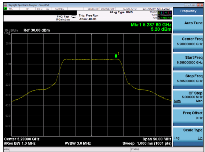
Plot 7-17. PSD (20MHz BW 802.11n - Ch. 56, MCS0)
