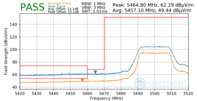
Plot 7-46. FCM (Pk & Avg, Ch.100, 802.11n, MCS0)
