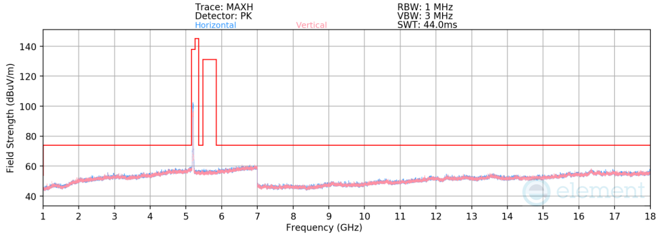
Plot 7-26. Radiated Spurious Emissions above 1GHz (802.11n – Ch. 40)
