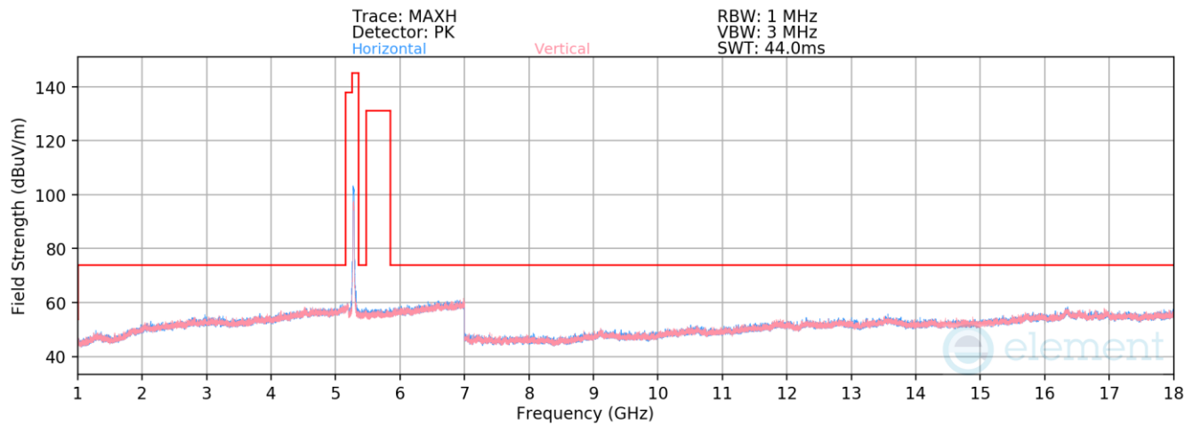
Plot 7-29. Radiated Spurious Emissions above 1GHz (802.11n – Ch. 56)
