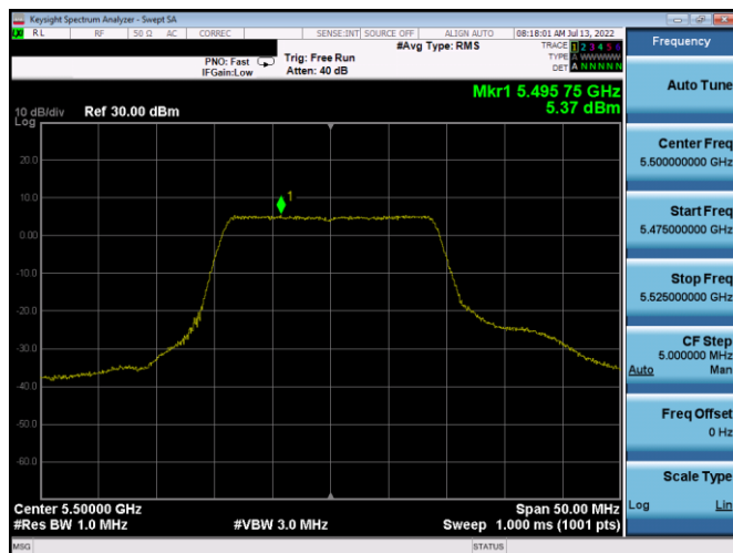
Plot 7-19. PSD (20MHz BW 802.11n - Ch. 100, MCS0)
