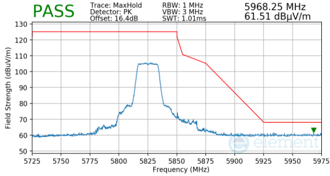
Plot 7-54. FCM (Pk, Ch.165, 802.11n, MCS0)
