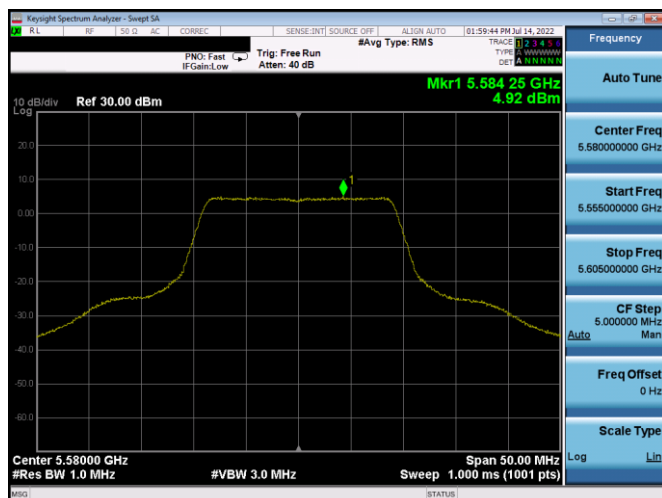
Plot 7-20. PSD (20MHz BW 802.11n - Ch. 116, MCS0)
