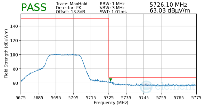
Plot 7-51. FCM (Pk, Ch.140, 802.11n, MCS7)
