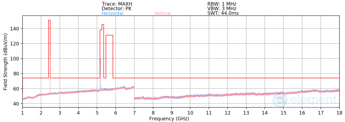
Plot 7-39. Radiated Spurious Emissions 1-18GHz Simultaneous Tx
