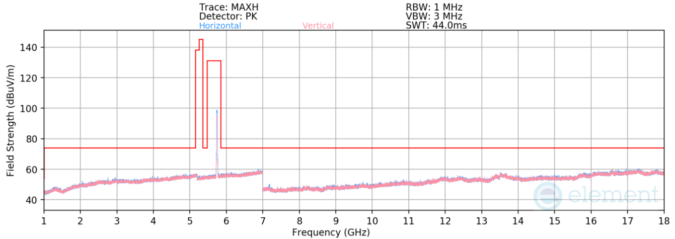
Plot 7-36. Radiated Spurious Emissions above 1GHz (802.11n – Ch. 149)
