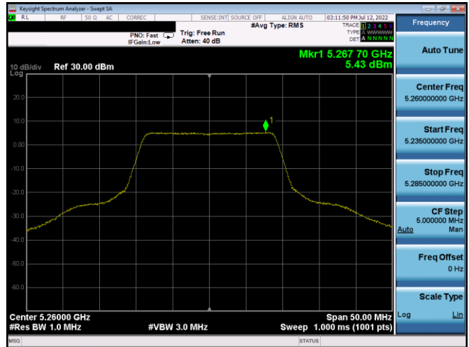
Plot 7-16. PSD (20MHz BW 802.11n - Ch. 52, MCS0)
