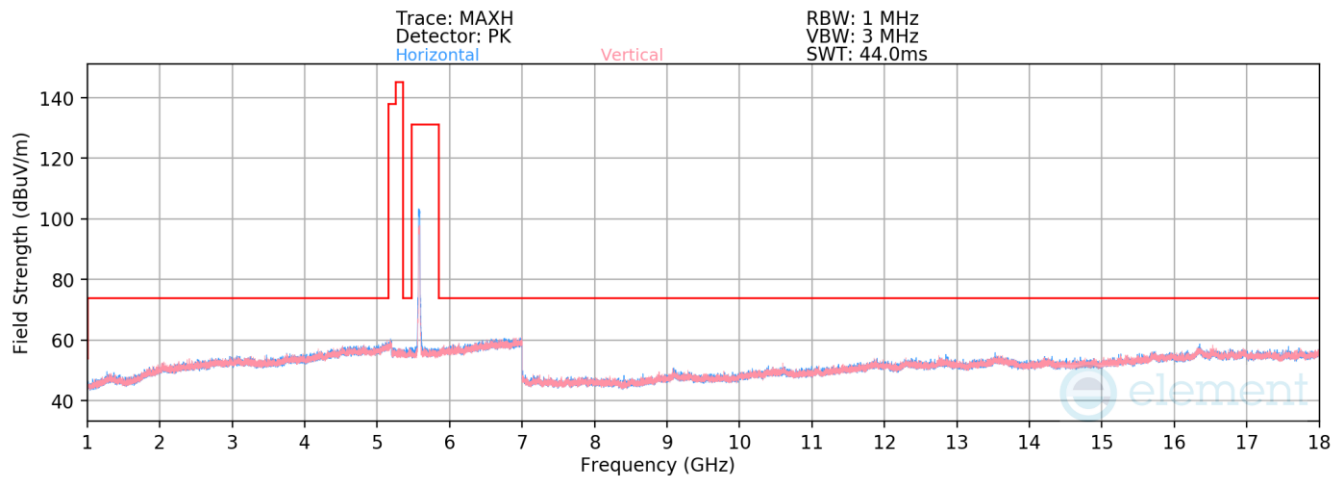
Plot 7-32. Radiated Spurious Emissions above 1GHz (802.11n – Ch. 116)
