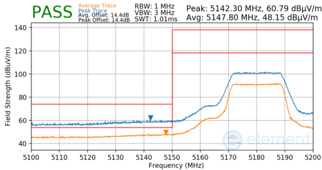
Plot 7-42. FCM (Pk & Avg, Ch.36, 802.11n, MCS0)
