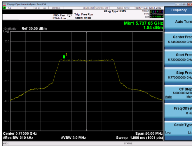
Plot 7-22. PSD (20MHz BW 802.11n – Ch. 149, MCS0)
