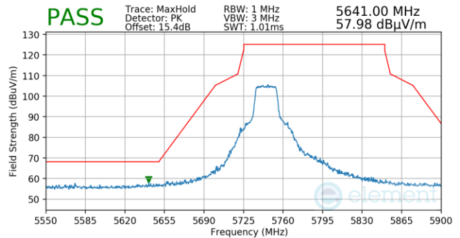
Plot 7-53. FCM (Pk, Ch.149, 802.11n, MCS7)
