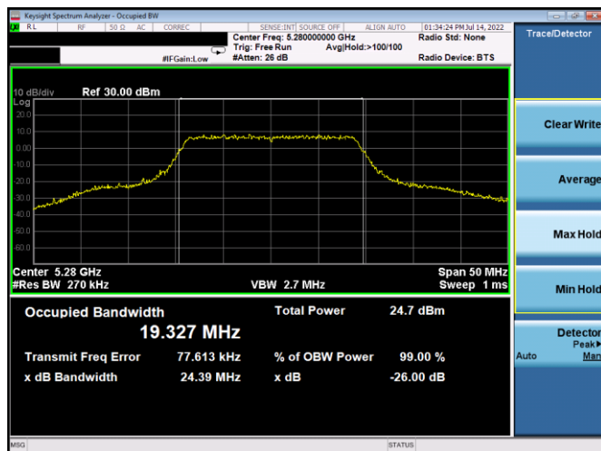
Plot 7-5. 26dB BW & 99% OBW (20MHz BW 802.11n – Ch. 56, MCS0)
