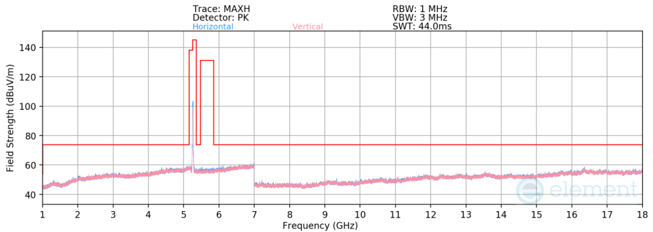
Plot 7-28. Radiated Spurious Emissions above 1GHz (802.11n – Ch. 52)
