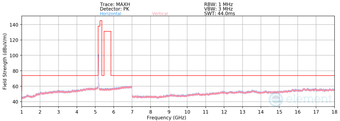
Plot 7-25. Radiated Spurious Emissions above 1GHz (802.11n – Ch. 36)
