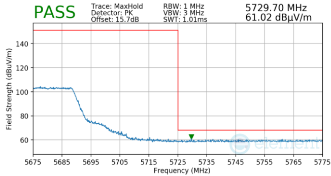
Plot 7-48. FCM (Pk, Ch.136, 802.11n, MCS0)
