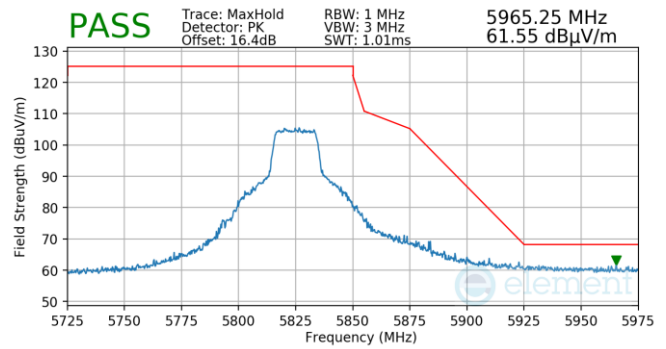
Plot 7-55. FCM (Pk, Ch.165, 802.11n, MCS7)
