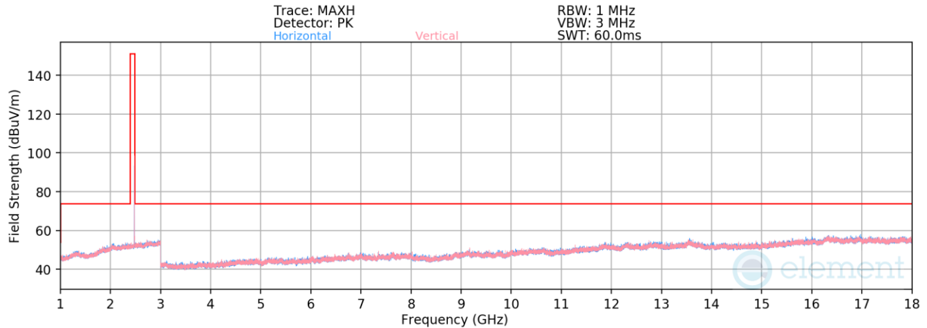
Plot 7-33. Radiated Spurious Emissions 1-18GHz (4Mbps, HDR4, ePA – Ch. 75)
