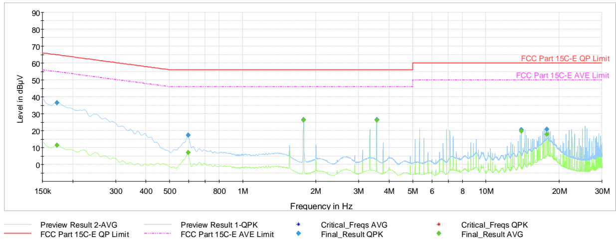
Plot 7-39. AC Line Conducted Plot with Bluetooth HDR (L1, 4Mbps ePA - Ch.38 with Laptop + Magnetic Charger)
