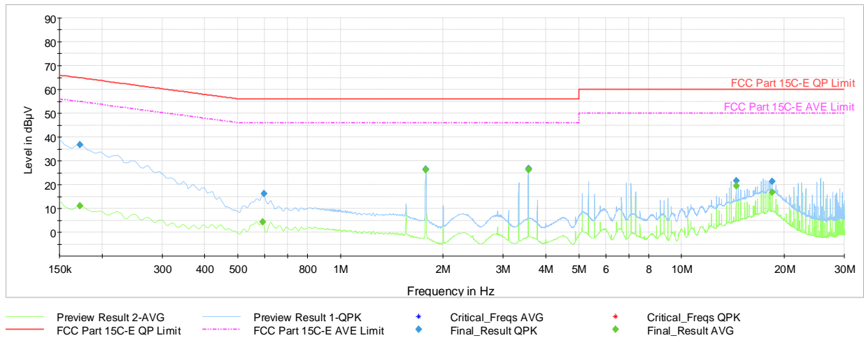
Plot 7-40. AC Line Conducted Plot with Bluetooth HDR (N, 4Mbps ePA - Ch.38 with Laptop + Magnetic Charger)
