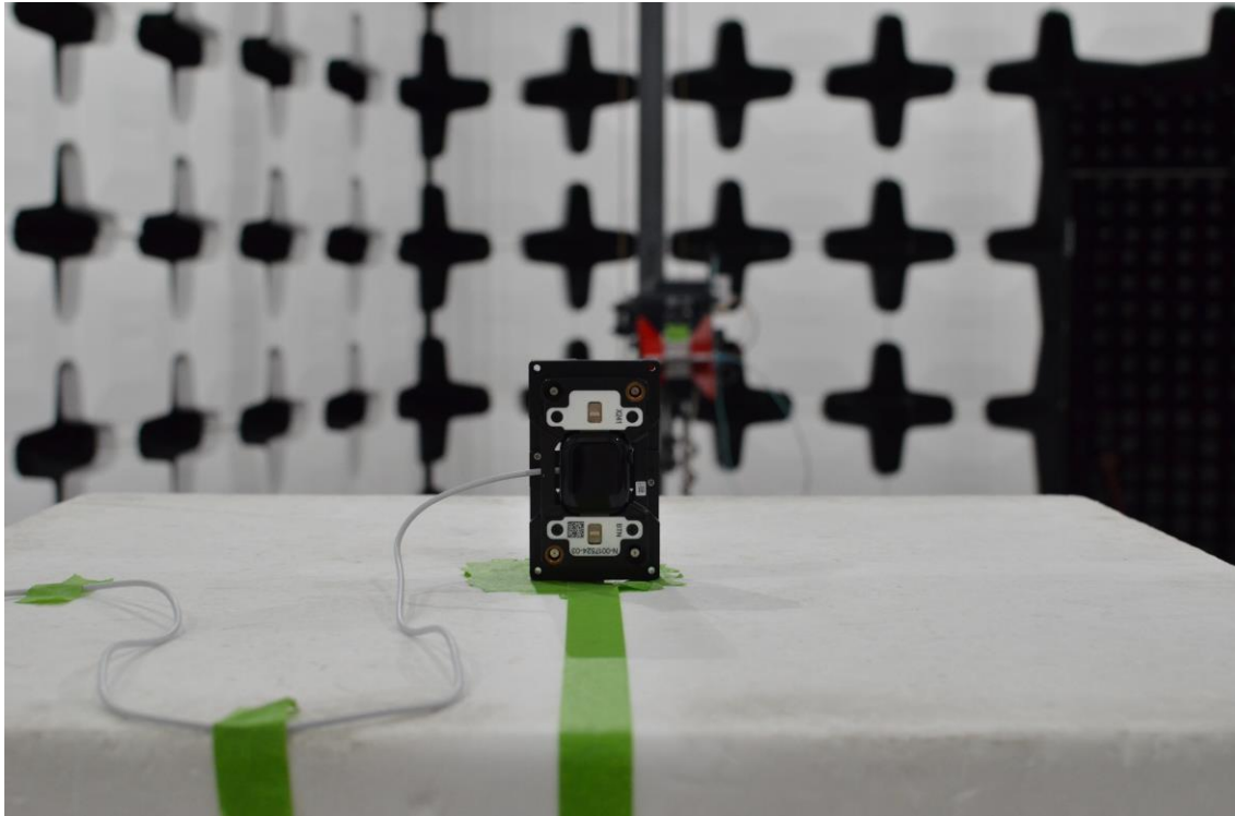
Figure 11: 1-18GHz Test Setup (Rear View)
