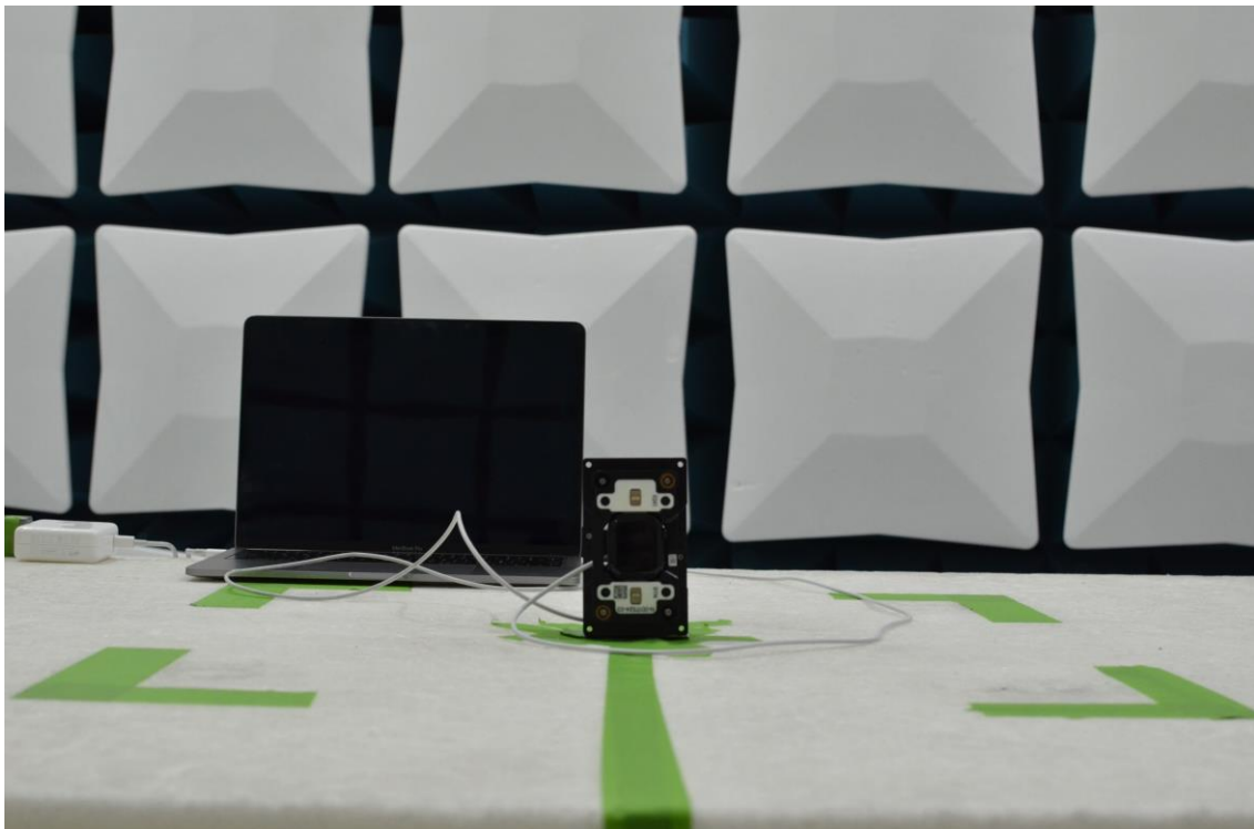
Figure 16: 30MHz-1GHz Test Setup (Front View)
