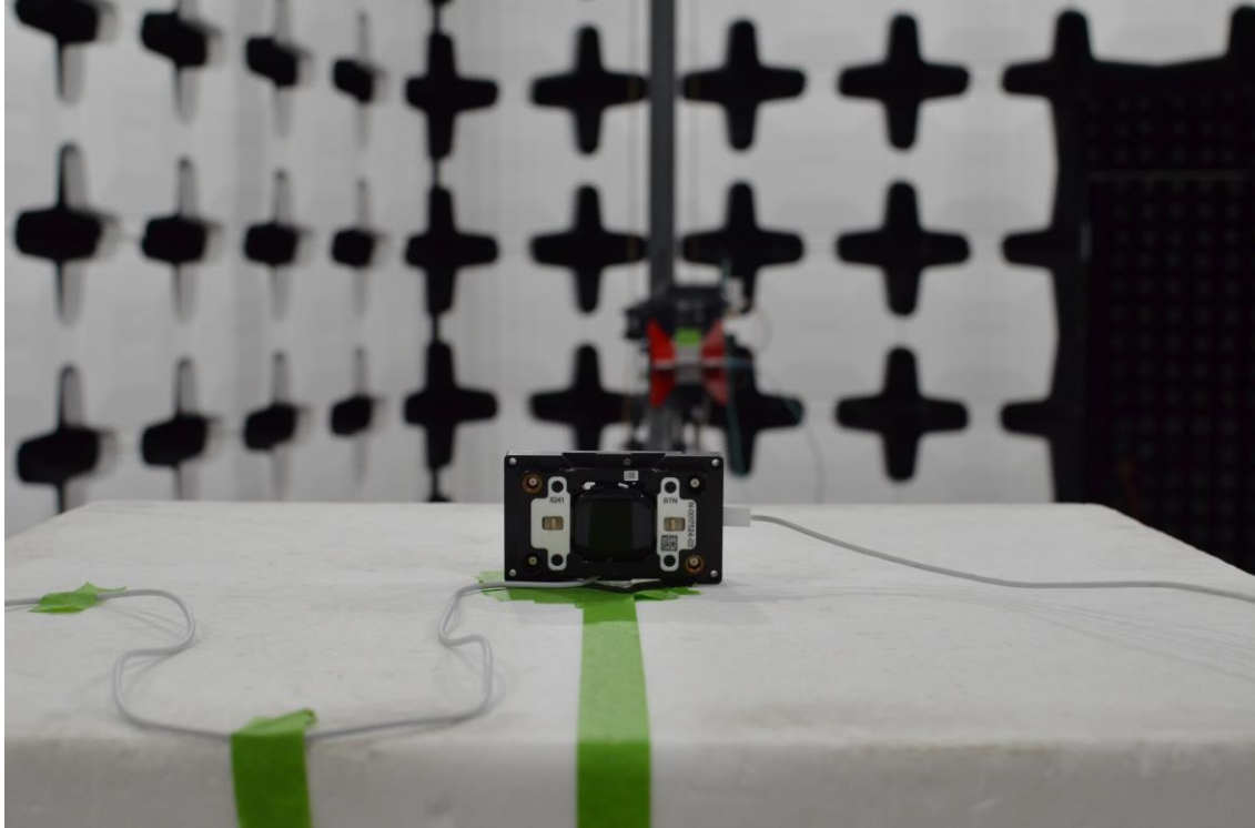
Figure 9: 1-18GHz Test Setup (Rear View)
