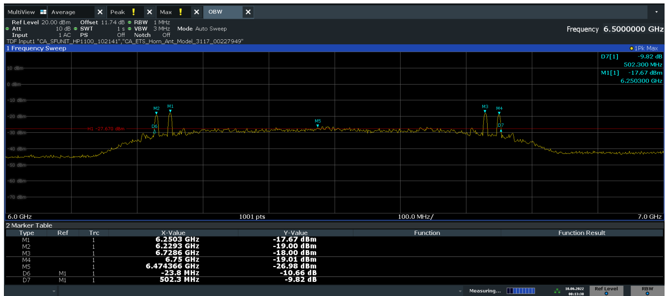
Plot 7-1. 10dBc Bandwidth (Ch. 5, Config 0/Payload 125)
