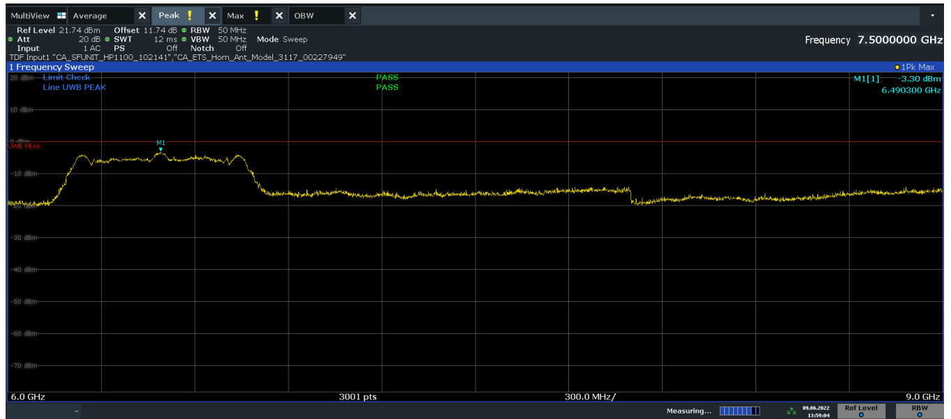
Plot 7-5. Peak Radiated Power (Ch. 5, Config 0/Payload 125)
