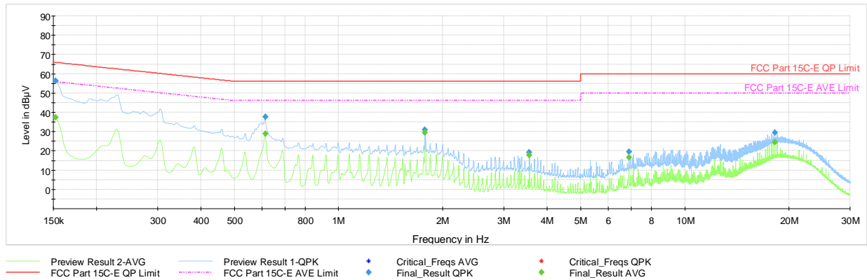
Plot 7-44. AC Line Conducted Plot (Ch. 9, Config 0, Payload 125 N, with PC via USB-C cable with magnetic charger)
