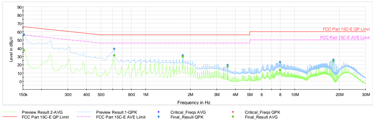
Plot 7-43. AC Line Conducted (Ch. 9, Config 0, Payload 125 L1, with PC via USB-C cable with magnetic charger)
