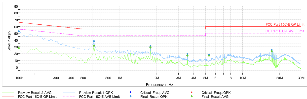
Plot 7-41. AC Line Conducted (Ch. 5, Config 0, Payload 125 L1, with PC via USB-C cable with magnetic charger)
