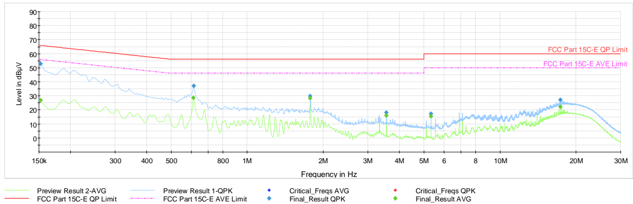
Plot 7-42. AC Line Conducted (Ch. 5, Config 0, Payload 125 N, with PC via USB-C cable with magnetic charger)
