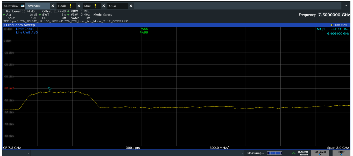
Plot 7-7. Average Radiated Power (Ch. 5, Config 0/Payload 125)
