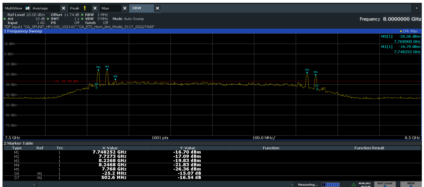
Plot 7-2. 10dBc Bandwidth (Ch. 9, Config 0/Payload 125)
