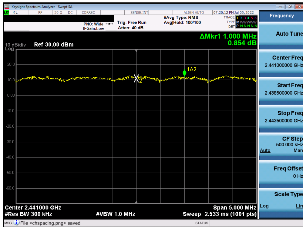
Plot 7-16. Channel Spacing Plot (Bluetooth, 8DPSK, ePA)
