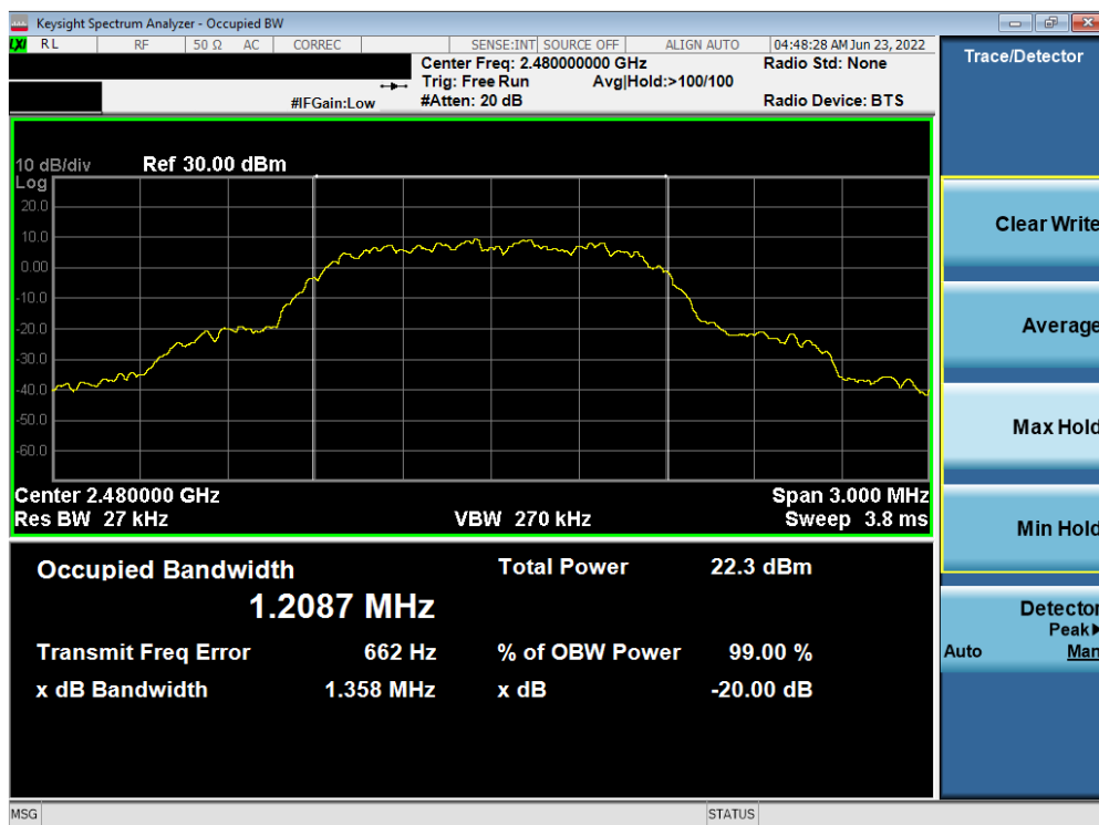
Plot 7-6. Conducted 20dB BW and 99% OBW Plot (Bluetooth, 8DPSK, ePA – Ch. 78)
