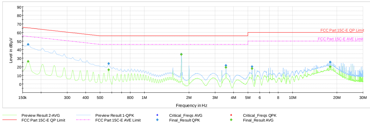
Plot 7-43. AC Line-Conducted Test Plot (N, GFSK ePA – Ch.78, with Laptop & Magnetic Charger)
