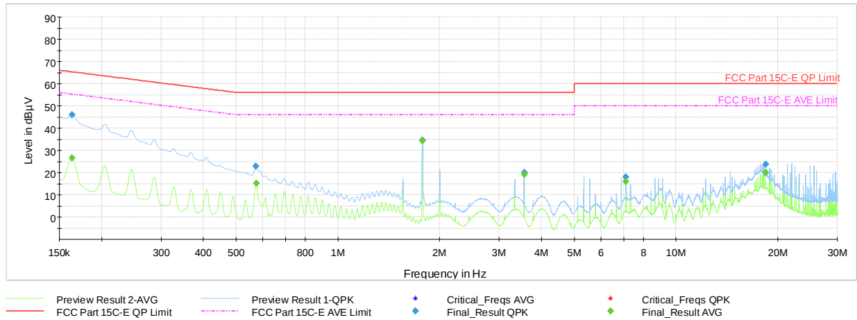
Plot 7-42. AC Line-Conducted Test Plot (L1, GFSK ePA – Ch.78, with Laptop & Magnetic Charger)
