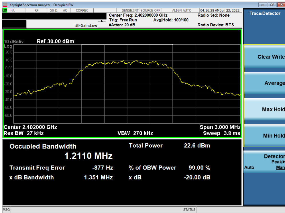
Plot 7-4. Conducted 20dB BW and 99% OBW Plot (Bluetooth, 8DPSK, ePA – Ch. 0)
