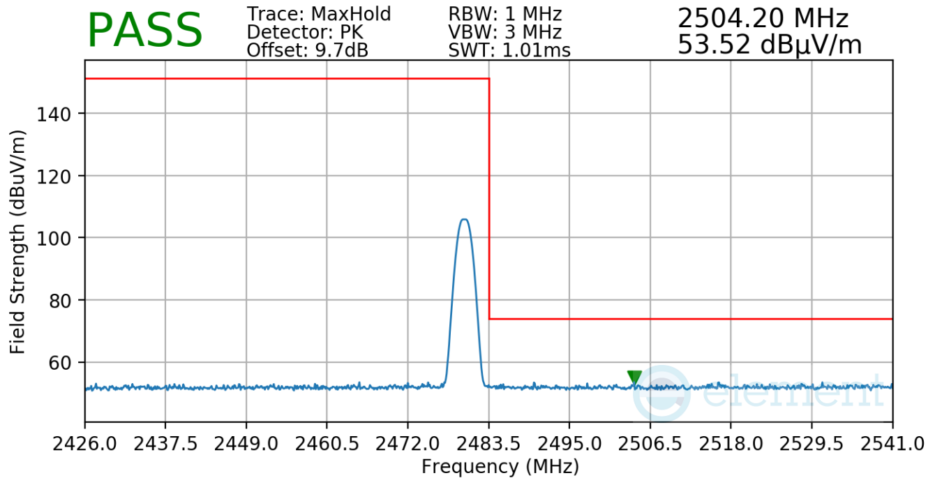
Plot 7-39. Radiated Restricted Upper Band Edge Measurement
