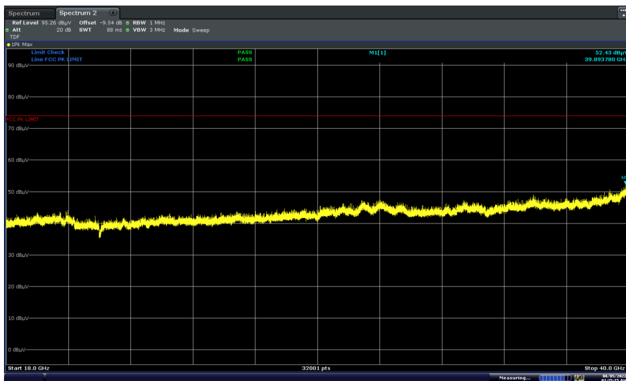
Plot 7-36. Radiated Spurious Emissions above 18GHz – Simultaneous Transmission (Pol. V)
