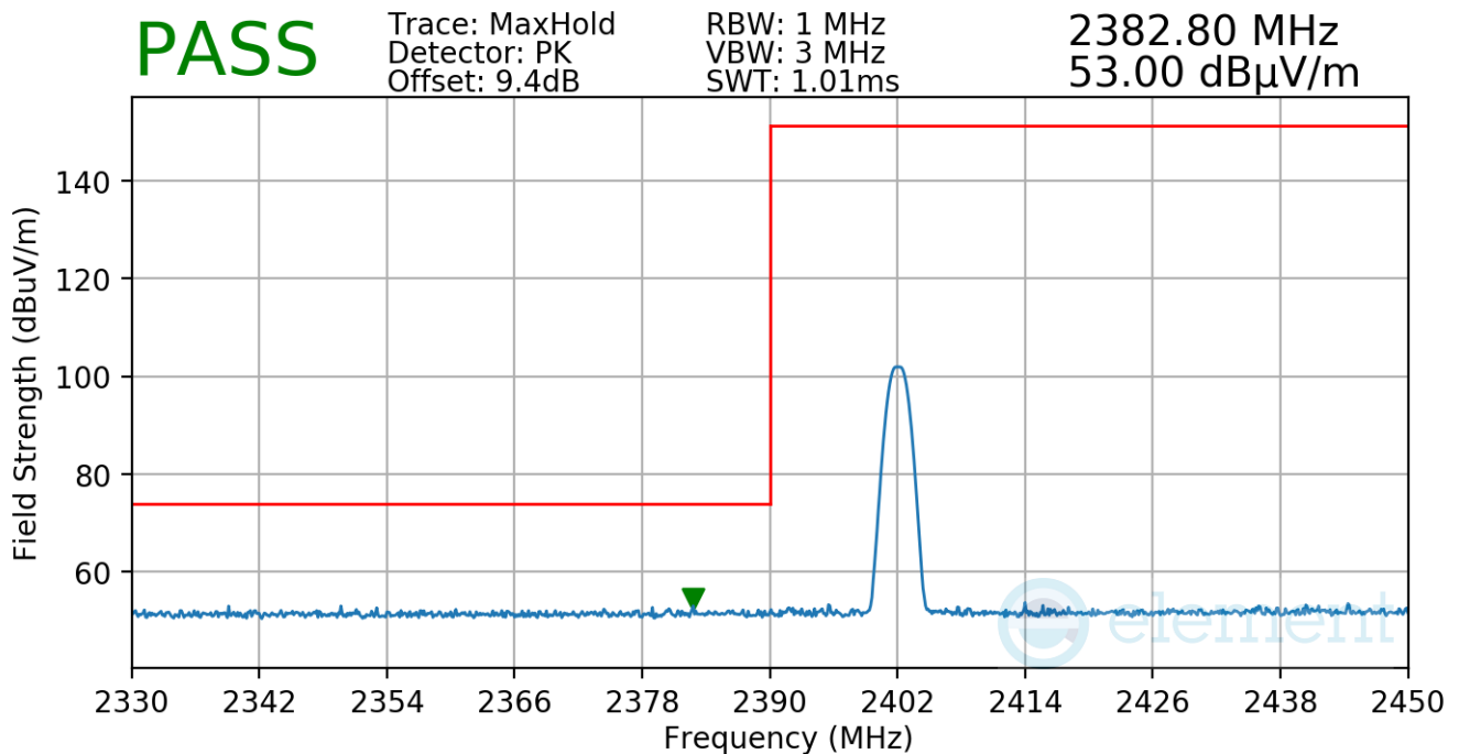
Plot 7-37. Radiated Restricted Lower Band Edge Measurement
