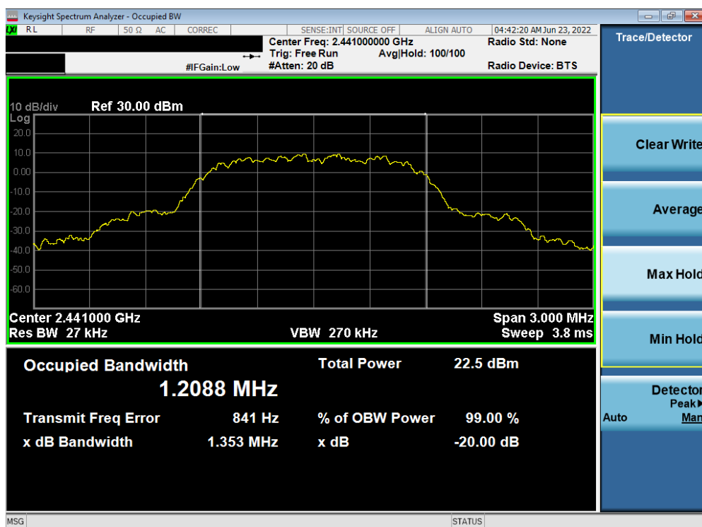
Plot 7-5. Conducted 20dB BW and 99% OBW Plot (Bluetooth, 8DPSK, ePA – Ch. 39)
