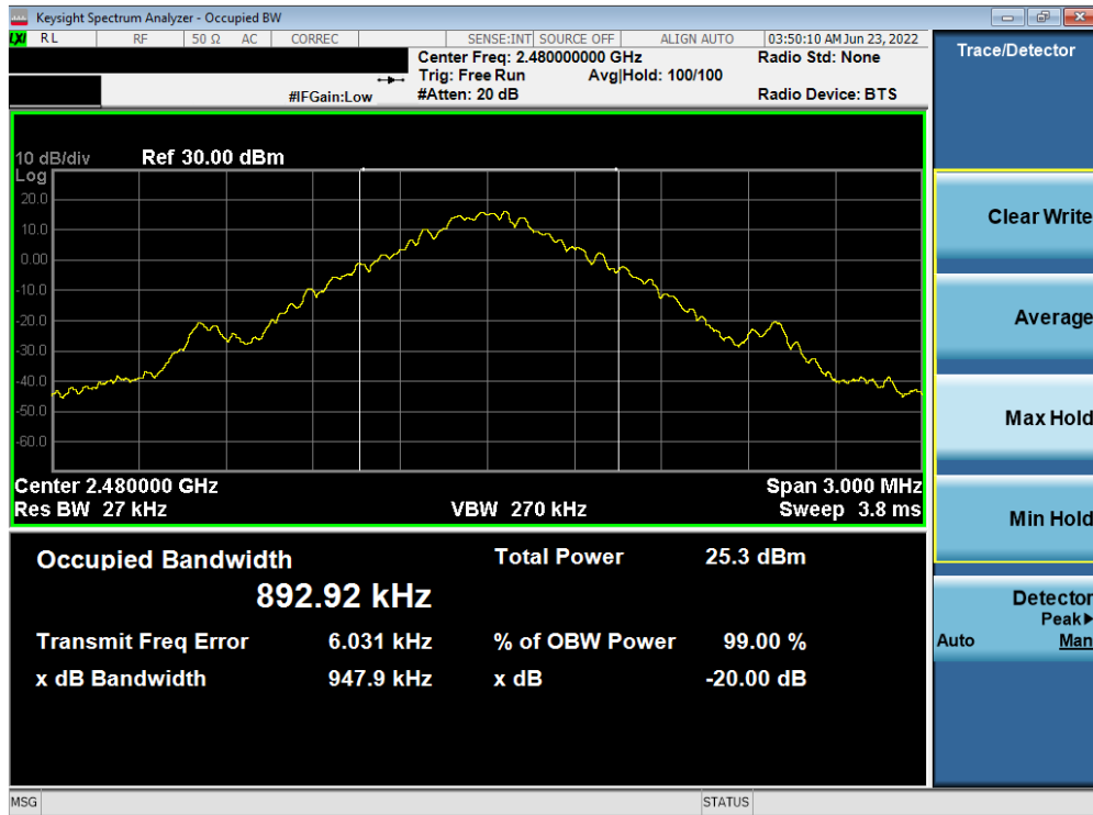
Plot 7-3. Conducted 20dB BW and 99% OBW Plot (Bluetooth, GFSK, ePA – Ch. 78)
