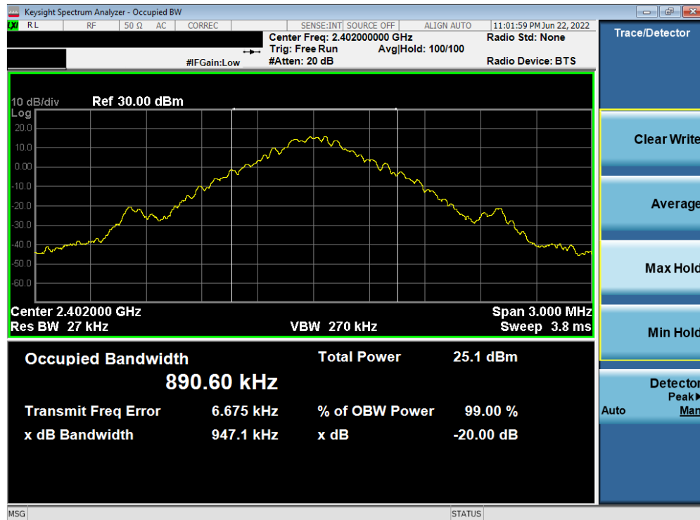
Plot 7-1. Conducted 20dB BW and 99% OBW Plot (Bluetooth, GFSK, ePA – Ch. 0)
