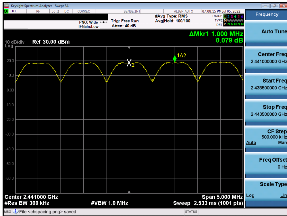
Plot 7-15. Channel Spacing Plot (Bluetooth, GFSK, ePA)
