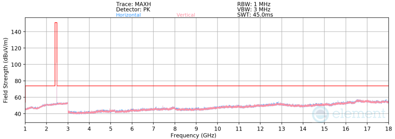
Plot 7-31. Radiated Spurious Emissions above 1GHz (BT GFSK ePA – Ch. 78)
