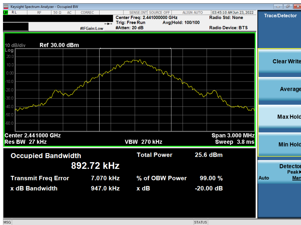
Plot 7-2. Conducted 20dB BW and 99% OBW Plot (Bluetooth, GFSK, ePA – Ch. 39)
