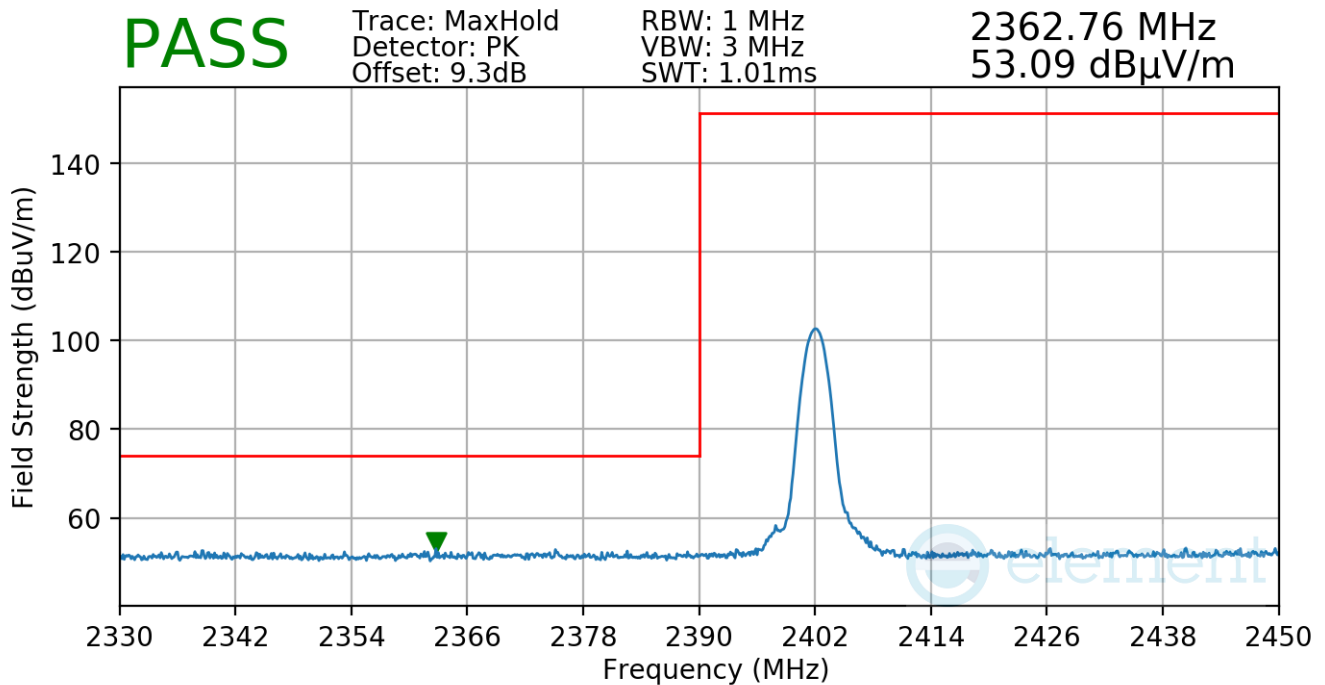
Plot 7-38. Radiated Restricted Lower Band Edge Measurement
