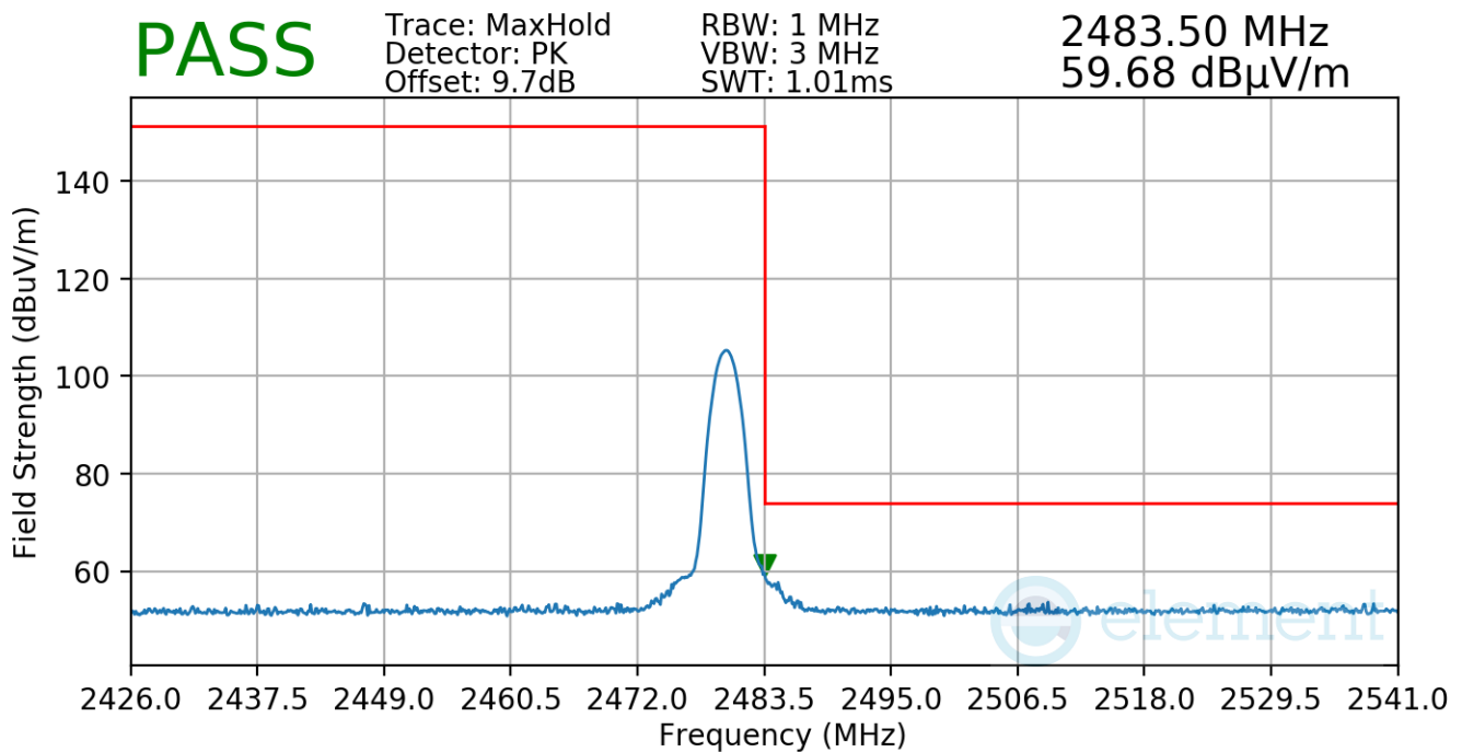
Plot 7-40. Radiated Restricted Upper Band Edge Measurement
