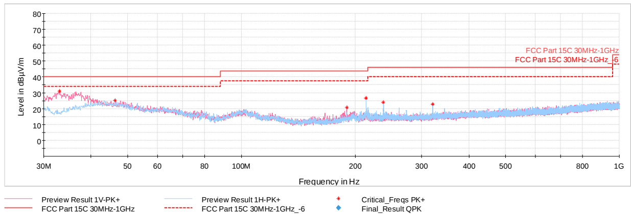
Plot 7-41. Radiated Spurious Plot Below 1GHz (GFSK ePA – Ch.78, Pol. H & V, with AC/DC Adapter & Magnetic Charger)
