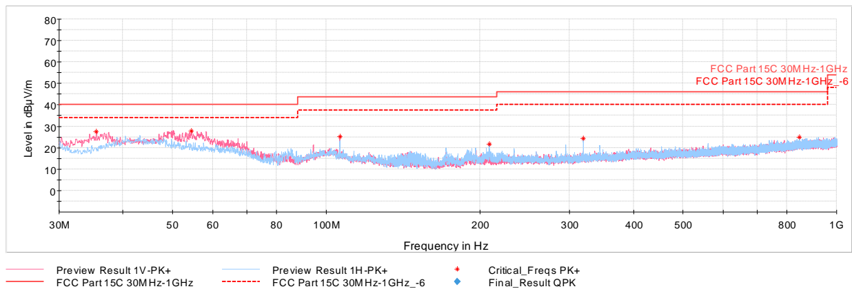
Plot 7-74. Radiated Spurious Emissions below 1GHz (802.11b – Ch.6, with AC/DC Adaptor and Magnetic Charger)
