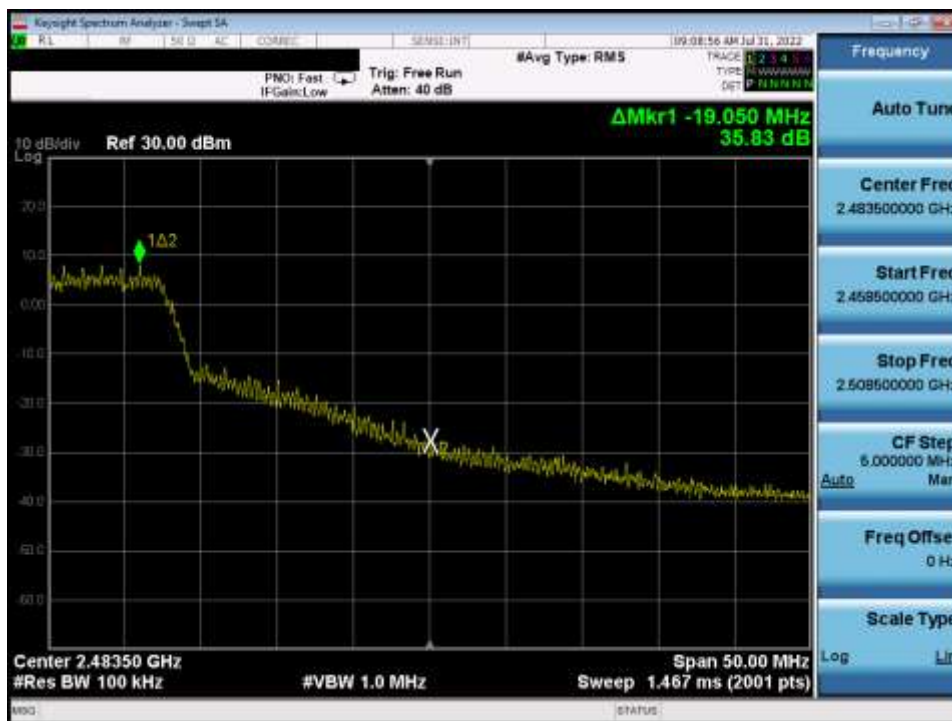
Plot 7-43. Band Edge Plot (802.11n MCS7 – Ch. 10)
