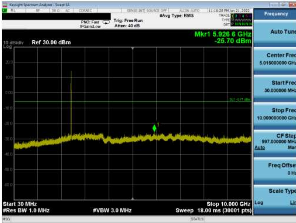
Plot 7-49. Conducted Spurious Plot (802.11b – Ch. 6)
