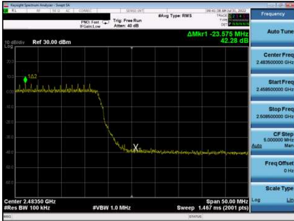
Plot 7-39. Band Edge Plot (802.11n MCS0 – Ch. 12)
