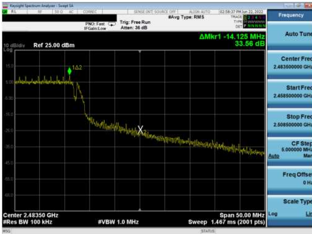
Plot 7-34. Band Edge Plot (802.11g – Ch. 13)
