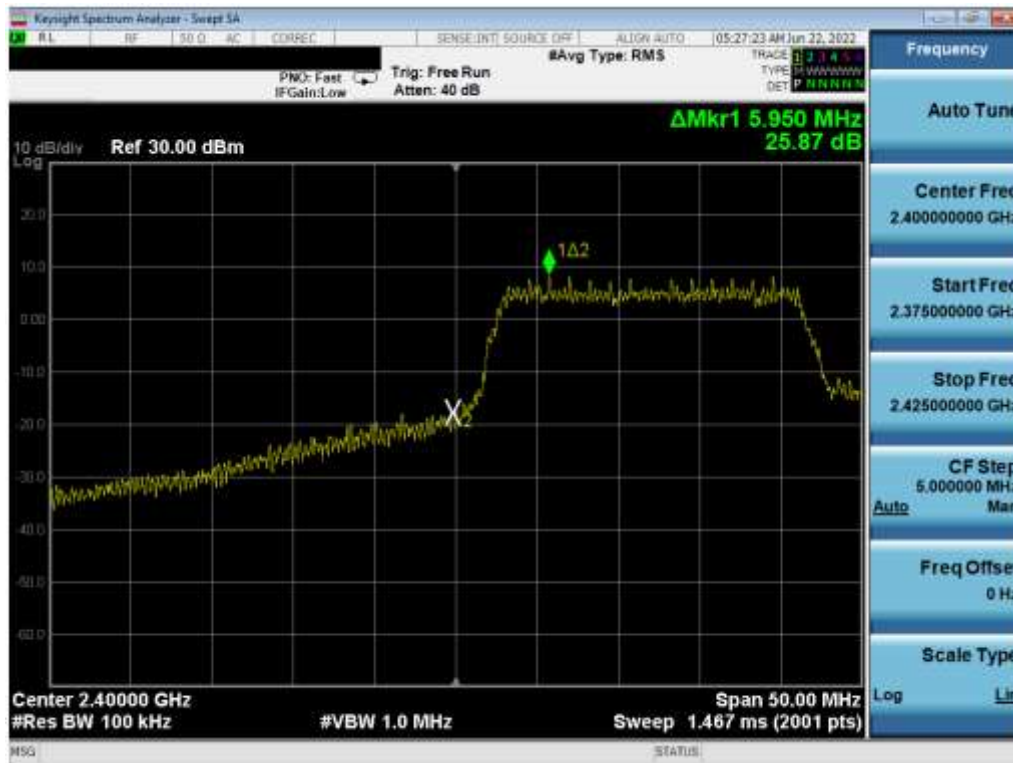
Plot 7-41. Band Edge Plot (802.11n MCS7 – Ch. 1)
