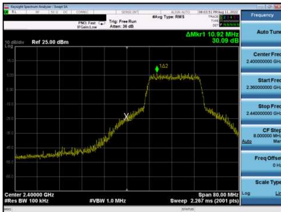
Plot 7-42. Band Edge Plot (802.11n MCS7 – Ch. 2)
