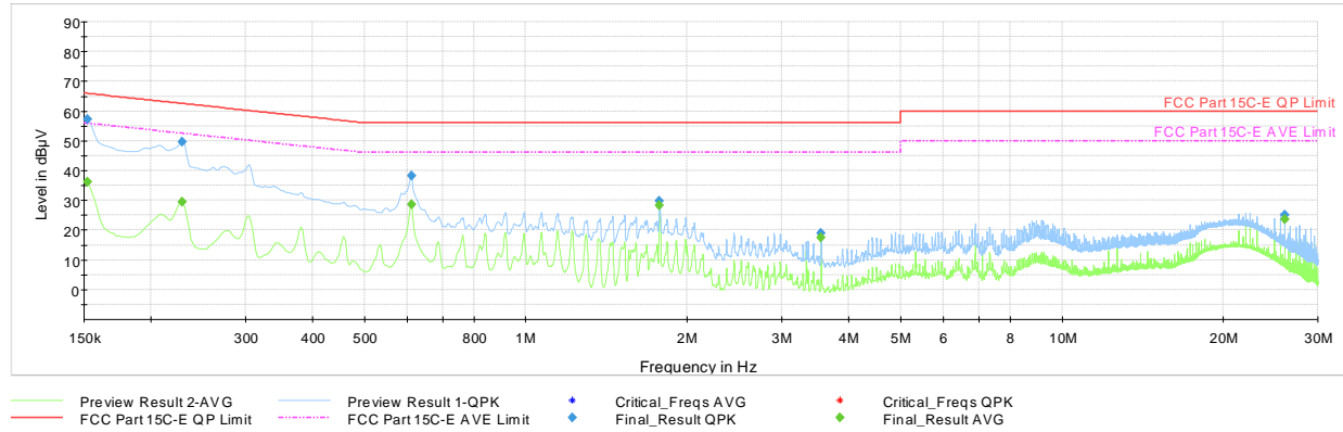
Plot 7-76. AC Line Conducted Plot 802.11b – Ch.6 (N), with Laptop
