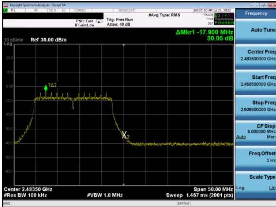
Plot 7-40. Band Edge Plot (802.11n MCS0 – Ch. 13)
