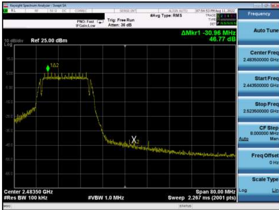
Plot 7-32. Band Edge Plot (802.11g– Ch. 11)
