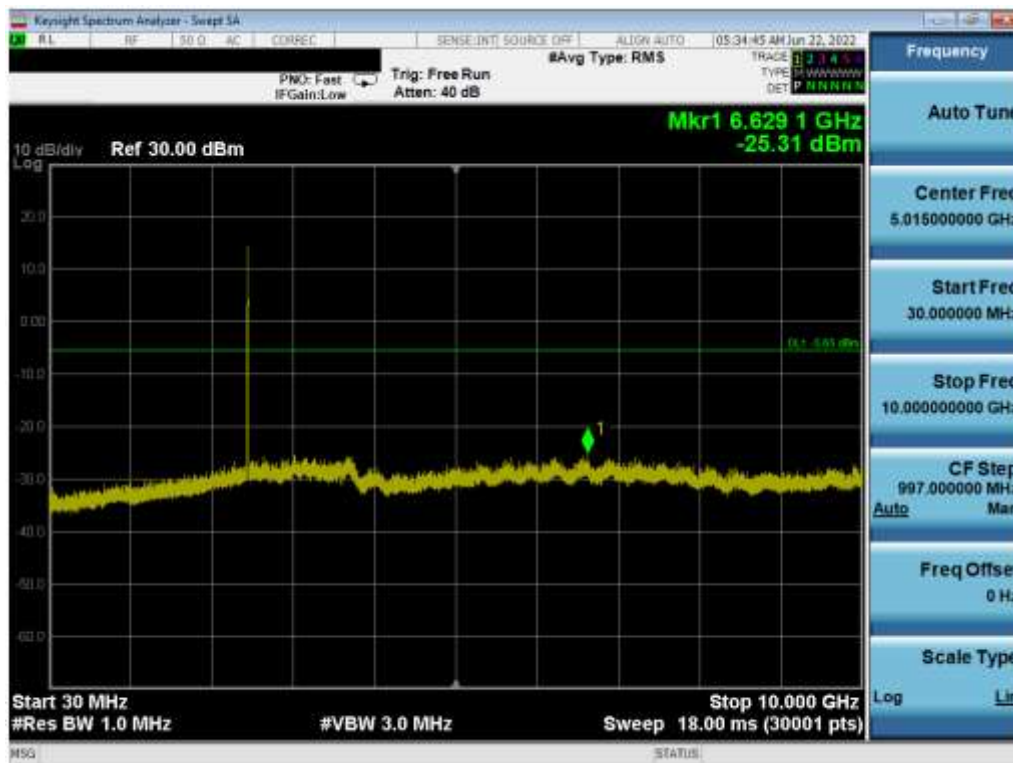
Plot 7-51. Conducted Spurious Plot (802.11b – Ch. 11)
