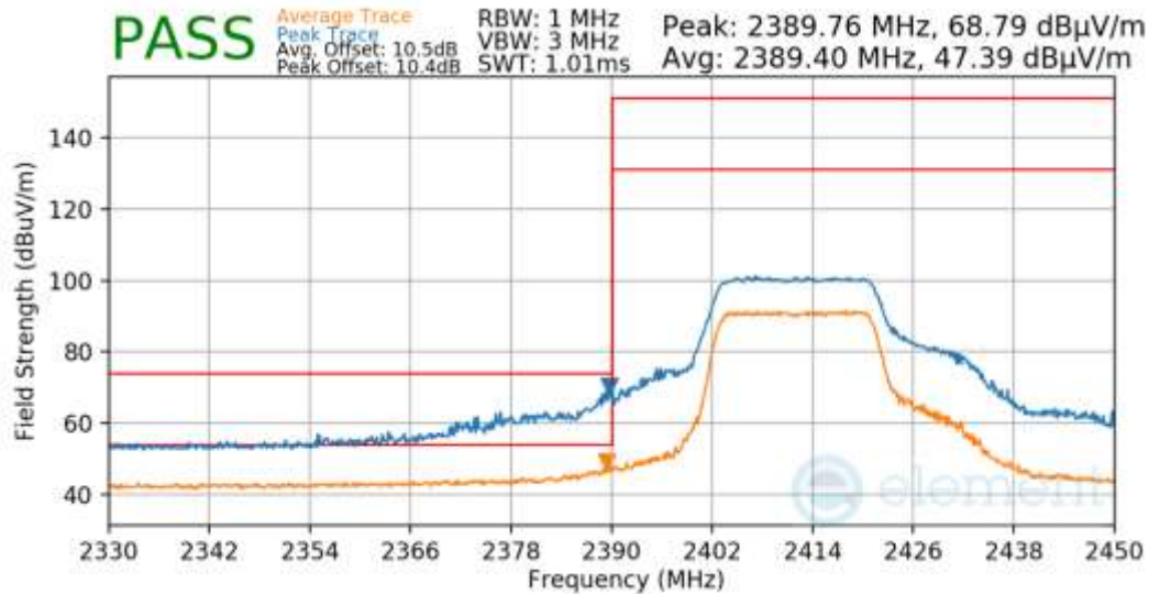
Plot 7-68. Radiated Restricted Lower Band Edge Measurement
