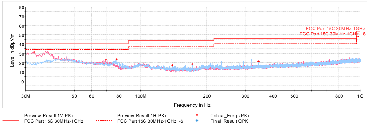
Plot 7-38. Radiated Spurious Emissions Below 1GHz (1Mbps, ePA – Ch.19, Pol. H & V, with AC/DC Adapter + Magnetic Charger)
