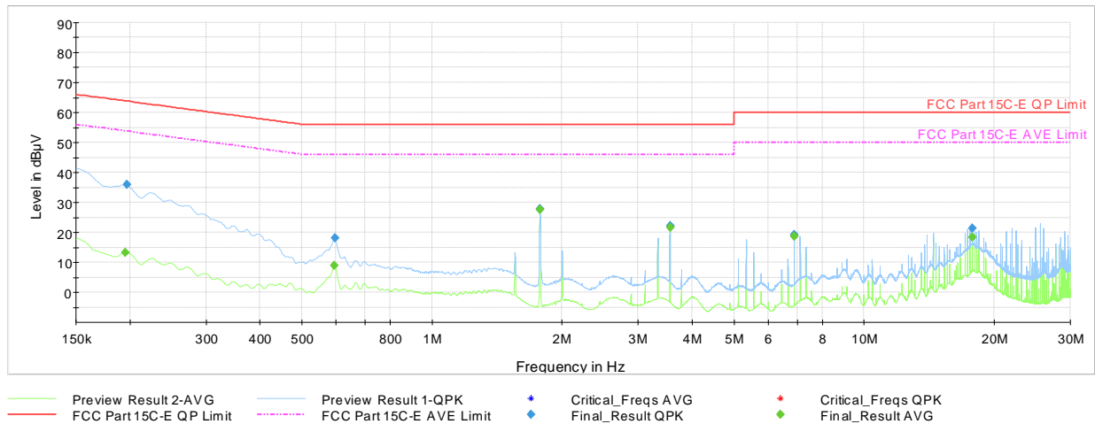
Plot 7-39. AC Line Conducted Plot with Bluetooth LE (L1, 1Mbps ePA – Ch.19 with AC/DC Adapter + Magnetic Charger)
