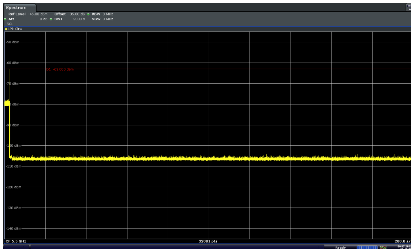
Figure 9-4. 5500MHz - Non-Occupancy Period (30 Minutes) - (20MHz)
