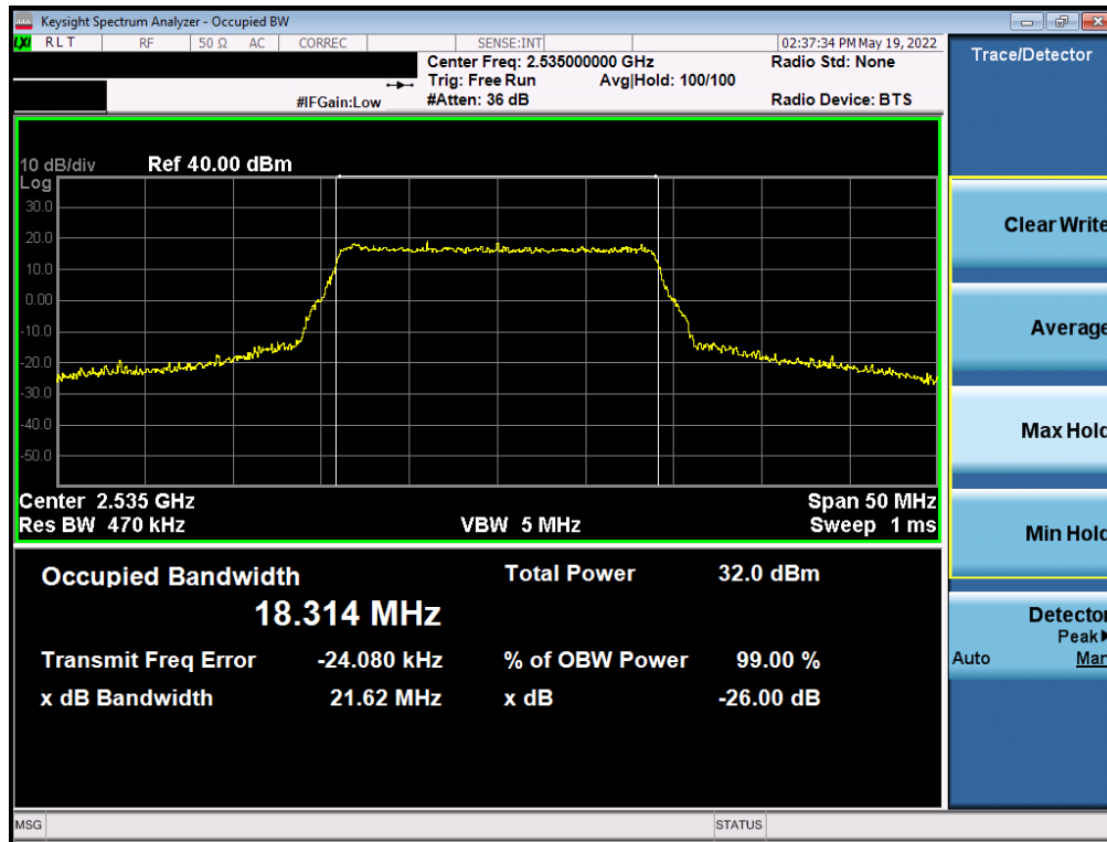
Plot 7-7. Occupied Bandwidth Plot (LTE Band 7 - 20MHz QPSK - Full RB)
