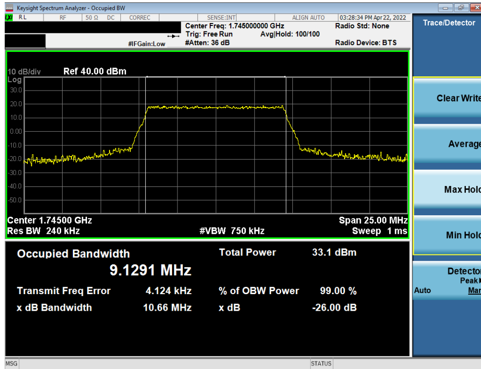
Plot 7-7. Occupied Bandwidth Plot (LTE Band 66/4 - 10MHz QPSK - Full RB)
