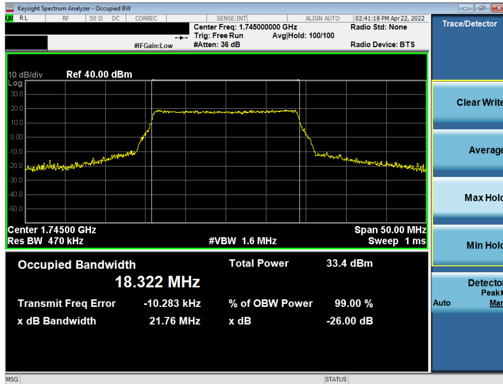
Plot 7-11. Occupied Bandwidth Plot (LTE Band 66/4 - 20MHz QPSK - Full RB)
