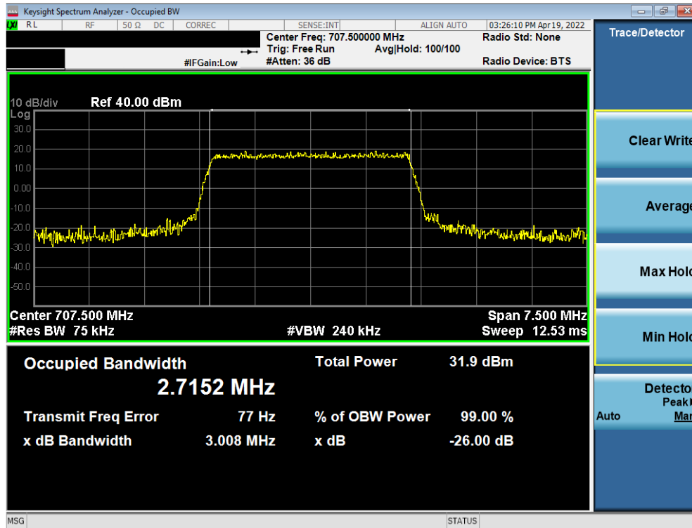
Plot 7-15. Occupied Bandwidth Plot (LTE Band 12 - 3MHz QPSK - Full RB)
