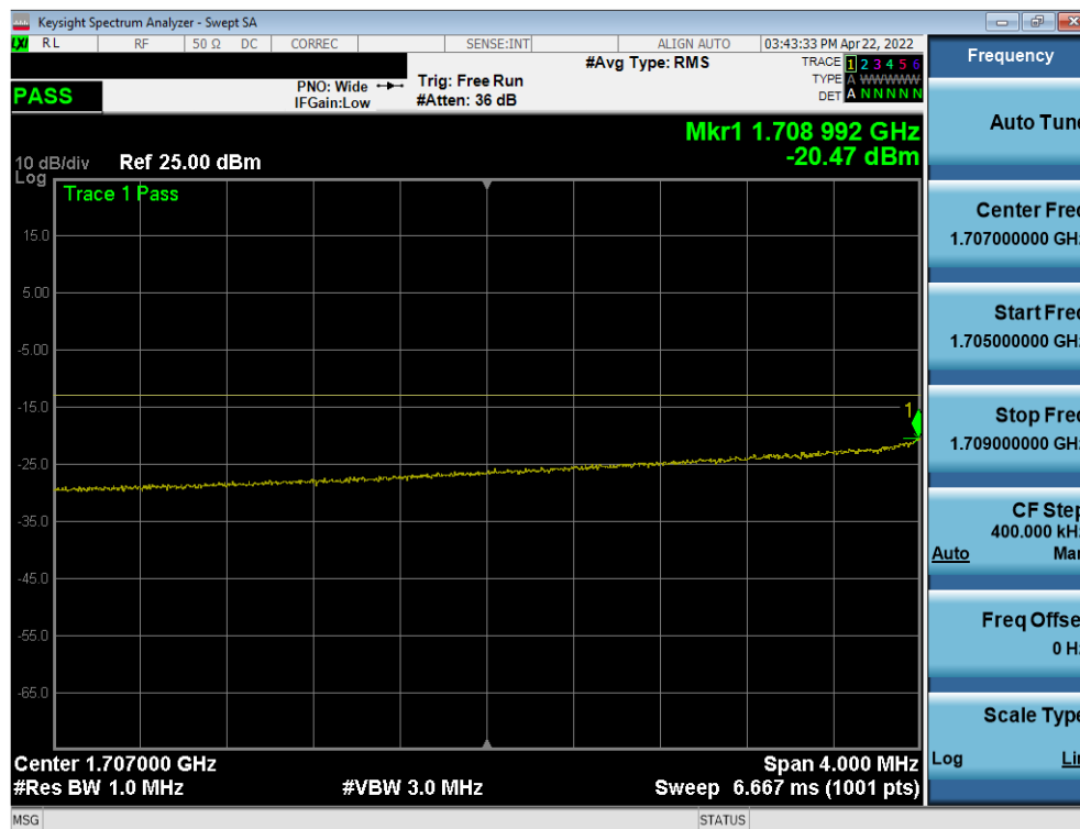
Plot 7-69. Lower Extended Band Edge Plot (LTE Band 66 - 10MHz QPSK – Full RB)
