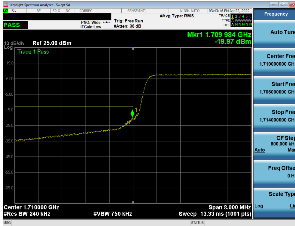
Plot 7-68. Lower Band Edge Plot (LTE Band 66 - 10MHz QPSK – Full RB)
