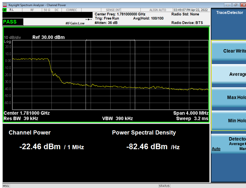
Plot 7-67. Upper Extended Band Edge Plot (LTE Band 66 - 5MHz QPSK – Full RB)
