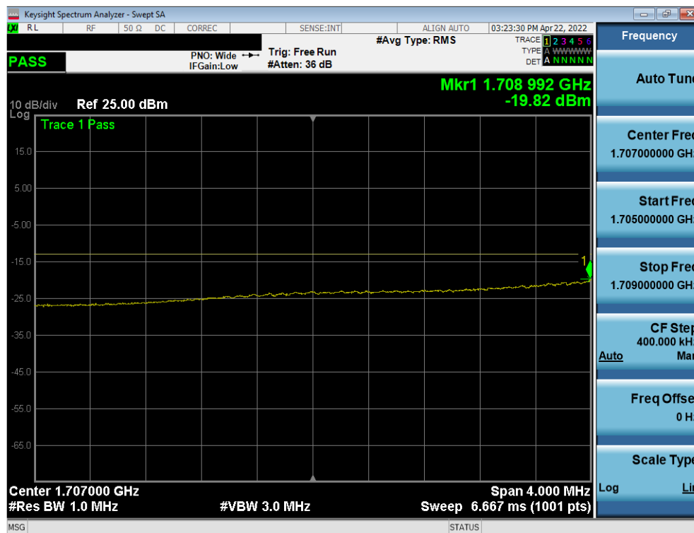
Plot 7-73. Lower Extended Band Edge Plot (LTE Band 66 - 15MHz QPSK – Full RB)
