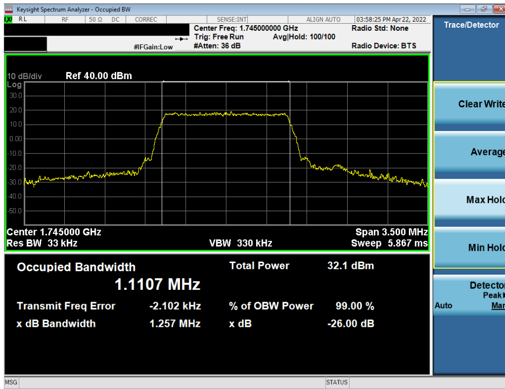
Plot 7-1. Occupied Bandwidth Plot (LTE Band 66/4 - 1.4MHz QPSK - Full RB)
