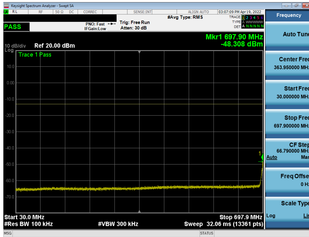
Plot 7-35. Conducted Spurious Plot (LTE Band 12/17 - 10MHz QPSK - RB Size 1, RB Offset 0 - Low Channel)
