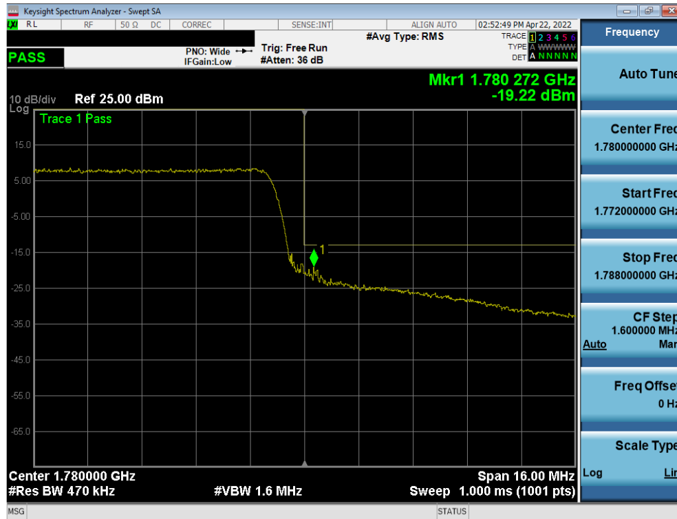
Plot 7-78. Upper Band Edge Plot (LTE Band 66 - 20MHz QPSK – Full RB)
