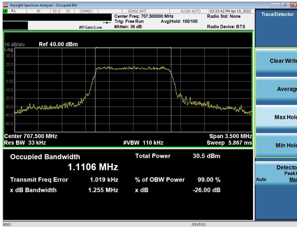
Plot 7-14. Occupied Bandwidth Plot (LTE Band 12 – 1.4MHz 16-QAM - Full RB)
