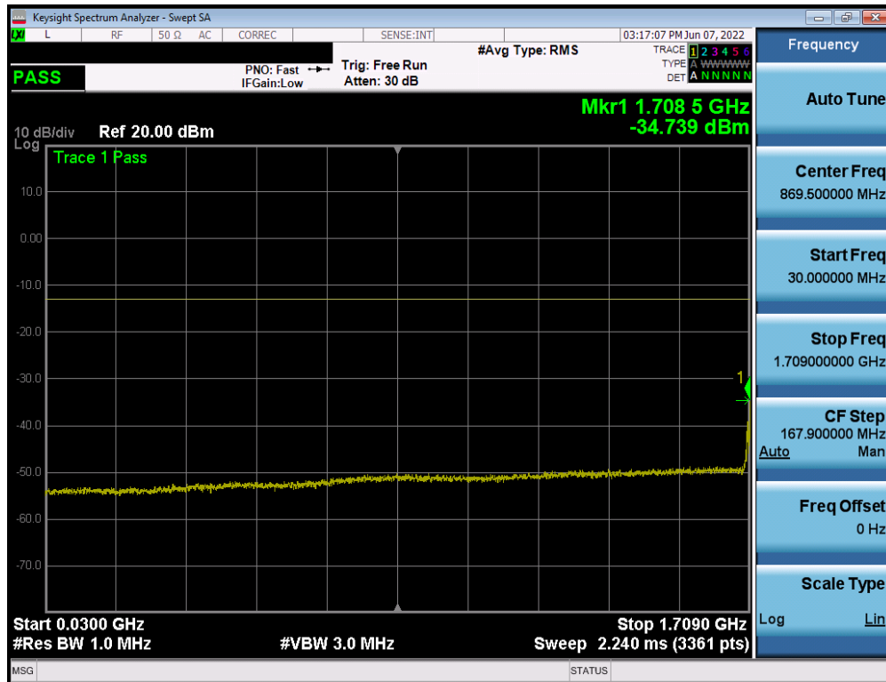
Plot 7-26. Conducted Spurious Plot (LTE Band 66/4 - 20MHz QPSK - RB Size 1, RB Offset 0 - Low Channel)
