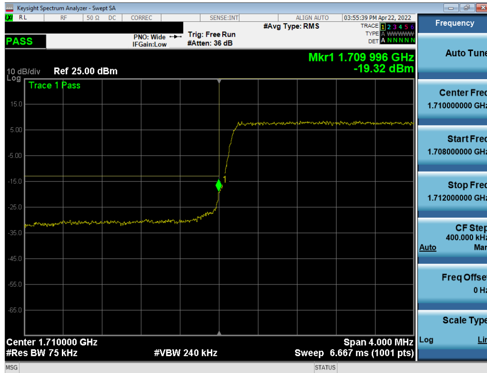
Plot 7-60. Lower Band Edge Plot (LTE Band 66 - 3MHz QPSK – Full RB)
