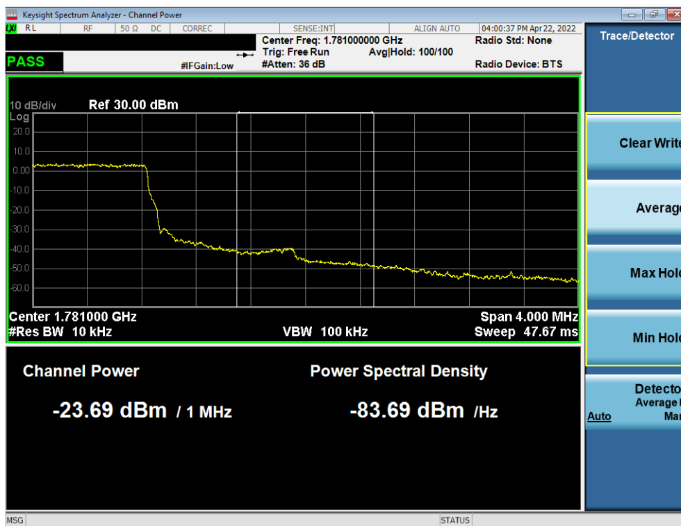
Plot 7-59. Upper Extended Band Edge Plot (LTE Band 66 – 1.4MHz QPSK – Full RB)
