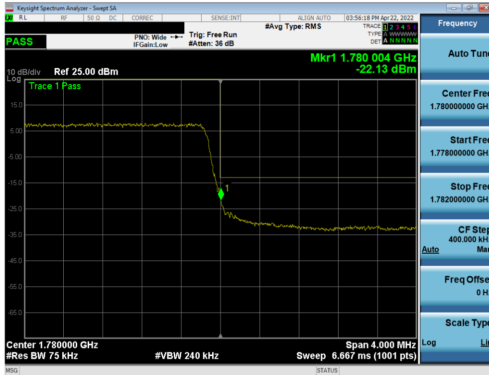
Plot 7-62. Upper Band Edge Plot (LTE Band 66 - 3MHz QPSK – Full RB)
