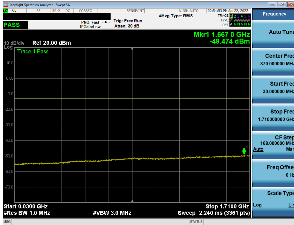
Plot 7-32. Conducted Spurious Plot (LTE Band 66/4 - 20MHz QPSK - RB Size 1, RB Offset 0 - High Channel)
