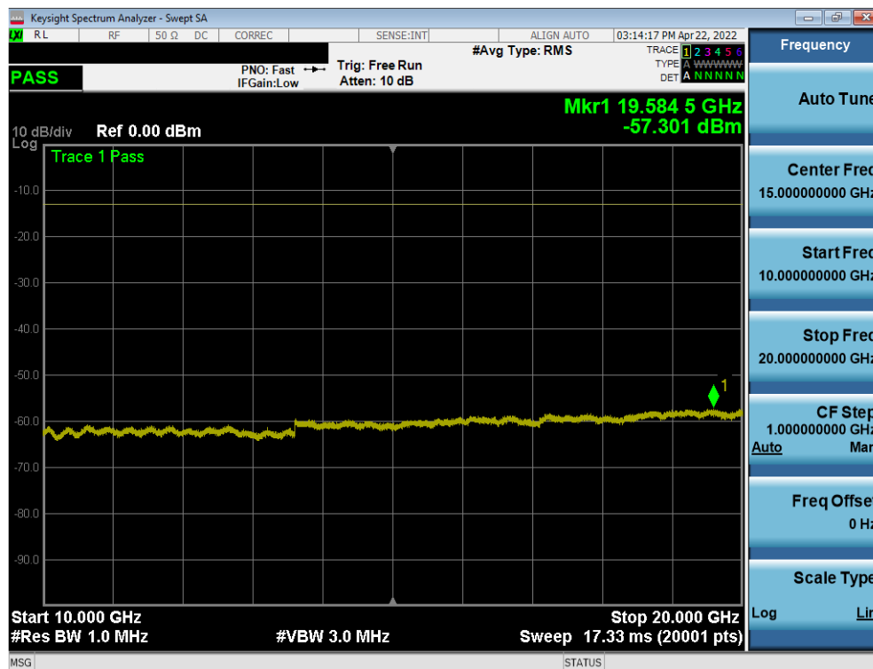
Plot 7-34. Conducted Spurious Plot (LTE Band 66/4 - 20MHz QPSK - RB Size 1, RB Offset 0 - High Channel)
