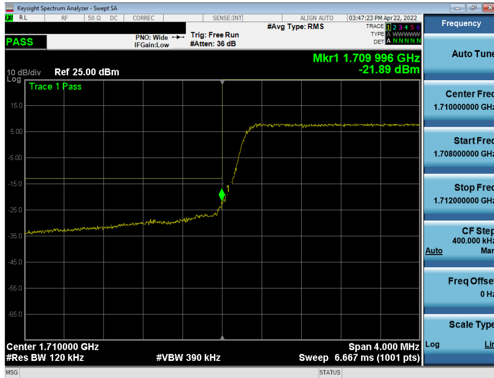
Plot 7-64. Lower Band Edge Plot (LTE Band 66 - 5MHz QPSK – Full RB)
