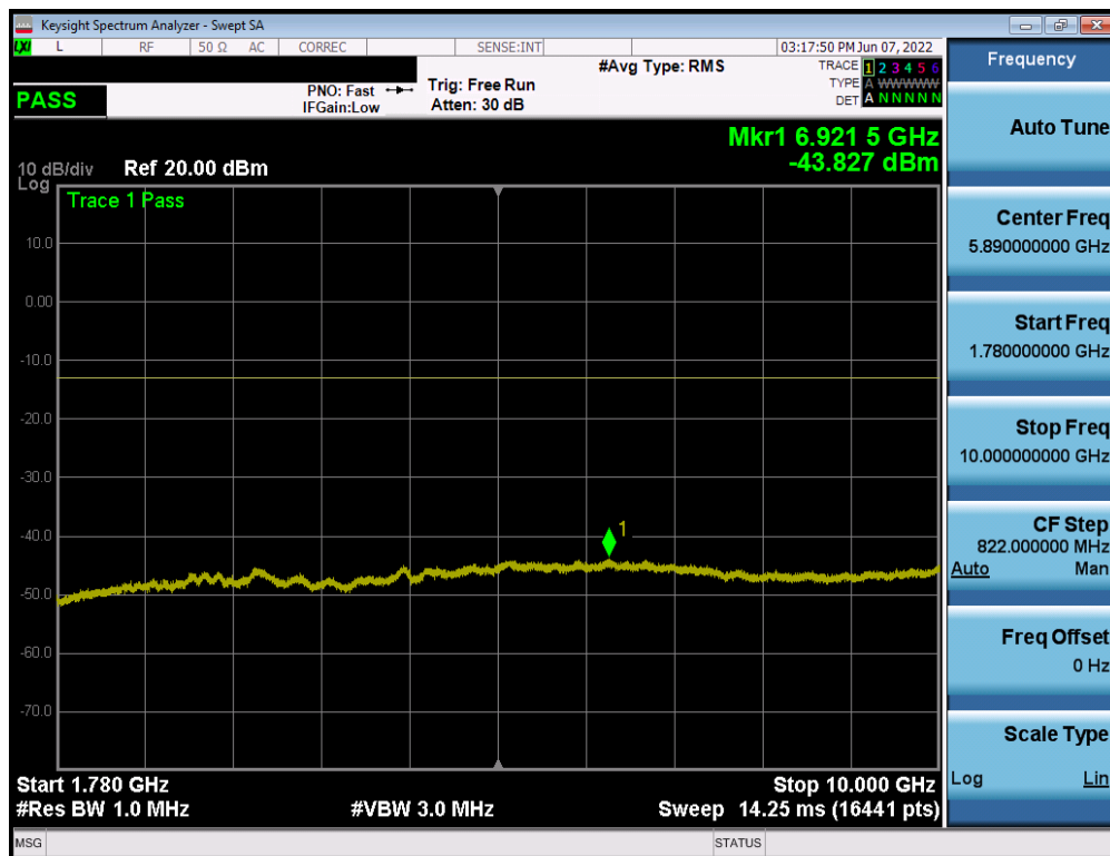
Plot 7-27. Conducted Spurious Plot (LTE Band 66/4 - 20MHz QPSK - RB Size 1, RB Offset 0 - Low Channel)
