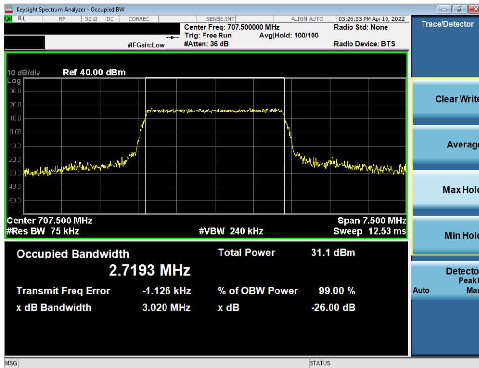
Plot 7-16. Occupied Bandwidth Plot (LTE Band 12 - 3MHz 16-QAM - Full RB)
