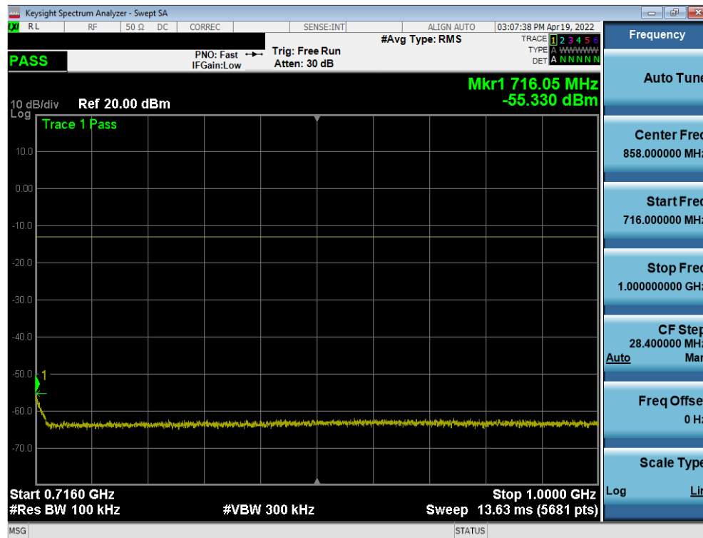
Plot 7-36. Conducted Spurious Plot (LTE Band 12/17 - 10MHz QPSK - RB Size 1, RB Offset 0 - Low Channel)
