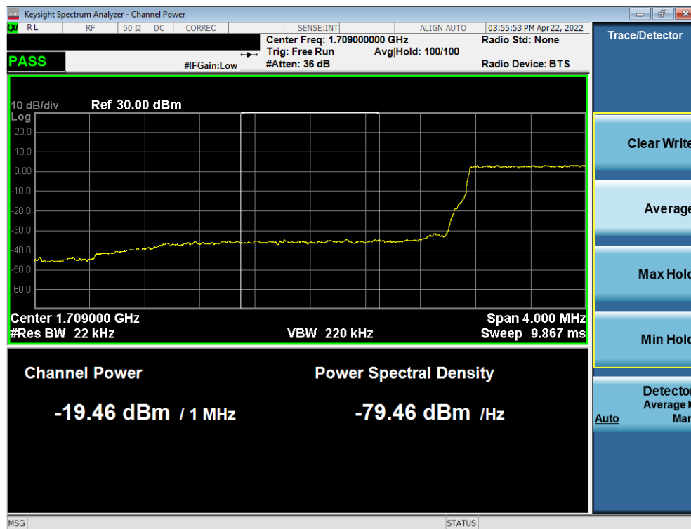
Plot 7-61. Lower Extended Band Edge Plot (LTE Band 66 - 3MHz QPSK – Full RB)
