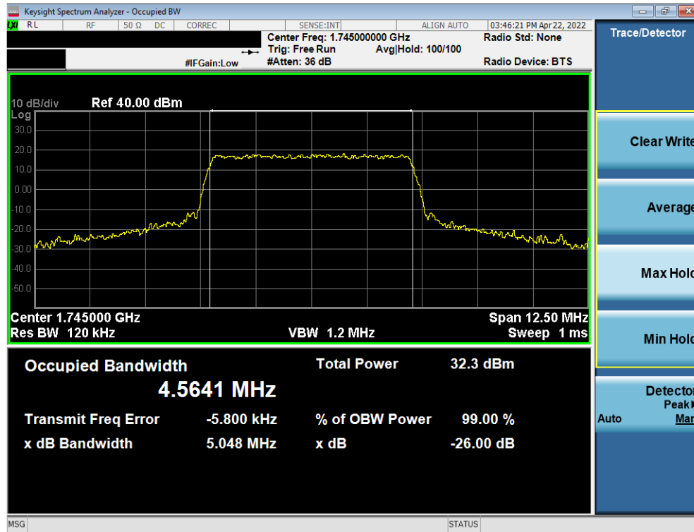
Plot 7-5. Occupied Bandwidth Plot (LTE Band 66/4 - 5MHz QPSK - Full RB)
