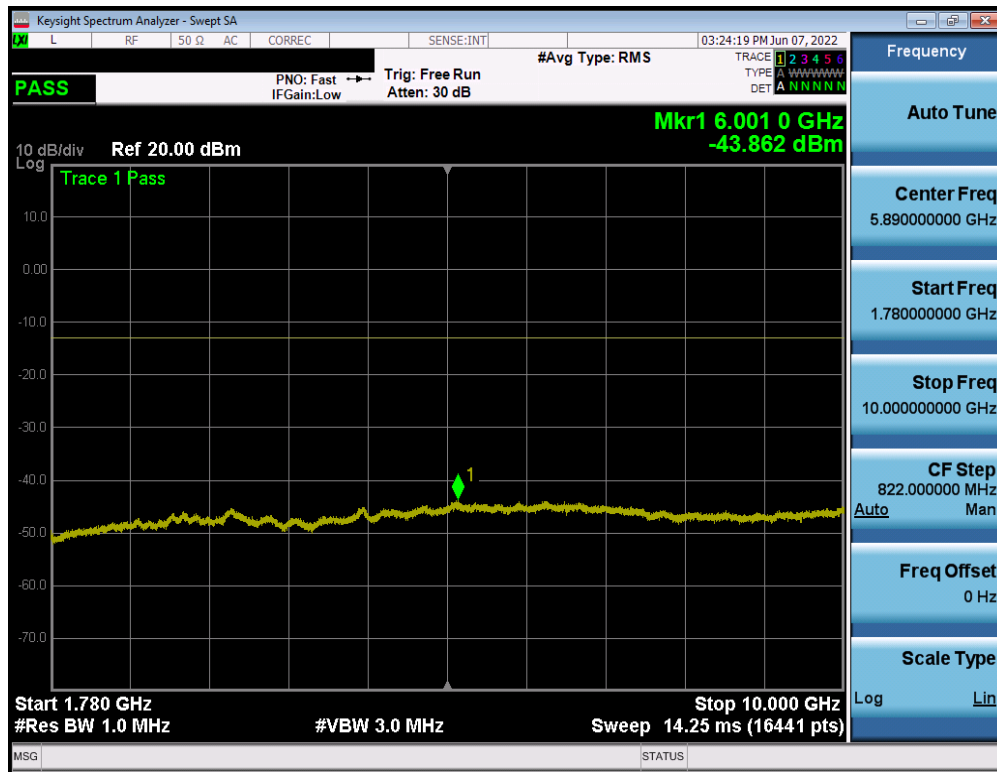
Plot 7-30. Conducted Spurious Plot (LTE Band 66/4 - 20MHz QPSK - RB Size 1, RB Offset 0 - Mid Channel)
