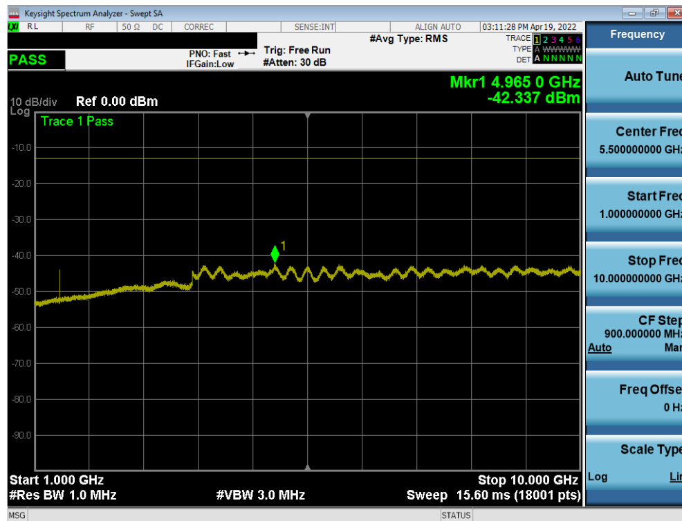
Plot 7-40. Conducted Spurious Plot (LTE Band 12/17 - 10MHz QPSK - RB Size 1, RB Offset 0 - Mid Channel)
