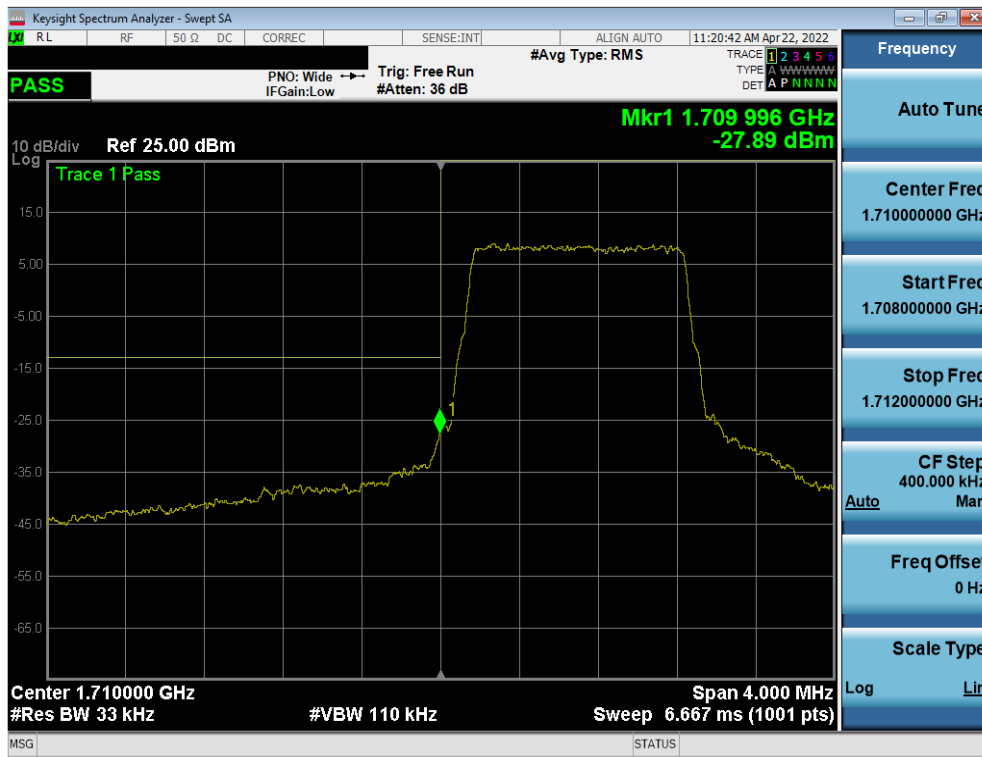
Plot 7-80. Lower Band Edge Plot (LTE Band 4 – 1.4MHz QPSK – Full RB)
