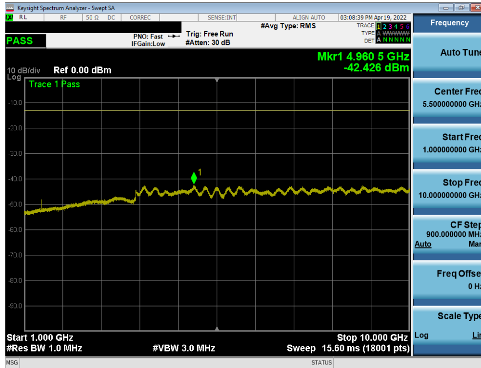
Plot 7-37. Conducted Spurious Plot (LTE Band 12/17 - 10MHz QPSK - RB Size 1, RB Offset 0 - Low Channel)
