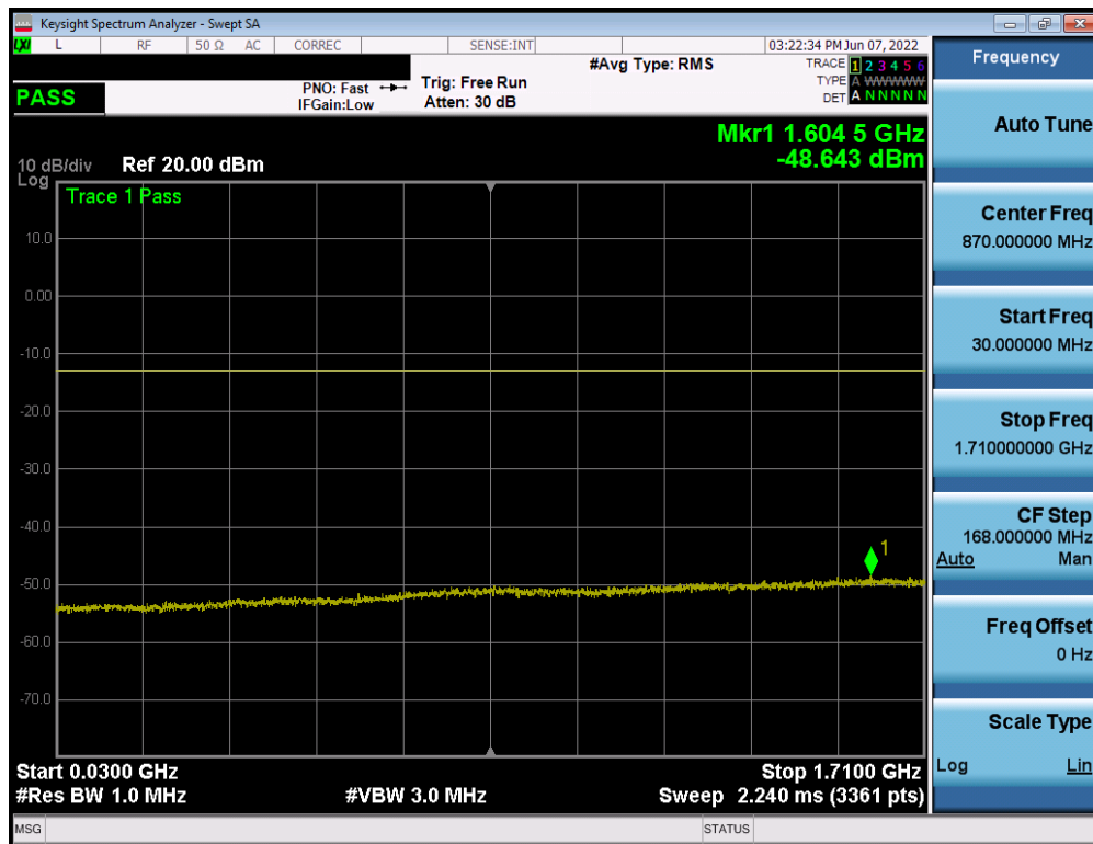
Plot 7-29. Conducted Spurious Plot (LTE Band 66/4 - 20MHz QPSK - RB Size 1, RB Offset 0 - Mid Channel)
