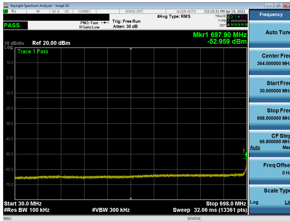
Plot 7-38. Conducted Spurious Plot (LTE Band 12/17 - 10MHz QPSK - RB Size 1, RB Offset 0 - Mid Channel)
