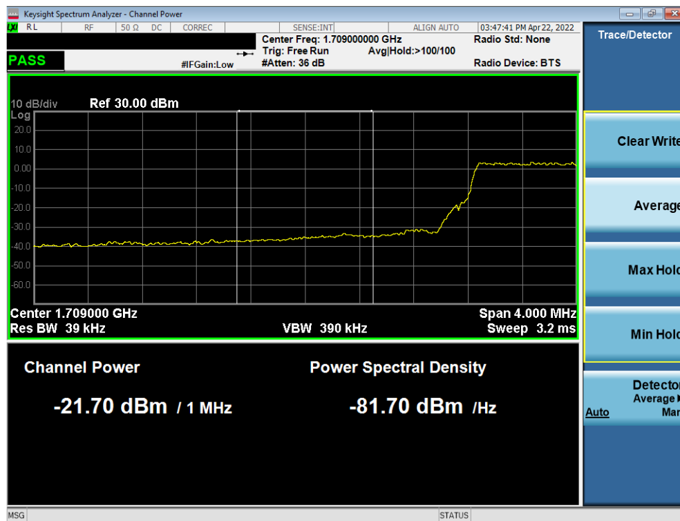
Plot 7-65. Lower Extended Band Edge Plot (LTE Band 66 - 5MHz QPSK – Full RB)
