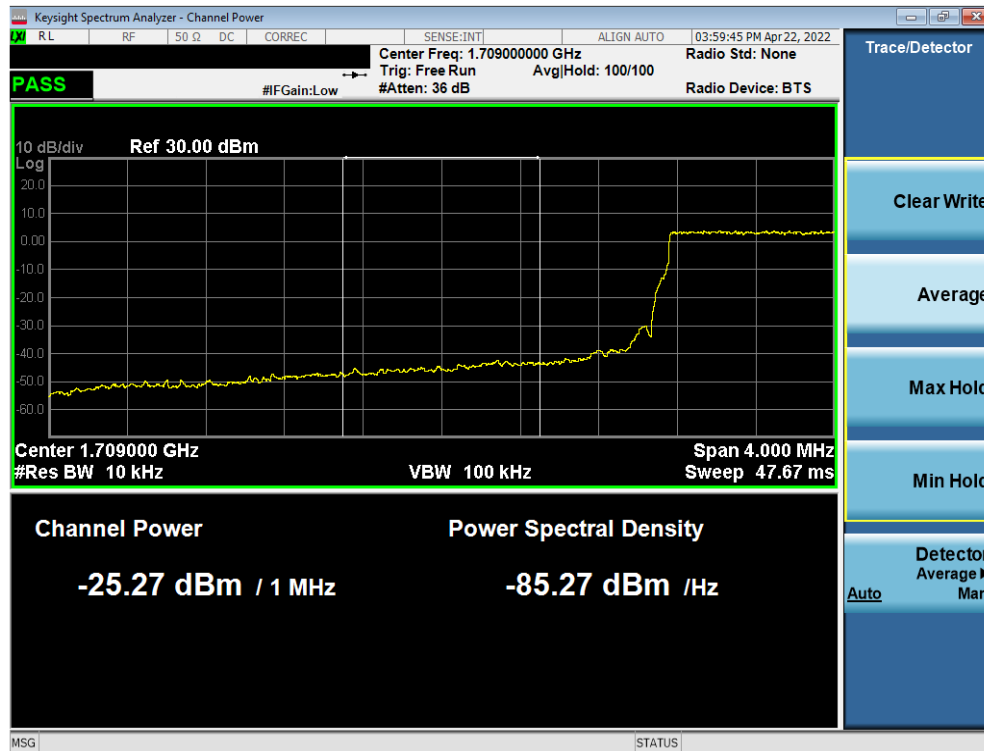
Plot 7-57. Lower Extended Band Edge Plot (LTE Band 66 – 1.4MHz QPSK – Full RB)
