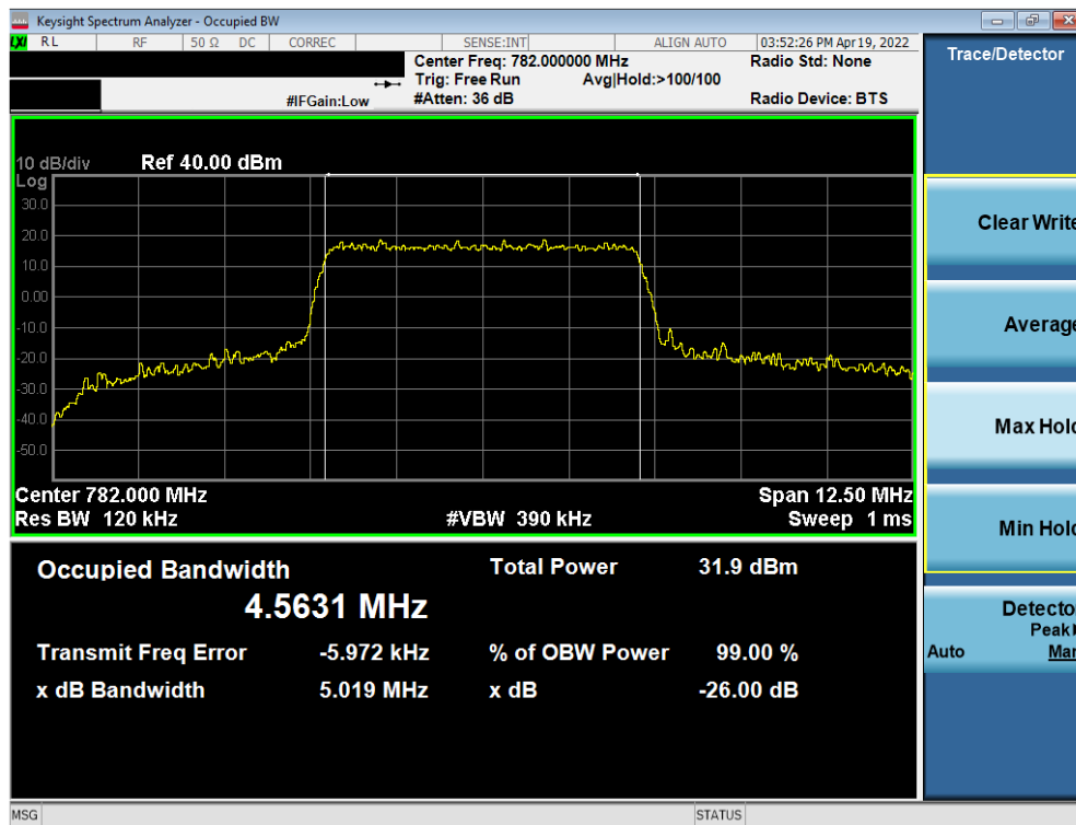
Plot 7-22. Occupied Bandwidth Plot (LTE Band 13 - 5MHz 16-QAM - Full RB)
