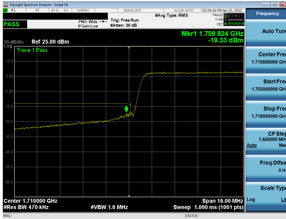
Plot 7-76. Lower Band Edge Plot (LTE Band 66 - 20MHz QPSK – Full RB)
