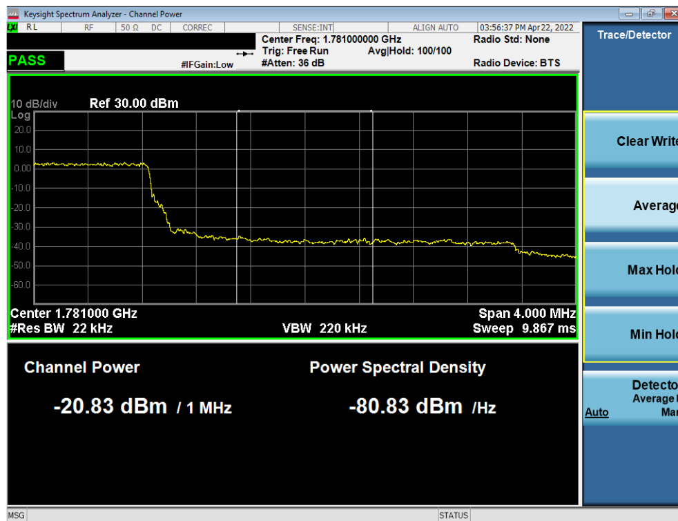
Plot 7-63. Upper Extended Band Edge Plot (LTE Band 66 - 3MHz QPSK – Full RB)
