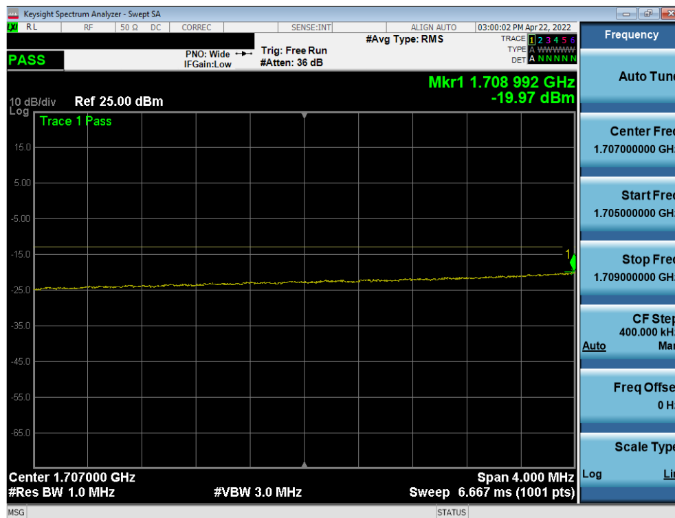
Plot 7-77. Lower Extended Band Edge Plot (LTE Band 66 - 20MHz QPSK – Full RB)
