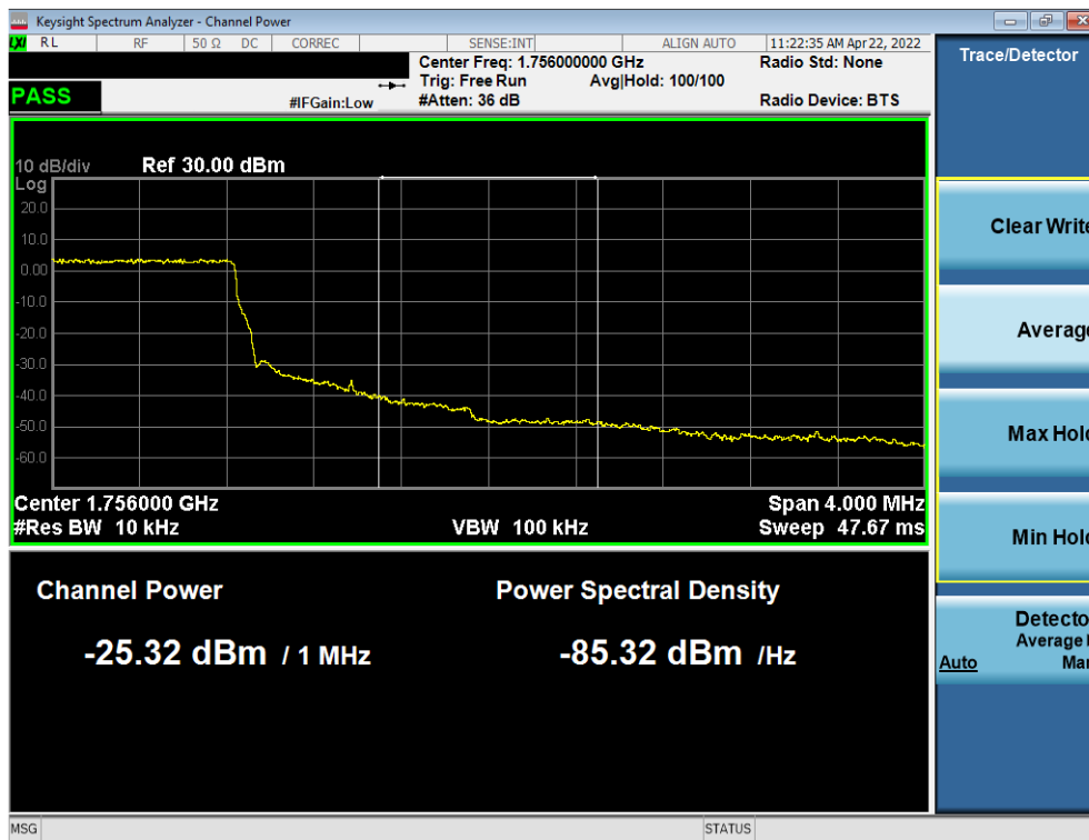
Plot 7-83. Upper Extended Band Edge Plot (LTE Band 4 – 1.4MHz QPSK – Full RB)
