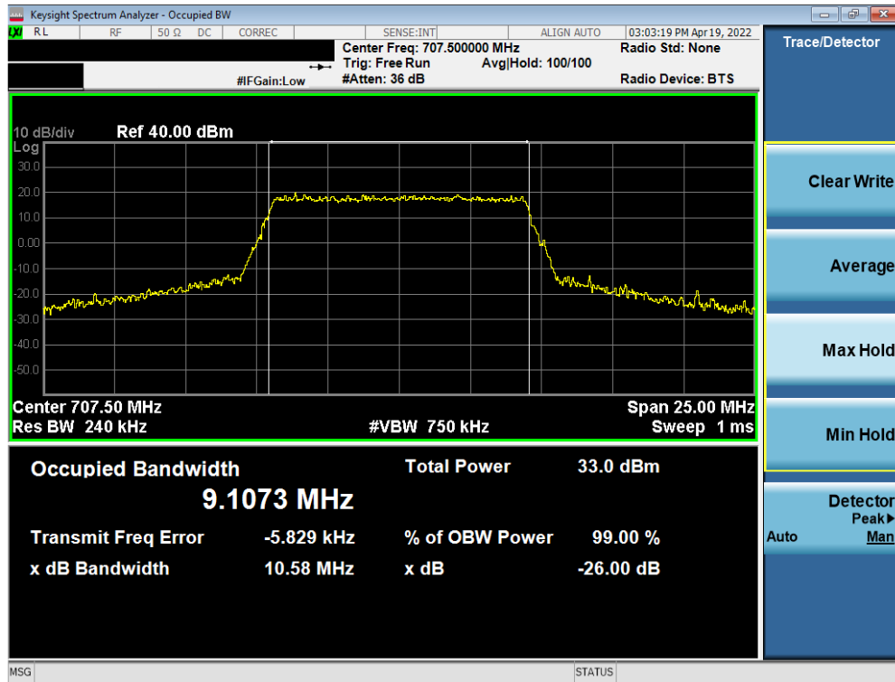
Plot 7-19. Occupied Bandwidth Plot (LTE Band 12/17 - 10MHz QPSK - Full RB)
