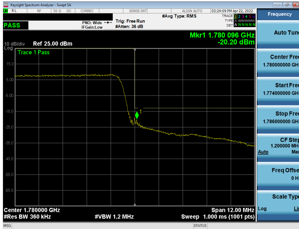
Plot 7-74. Upper Band Edge Plot (LTE Band 66 - 15MHz QPSK – Full RB)
