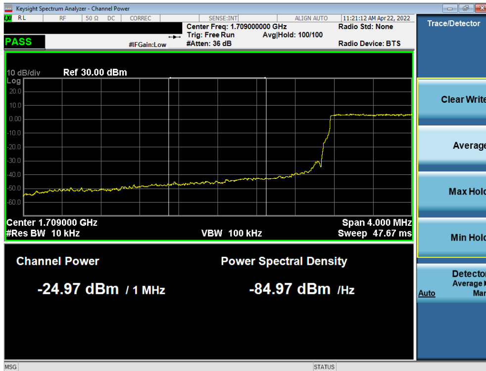
Plot 7-81. Lower Extended Band Edge Plot (LTE Band 4 – 1.4MHz QPSK – Full RB)
