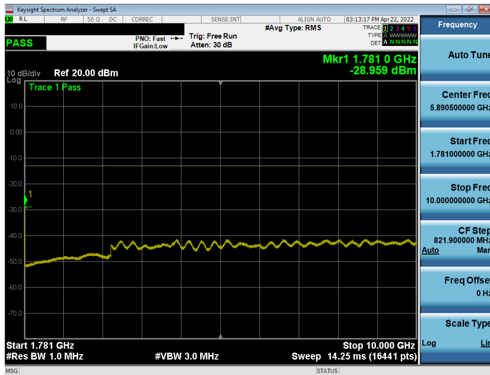
Plot 7-33. Conducted Spurious Plot (LTE Band 66/4 - 20MHz QPSK - RB Size 1, RB Offset 0 - High Channel)
