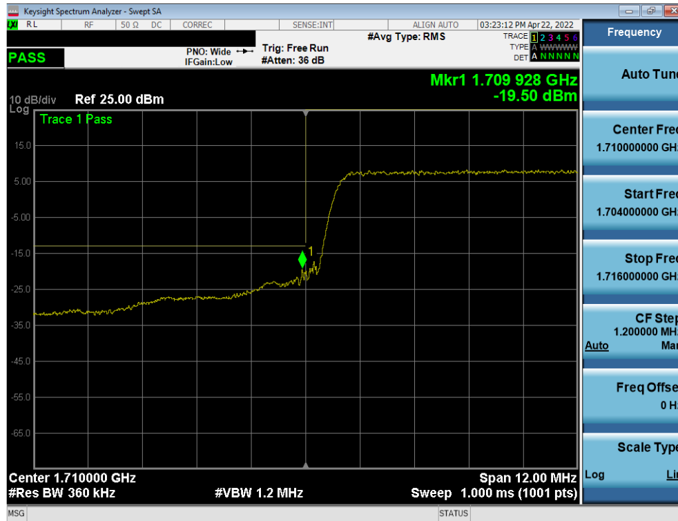
Plot 7-72. Lower Band Edge Plot (LTE Band 66 - 15MHz QPSK – Full RB)
