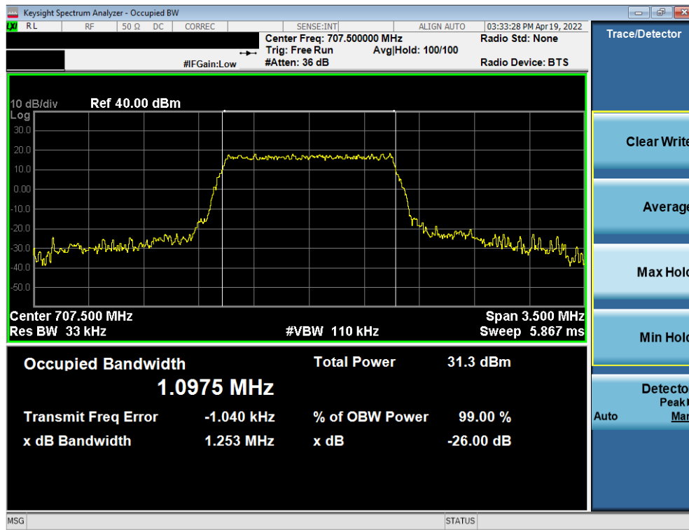
Plot 7-13. Occupied Bandwidth Plot (LTE Band 12 – 1.4MHz QPSK - Full RB)
