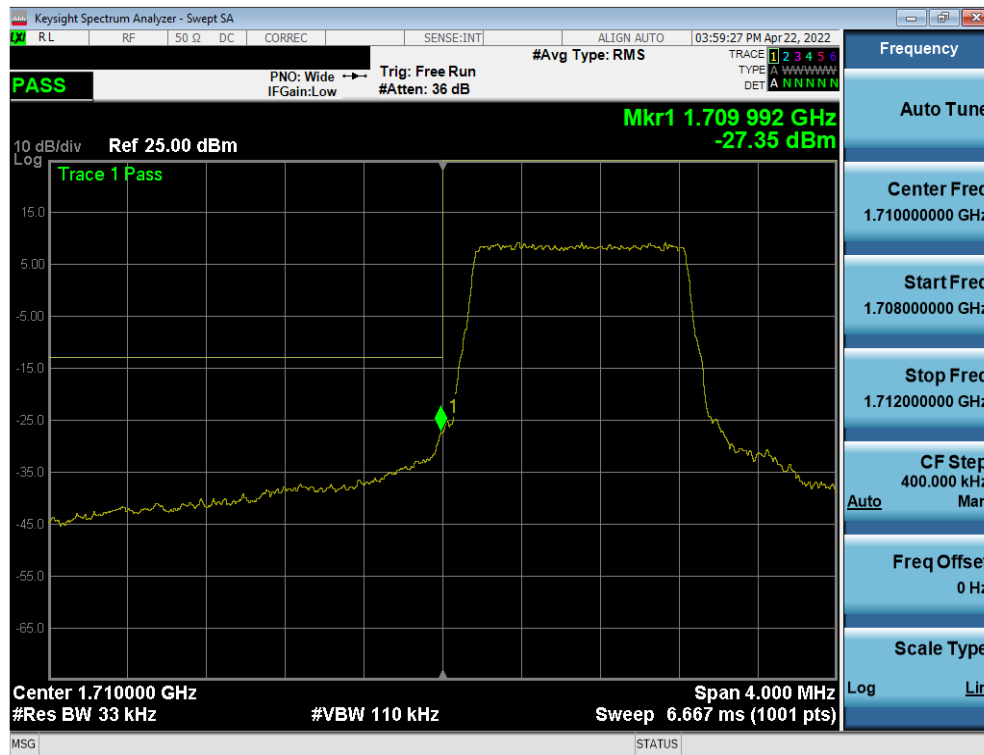
Plot 7-56. Lower Band Edge Plot (LTE Band 66 – 1.4MHz QPSK – Full RB)
