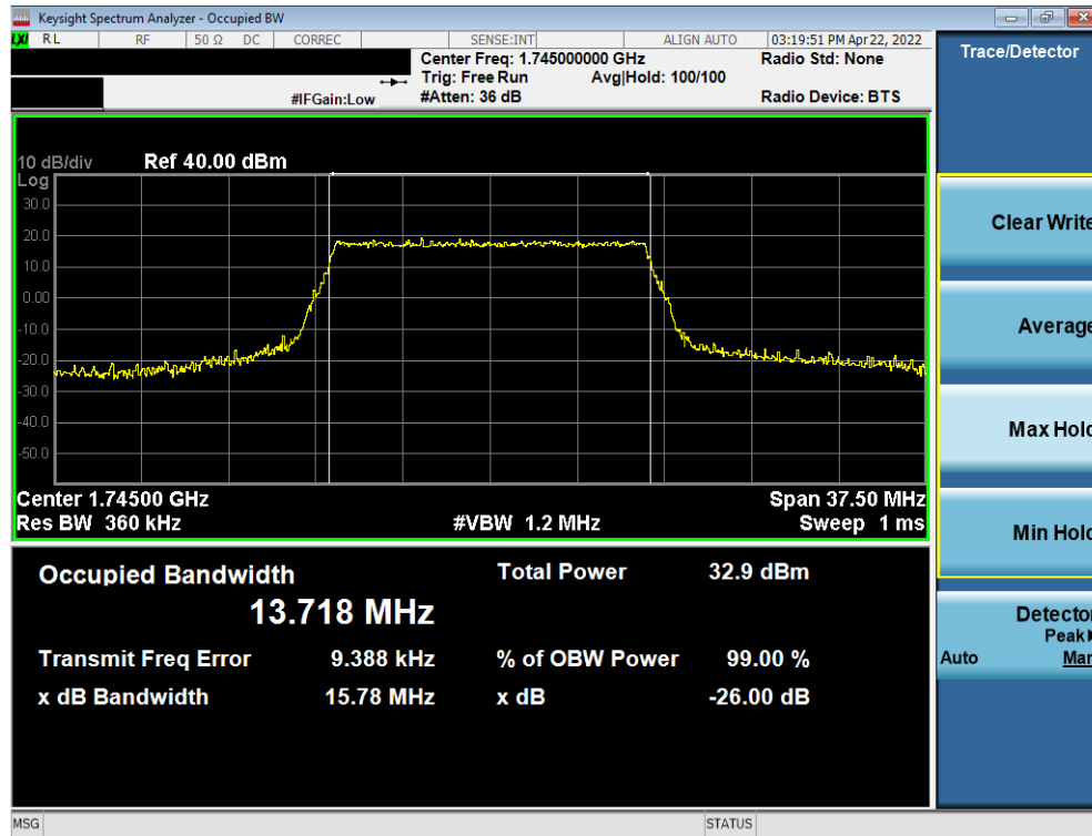
Plot 7-9. Occupied Bandwidth Plot (LTE Band 66/4 - 15MHz QPSK - Full RB)
