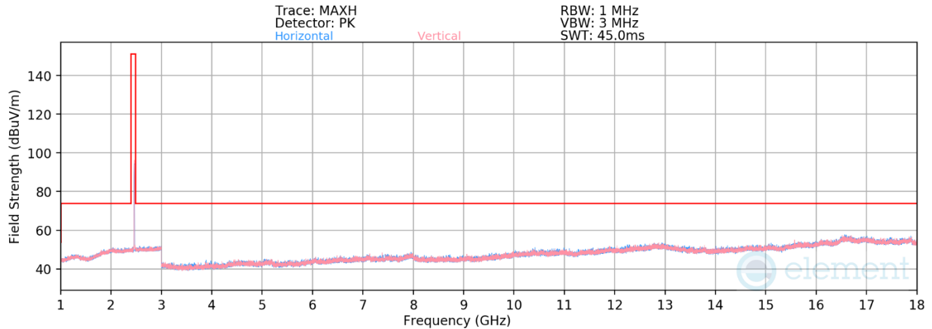
Plot 7-52. Radiated Spurious Emissions above 1GHz (802.11b – Ch. 11)
