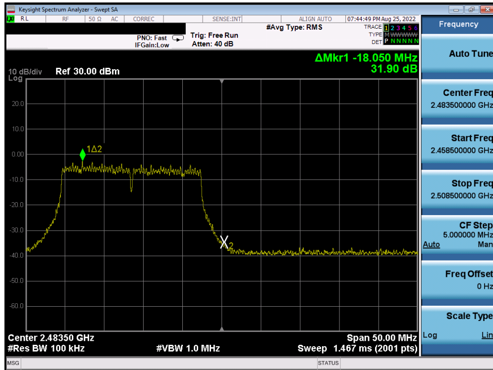
Plot 7-43. Band Edge Plot (802.11n MCS7 – Ch. 13)
