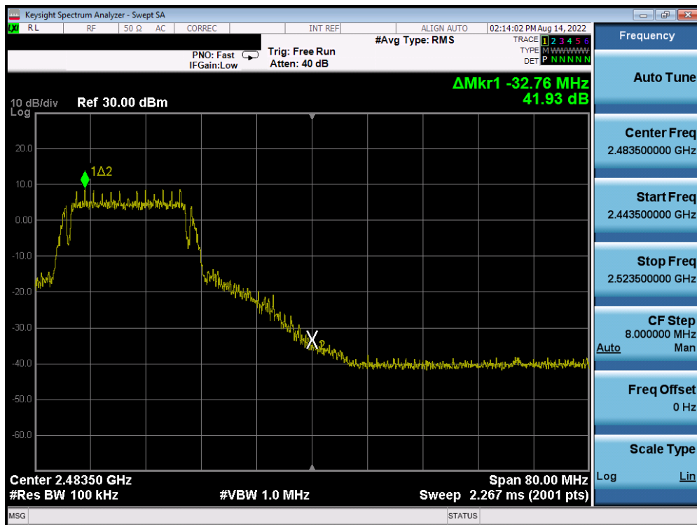
Plot 7-30. Band Edge Plot (802.11g – Ch. 10)
