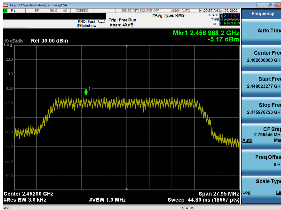
Plot 7-24. Power Spectral Density Plot (802.11n MCS7 – Ch. 11)
