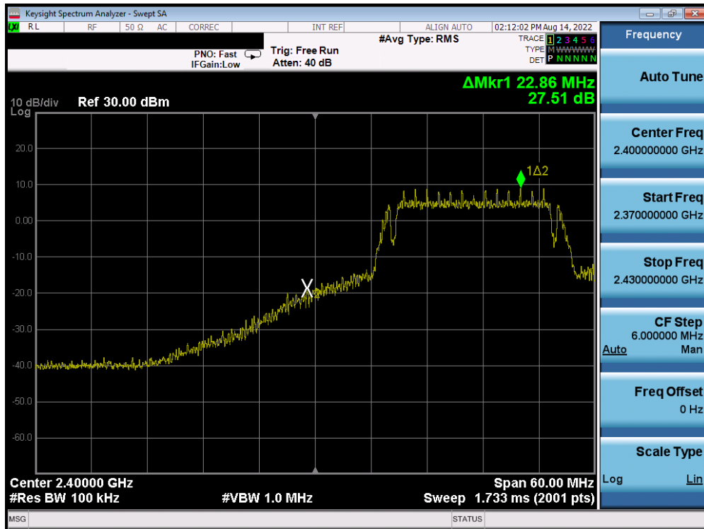
Plot 7-29. Band Edge Plot (802.11g– Ch. 2)
