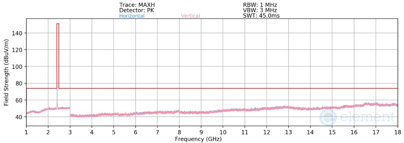
Plot 7-50. Radiated Spurious Emissions above 1GHz (802.11b – Ch. 1)
