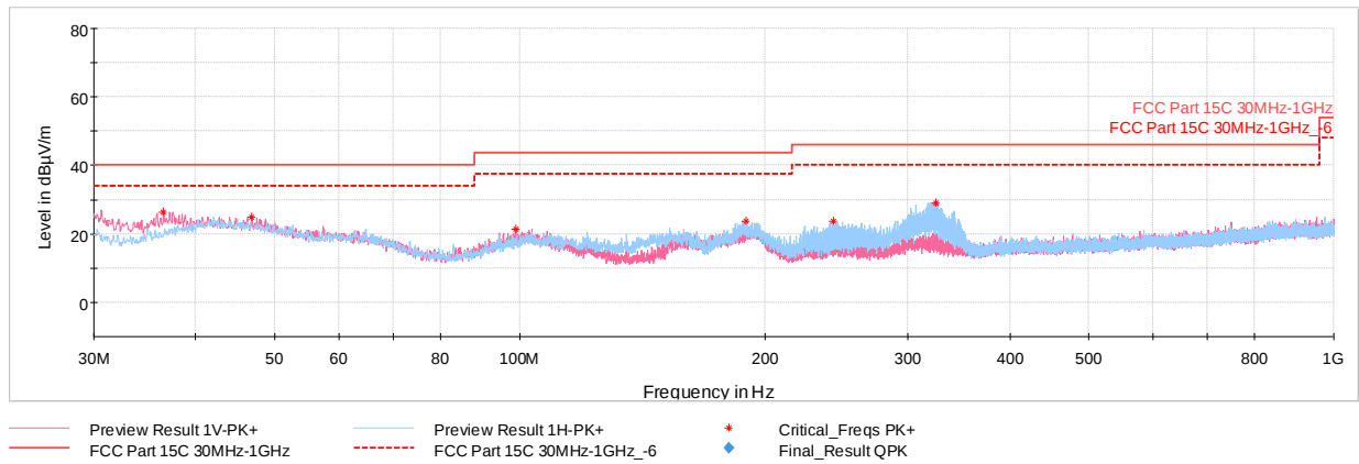
Plot 7-72. Radiated Spurious Emissions 30MHz - 1GHz 802.11b - Ch.6, with AC/DC Adapter and Magnetic Charger
