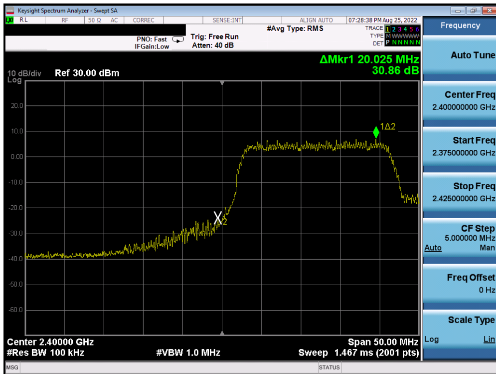
Plot 7-40. Band Edge Plot (802.11n MCS7 – Ch. 1)
