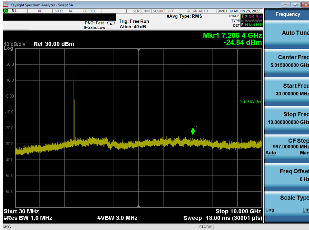
Plot 7-44. Conducted Spurious Plot (802.11b – Ch. 1)
