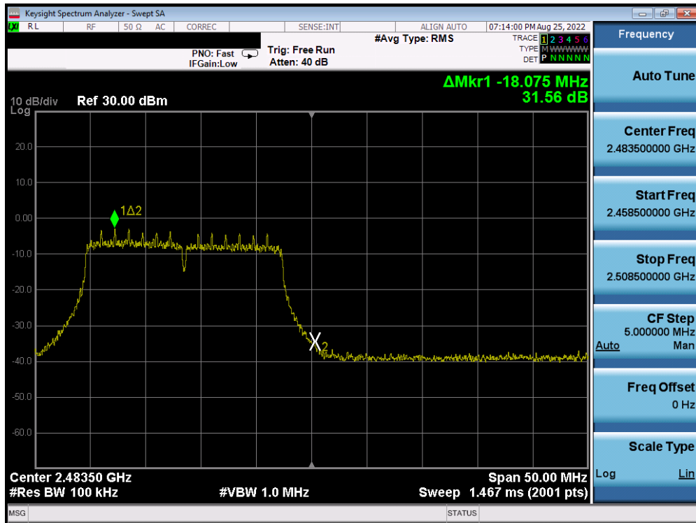
Plot 7-39. Band Edge Plot (802.11n MCS0 – Ch. 13)
