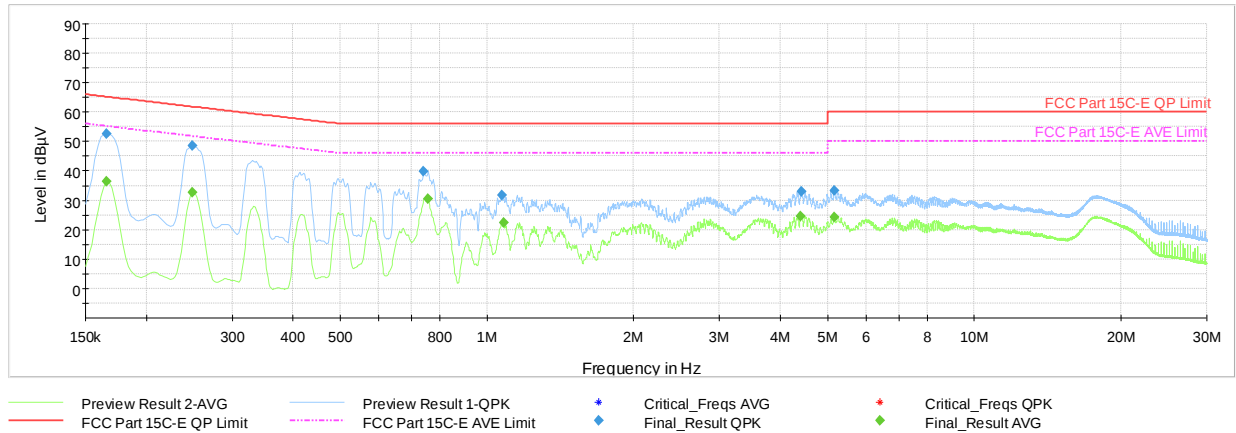
Plot 7-74. AC Line Conducted Plot 802.11b - Ch.6 (L1, with AC/DC Adapter + Laptop Charger)
