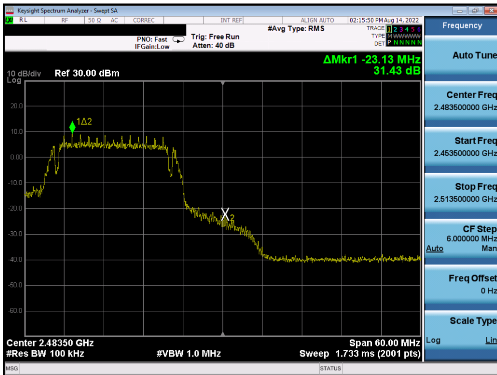
Plot 7-32. Band Edge Plot (802.11g – Ch. 12)
