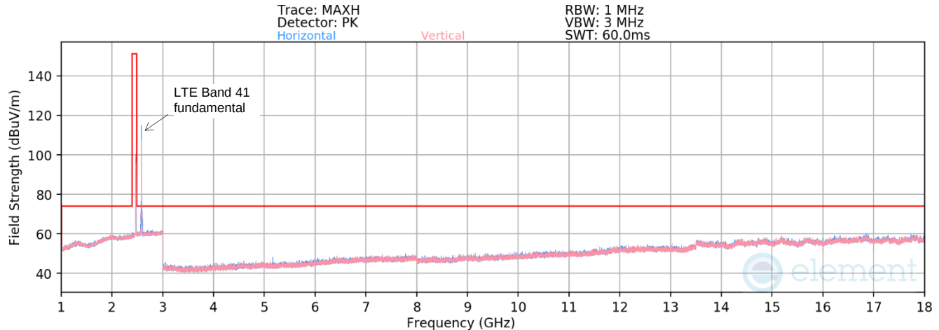
Plot 7-55. Radiated Spurious Emissions 1 - 18GHz – Simultaneous Transmission
