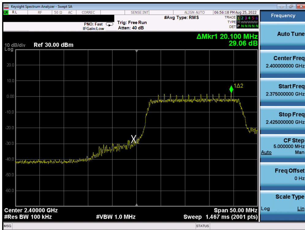
Plot 7-34. Band Edge Plot (802.11n MCS0 – Ch. 1)
