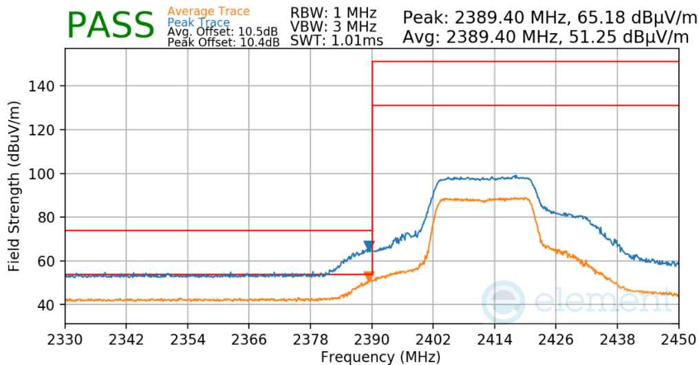
Plot 7-68. Radiated Restricted Lower Band Edge Measurement
