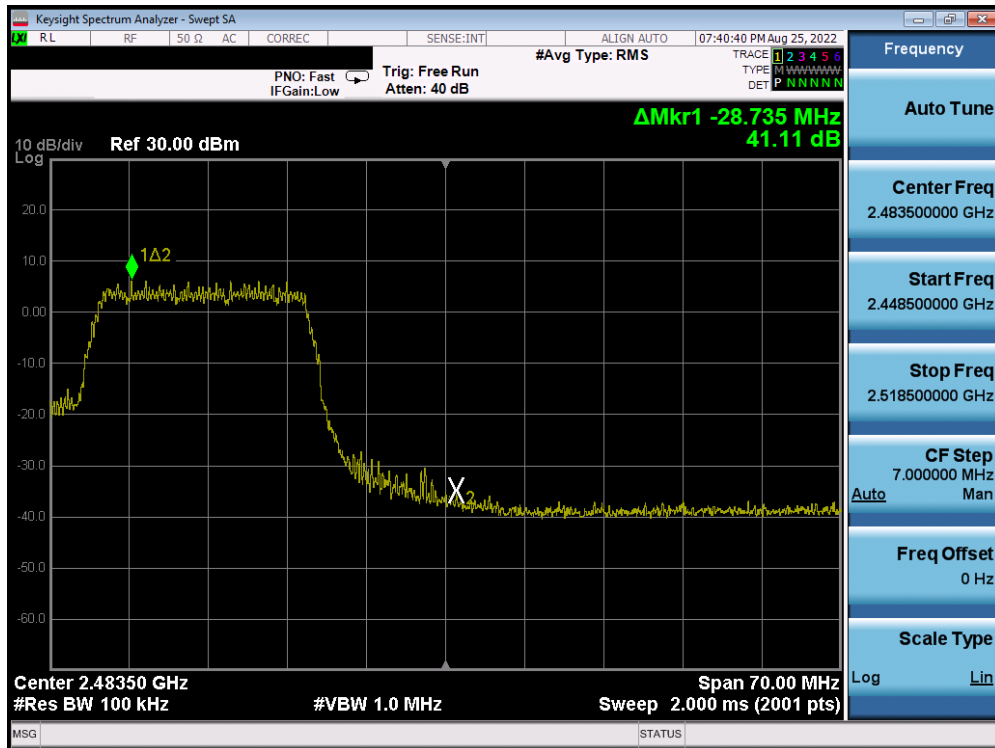
Plot 7-41. Band Edge Plot (802.11n MCS7 – Ch. 11)
