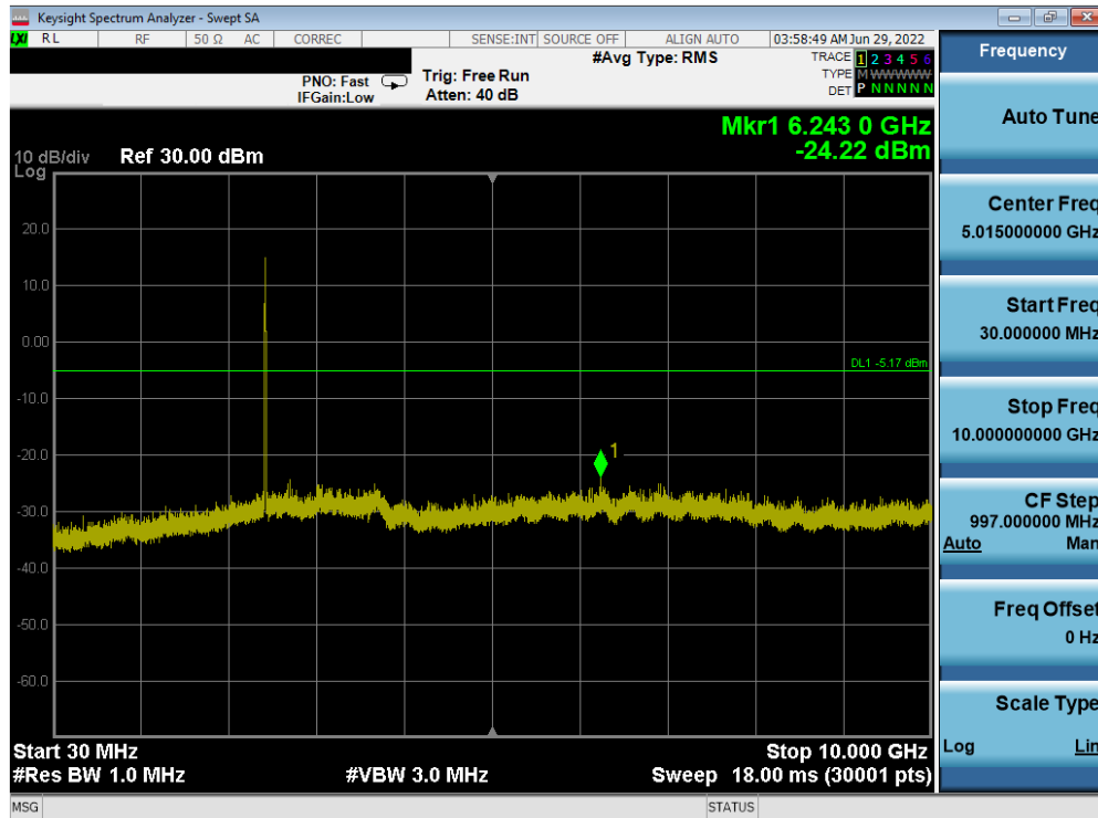
Plot 7-46. Conducted Spurious Plot (802.11b – Ch. 6)
