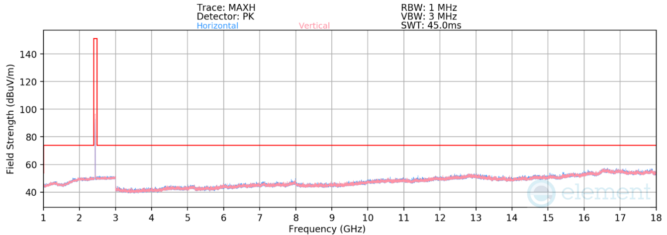
Plot 7-51. Radiated Spurious Emissions above 1GHz (802.11b – Ch. 6)
