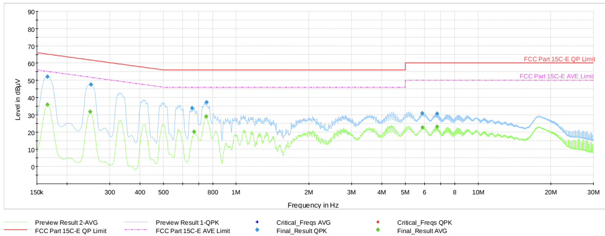
Plot 7-75. AC Line Conducted Plot 802.11b - Ch.6 (N, with AC/DC Adapter + Laptop Charger)
