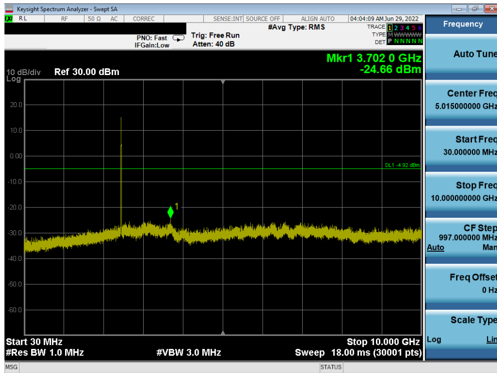
Plot 7-48. Conducted Spurious Plot (802.11b – Ch. 11)
