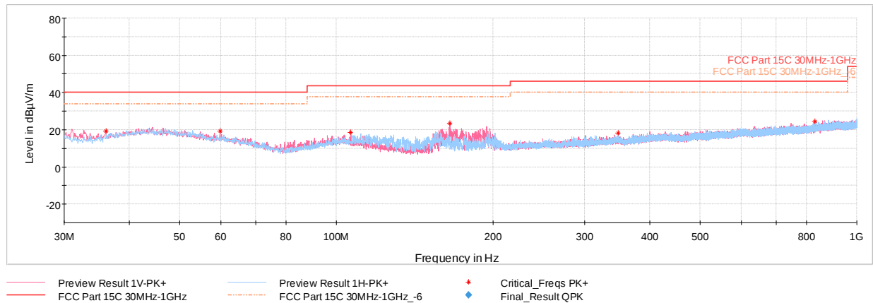
Plot 7-73. Radiated Spurious Emissions below 1GHz – Simultaneous Transmission
