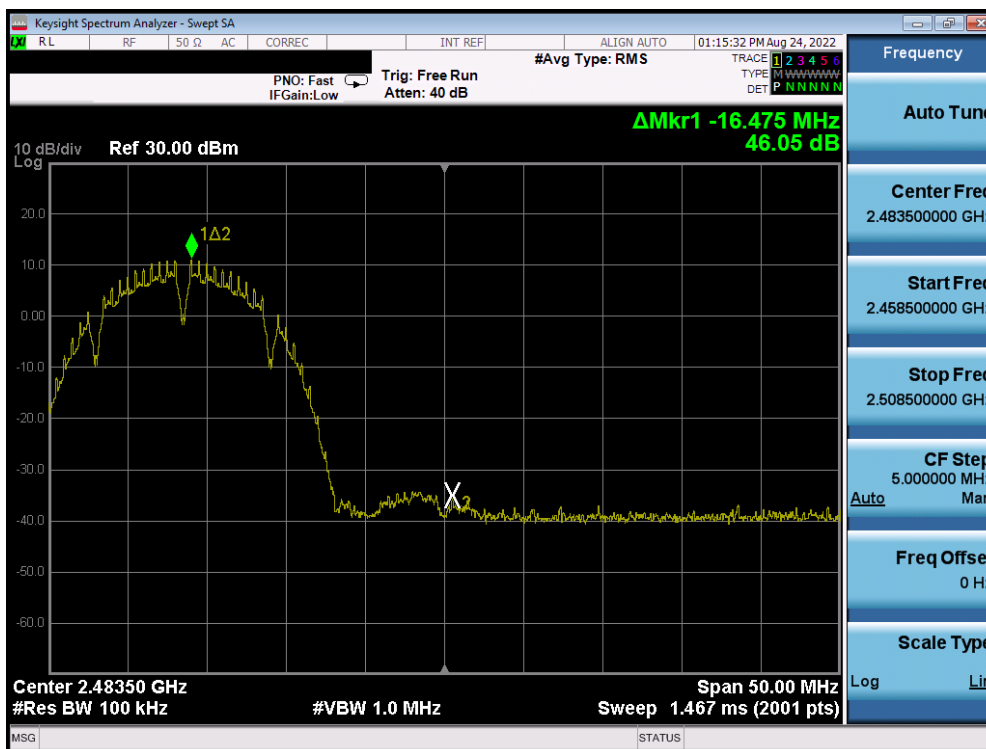
Plot 7-26. Band Edge Plot (802.11b– Ch. 12)
