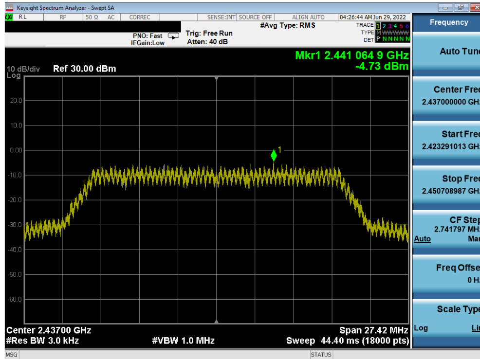
Plot 7-23. Power Spectral Density Plot (802.11n MCS7 – Ch. 6)
