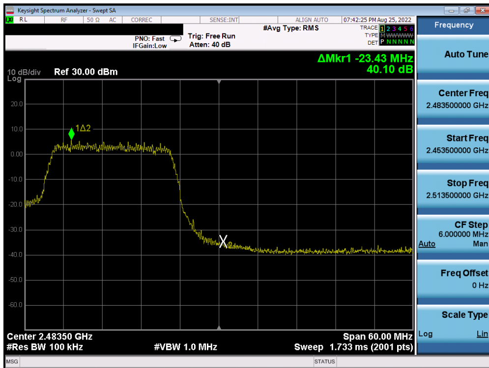
Plot 7-42. Band Edge Plot (802.11n MCS7 – Ch. 12)
