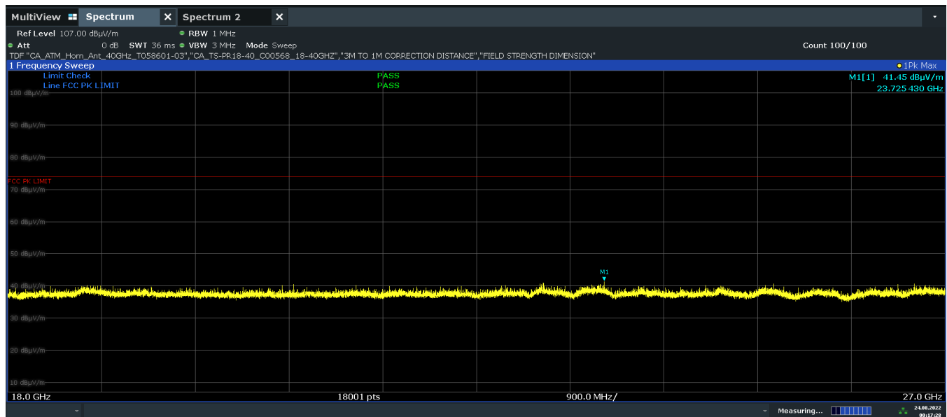
Plot 7-56. Radiated Spurious Emissions above 18GHz – Simultaneous Transmission (Pol. H)
