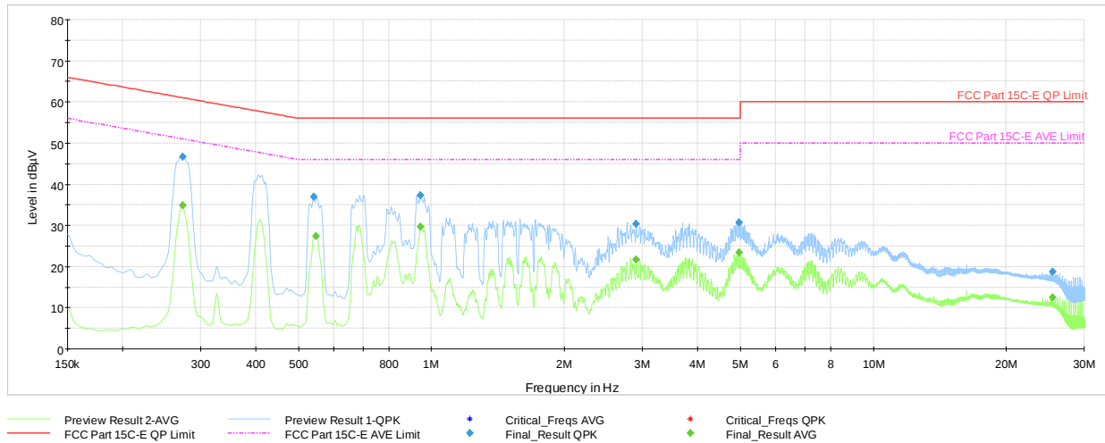
Plot 7-39. AC Line Conducted Plot with Bluetooth LE (L1, 1Mbps ePA – Ch.19 with AC/DC Adapter via USB cable with Magnetic Charger)
