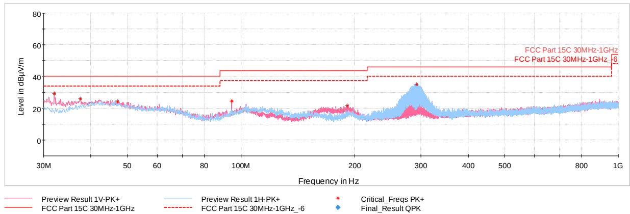
Plot 7-38. Radiated Spurious Emissions Below 1GHz (1Mbps, ePA – Ch. 19, Pol. H & V, with AC/DC adaptor via USB cable with Magnetic Charger)
