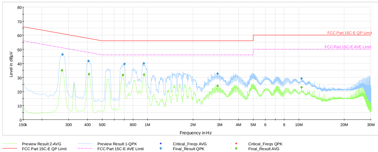
Plot 7-40. AC Line Conducted Plot with Bluetooth LE (N, 1Mbps ePA – Ch.19, with AC/DC Adapter via USB cable with Magnetic Charger)
