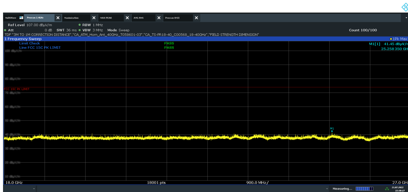
Plot 7-32. Radiated Spurious Emissions Above 18GHz (1Mbps ePA – Ch. 19, Pol. H)
