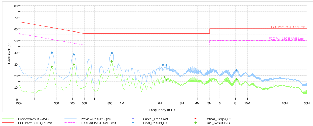
Plot 7-39. AC Line Conducted Plot with Bluetooth HDR (L1, 4Mbps ePA - Ch.38 with AC/DC Adapter + Laptop Charger)
