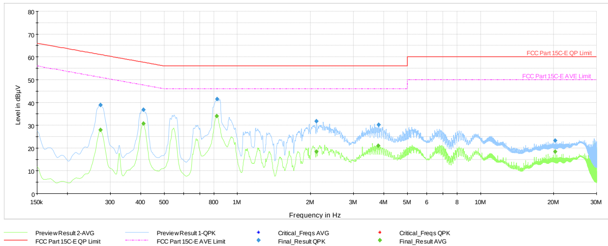
Plot 7-40. AC Line Conducted Plot with Bluetooth HDR (N, 4Mbps ePA - Ch.38 with AC/DC Adapter + Magnetic Charger)
