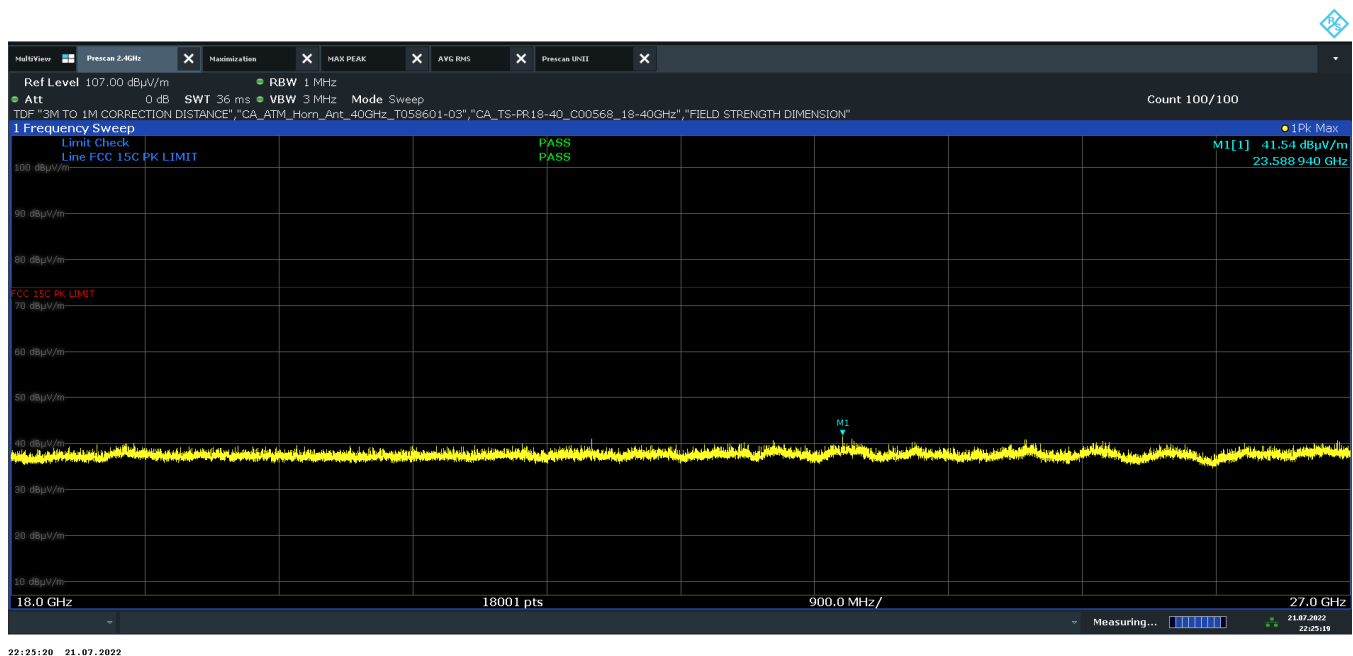
Plot 7-33. Radiated Spurious Emissions above 18GHz (BT GFSK – Ch.39, Pol. V)
