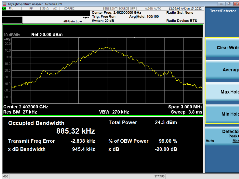
Plot 7-1. 20dB BW and 99% OBW Plot (Bluetooth, GFSK, ePA – Ch. 0)
