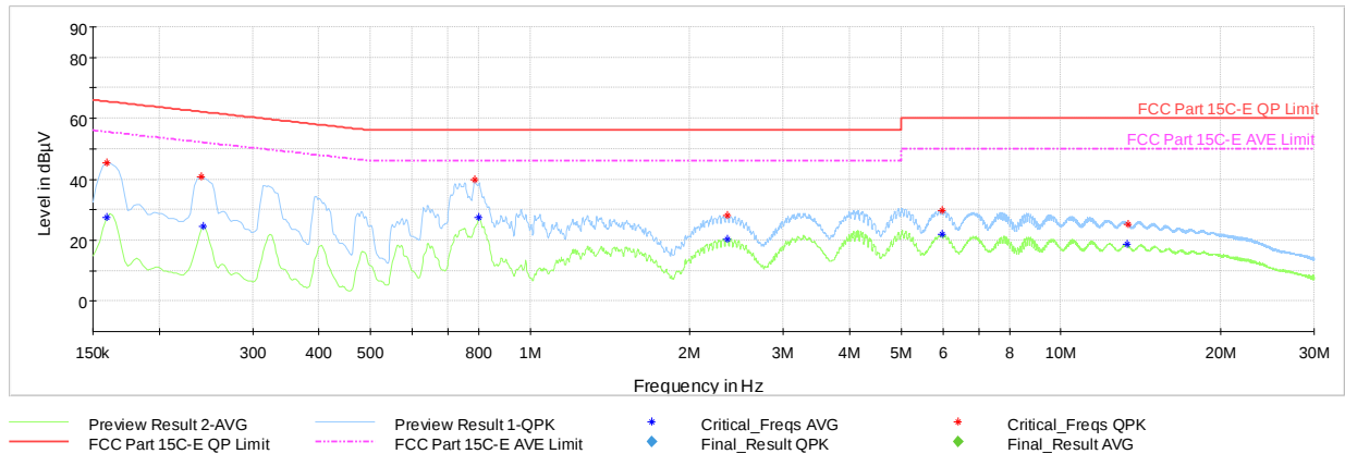
Plot 7-40. AC Line-Conducted Test Plot (N, GFSK ePA – Ch.39, with AC/DC Adapter via USB cable with Magnetic Charger)
