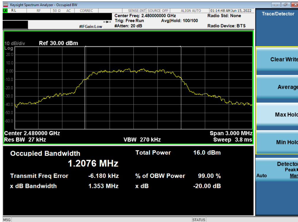
Plot 7-6. 20dB BW and 99% OBW Plot (Bluetooth, 8DPSK, ePA – Ch. 78)
