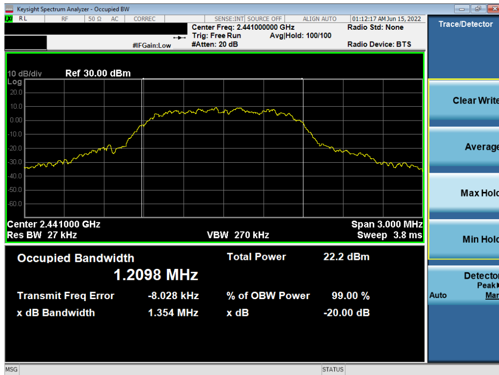
Plot 7-5. 20dB BW and 99% OBW Plot (Bluetooth, 8DPSK, ePA – Ch. 39)
