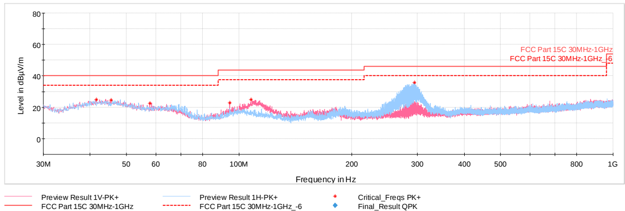
Plot 7-38. Radiated Spurious Emissions Below 1GHz (GFSK ePA – Ch.39, with Laptop via USB cable with Magnetic Charger)
