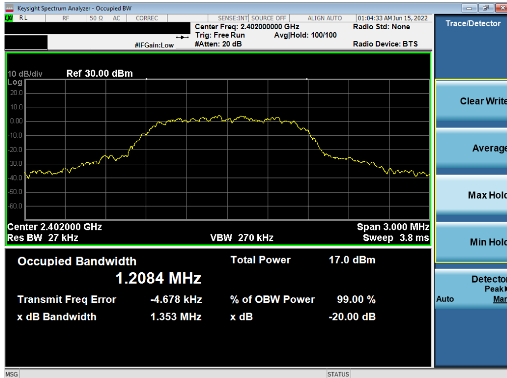
Plot 7-4. 20dB BW and 99% OBW Plot (Bluetooth, 8DPSK, ePA – Ch. 0)
