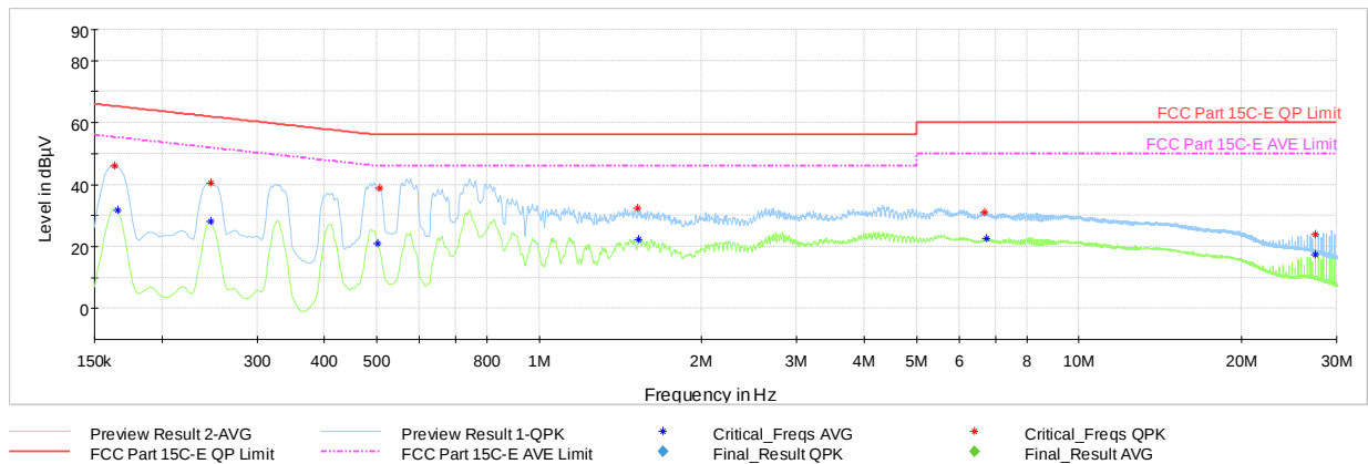
Plot 7-39. AC Line-Conducted Test Plot (L1, GFSK ePA – Ch.39, with AC/DC Adapter via USB cable with Magnetic Charger)
