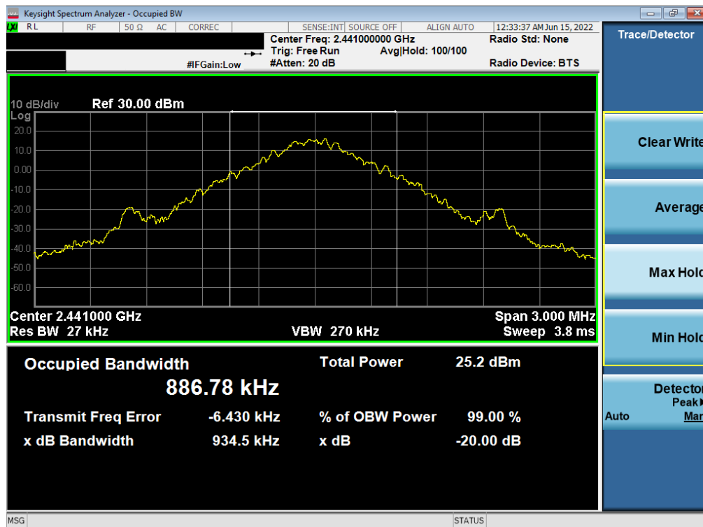
Plot 7-2. 20dB BW and 99% OBW Plot (Bluetooth, GFSK, ePA – Ch. 39)
