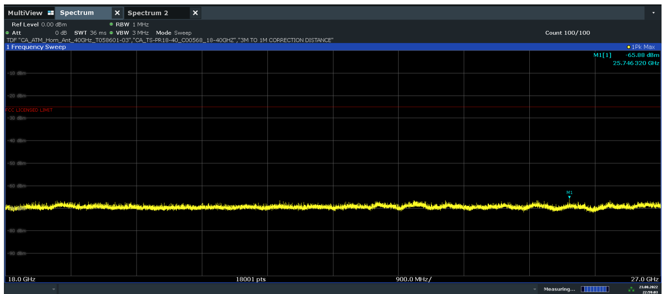
Plot 7-67. Antenna FCM Radiated Spurious Emissions -Simultaneous Transmission 18GHz - 27GHz Pol. H
