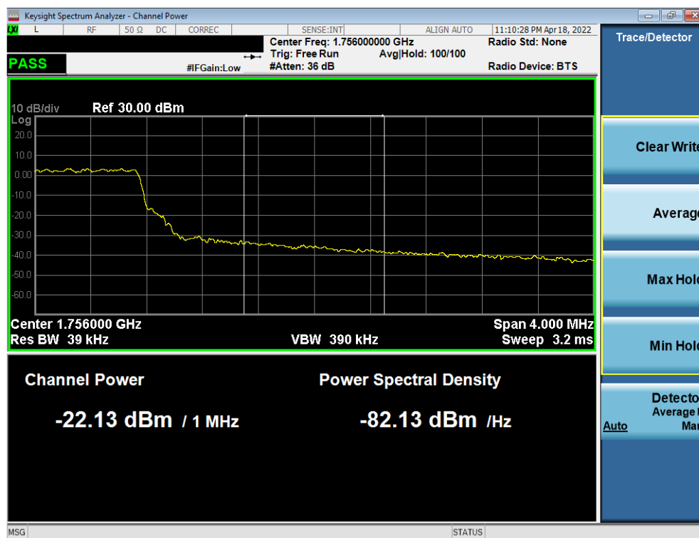
Plot 7-91. Upper Extended Band Edge Plot (LTE Band 4 - 5MHz QPSK – Full RB)
