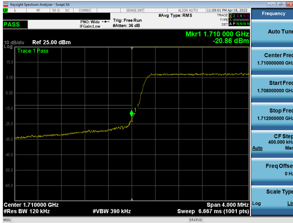
Plot 7-88. Lower Band Edge Plot (LTE Band 4 - 5MHz QPSK – Full RB)
