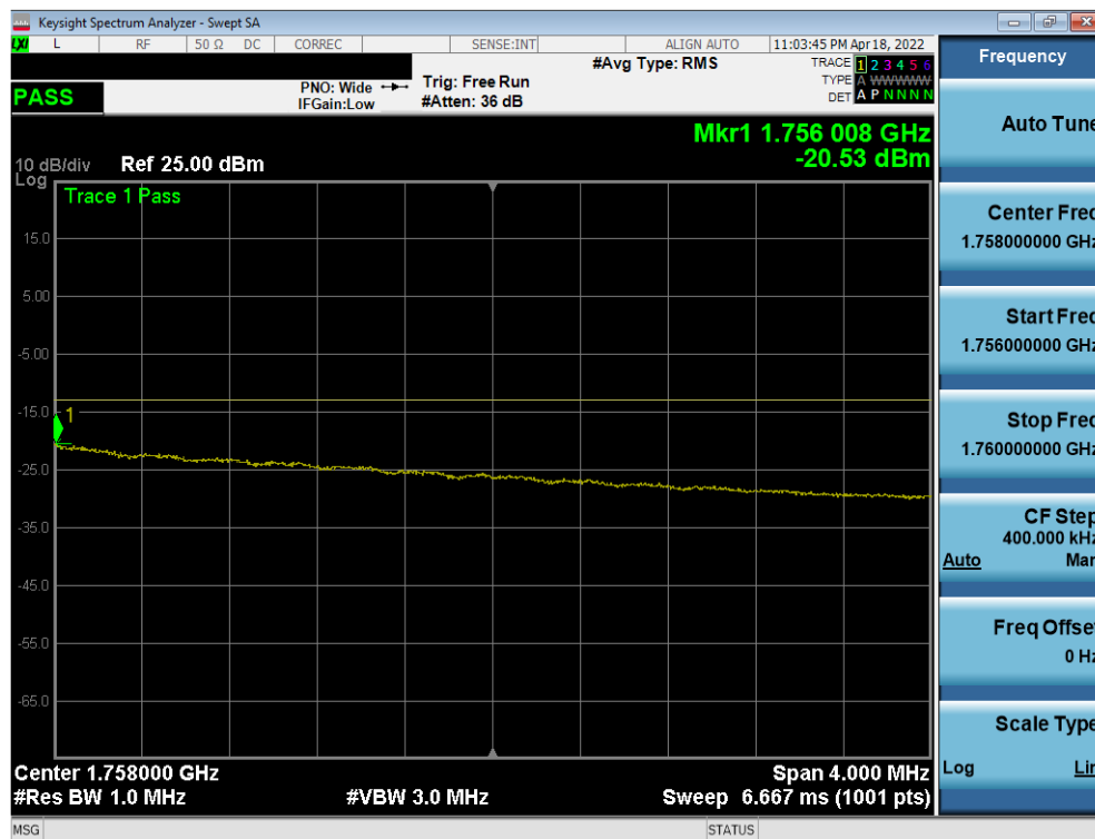
Plot 7-95. Upper Extended Band Edge Plot (LTE Band 4 - 10MHz QPSK – Full RB)
