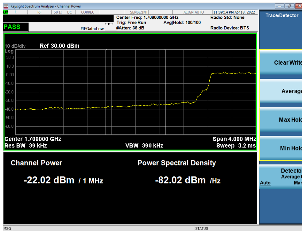
Plot 7-89. Lower Extended Band Edge Plot (LTE Band 4 - 5MHz QPSK – Full RB)
