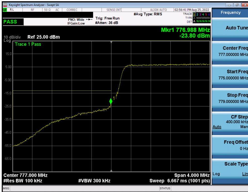
Plot 7-116. Lower Band Edge Plot (LTE Band 13 - 5MHz QPSK – Full RB)
