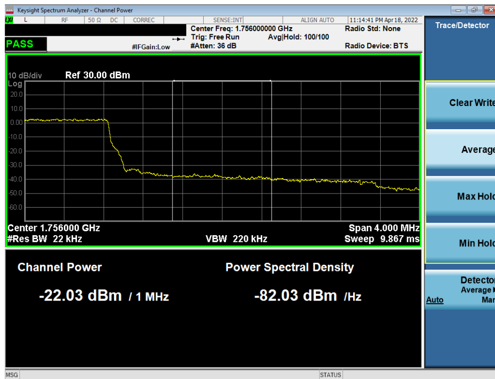
Plot 7-87. Upper Extended Band Edge Plot (LTE Band 4 - 3MHz QPSK – Full RB)
