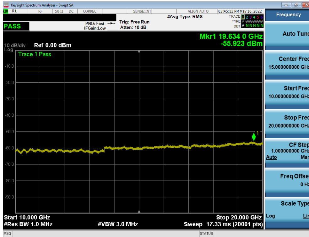
Plot 7-28. Conducted Spurious Plot (LTE Band 66/4 - 20MHz QPSK - RB Size 1, RB Offset 0 - Low Channel)
