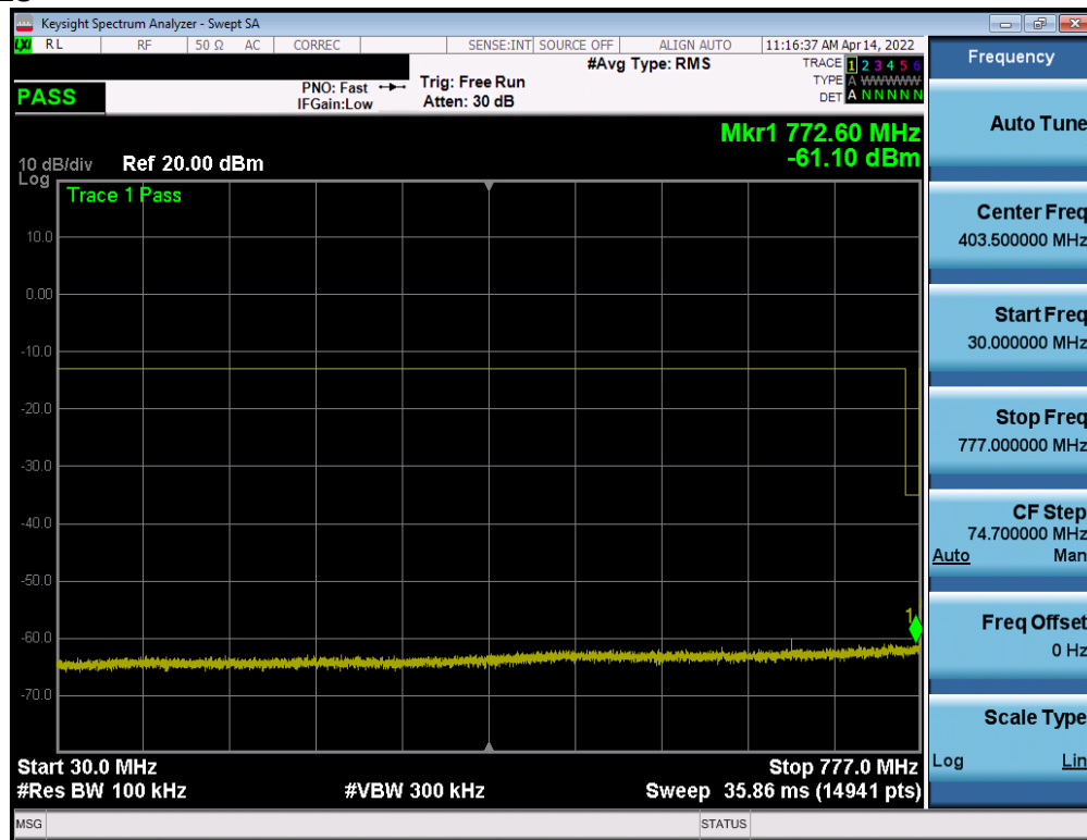
Plot 7-44. Conducted Spurious Plot (LTE Band 13 - 10MHz QPSK - RB Size 1, RB Offset 0)
