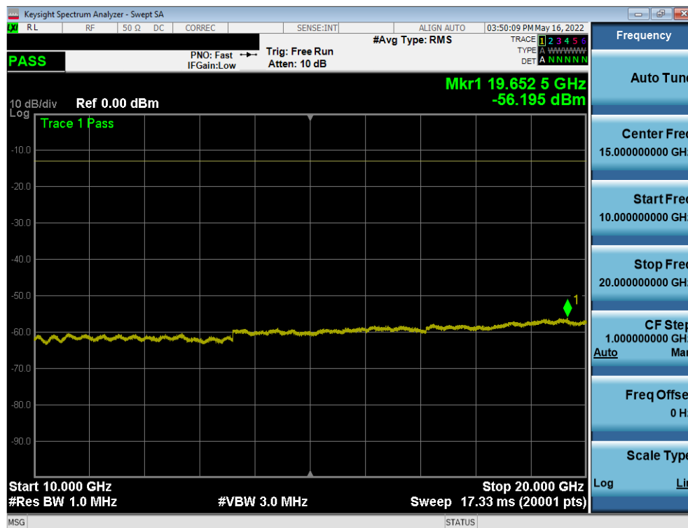
Plot 7-31. Conducted Spurious Plot (LTE Band 66/4 - 20MHz QPSK - RB Size 1, RB Offset 0 - Mid Channel)
