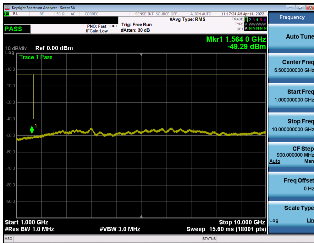
Plot 7-46. Conducted Spurious Plot (LTE Band 13 - 10MHz QPSK - RB Size 1, RB Offset 0)
