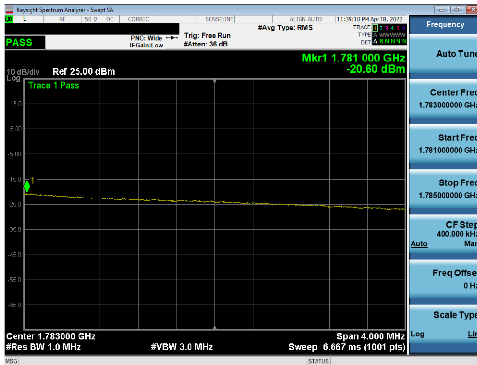
Plot 7-79. Upper Extended Band Edge Plot (LTE Band 66 - 20MHz QPSK – Full RB)
