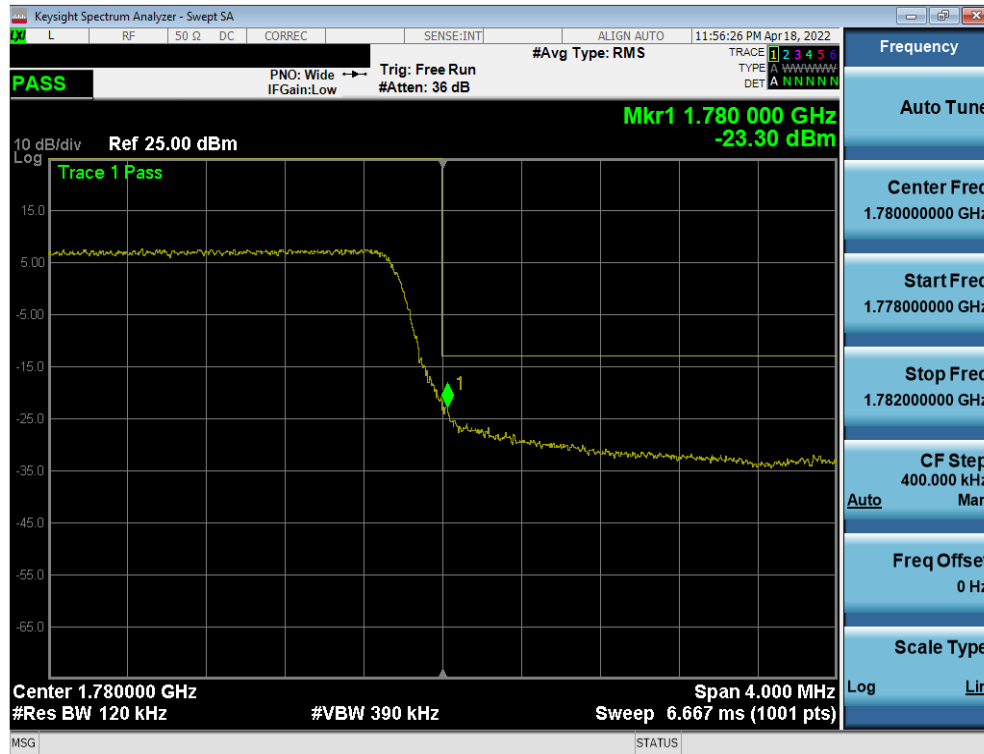
Plot 7-66. Upper Band Edge Plot (LTE Band 66 - 5MHz QPSK – Full RB)
