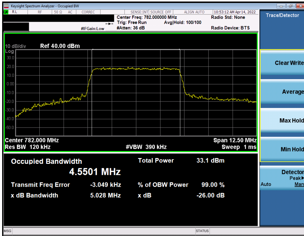
Plot 7-21. Occupied Bandwidth Plot (LTE Band 13 - 5MHz QPSK - Full RB)
