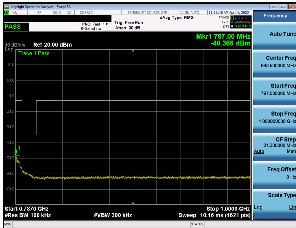
Plot 7-45. Conducted Spurious Plot (LTE Band 13 - 10MHz QPSK - RB Size 1, RB Offset 0)
