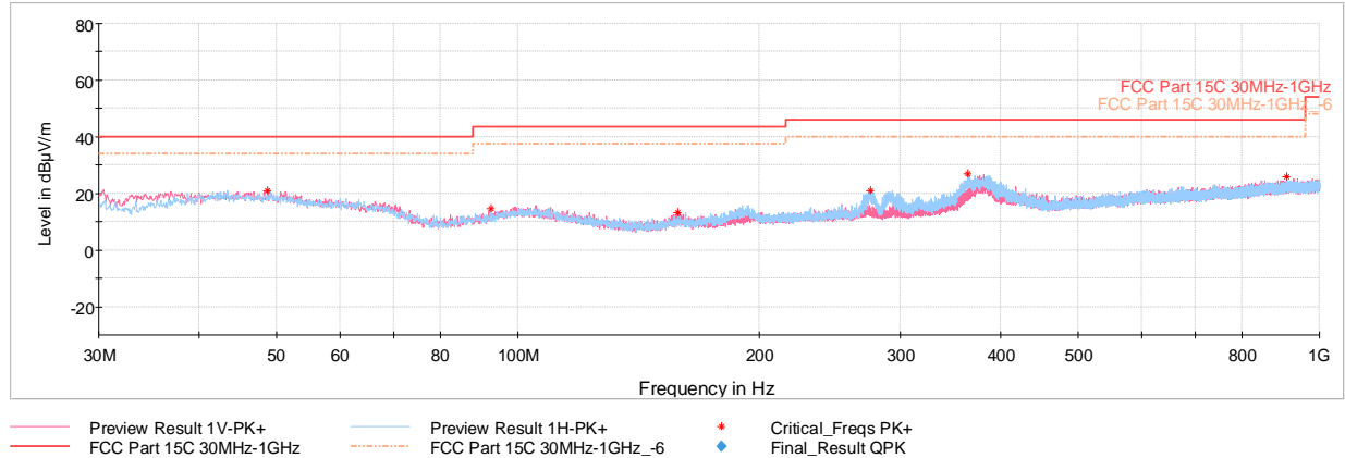
Plot 7-73. Radiated Spurious Emissions below 1GHz – Simultaneous Transmission
