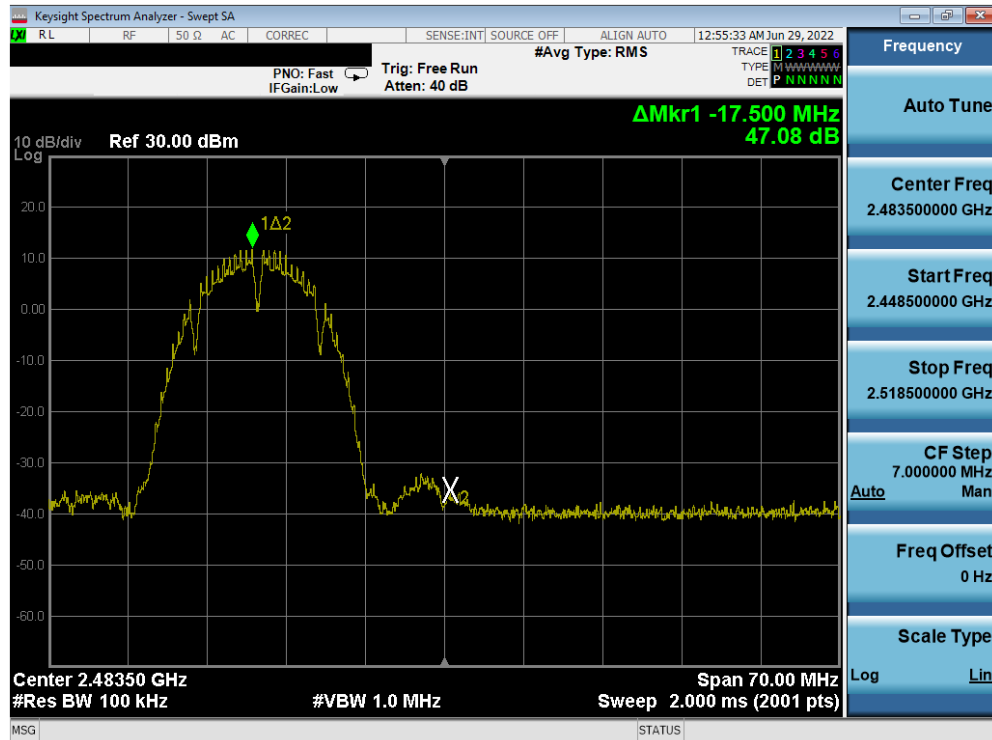
Plot 7-27. Band Edge Plot (802.11b – Ch. 12) – 6Mbps
