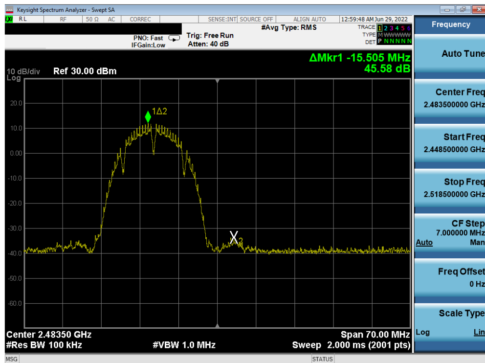
Plot 7-28. Band Edge Plot (802.11b – Ch. 13) – 6Mbps
